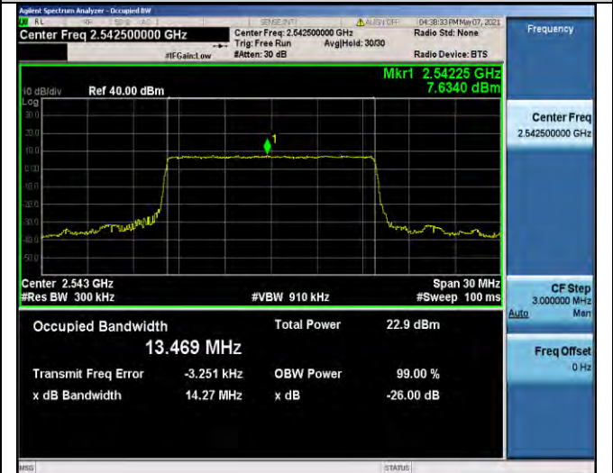
Band41-15MHz-QPSK-40115-75RB#0-13.469
