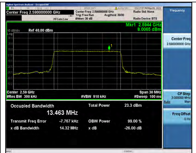
Band41-15MHz-16QAM-40590-75RB#0-13.463
