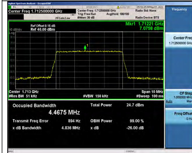
Band66-5MHz-16QAM-131997-25RB#0-4.4675
