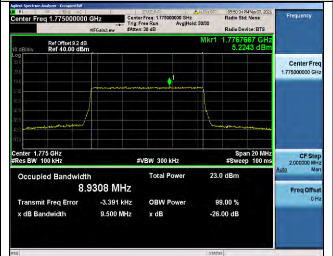
Band66-10MHz-16QAM-132622-50RB#0-8.9308
