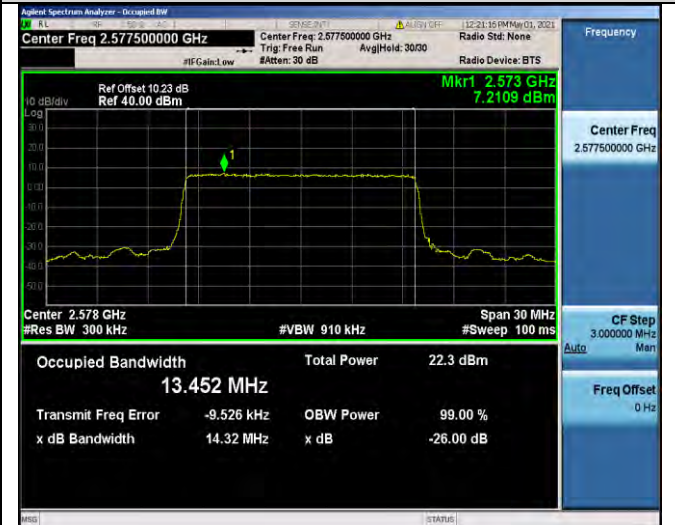
Band38-15MHz-QPSK-37825-75RB#0-13.452
