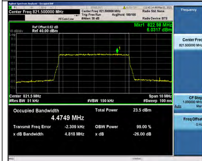
Band26-5MHz-16QAM-26765-25RB#0-4.4749
