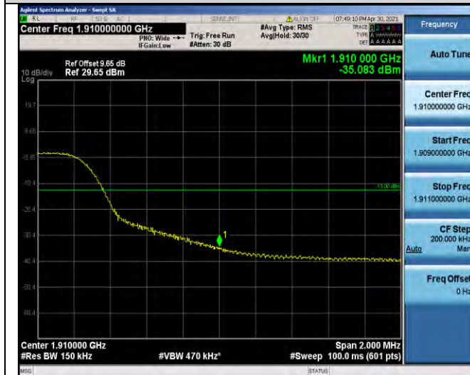
Band2-15MHz-16QAM-19125-75RB#0
