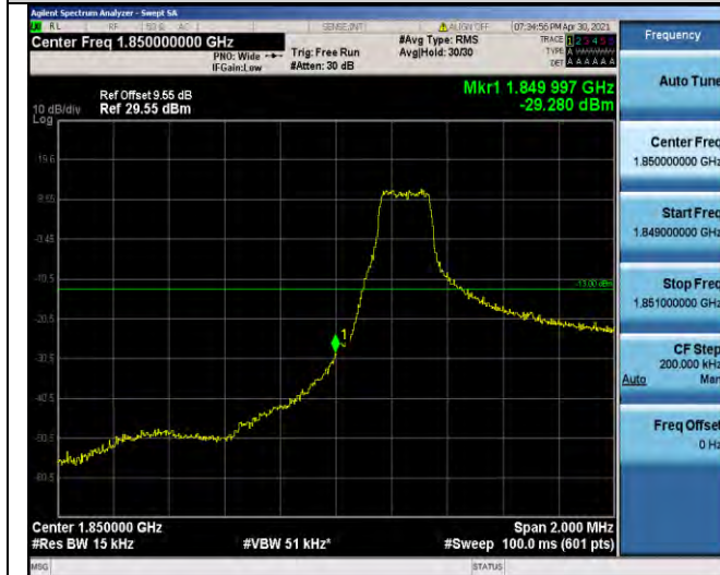
Band2-1.4MHz-16QAM-18607-1RB#0
