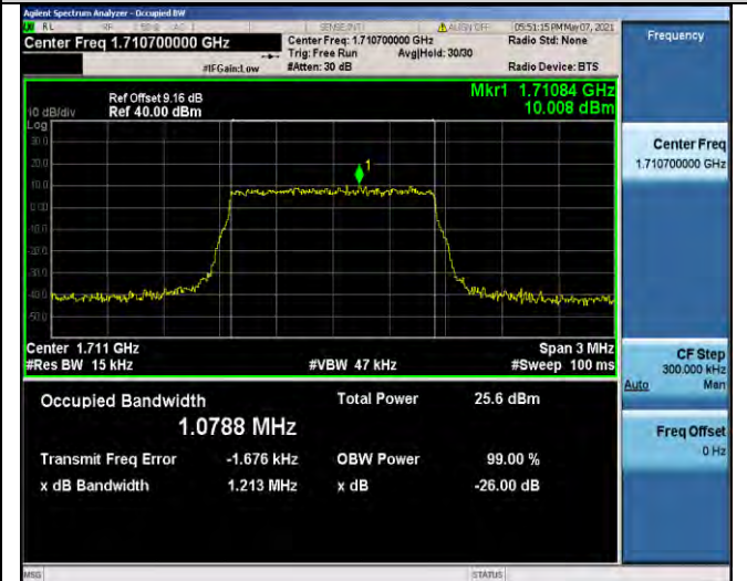
Band66-1.4MHz-QPSK-131979-6RB#0-1.0788
