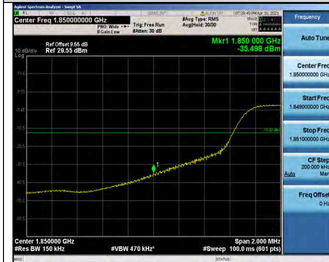
Band2-15MHz-QPSK-18675-75RB#0
