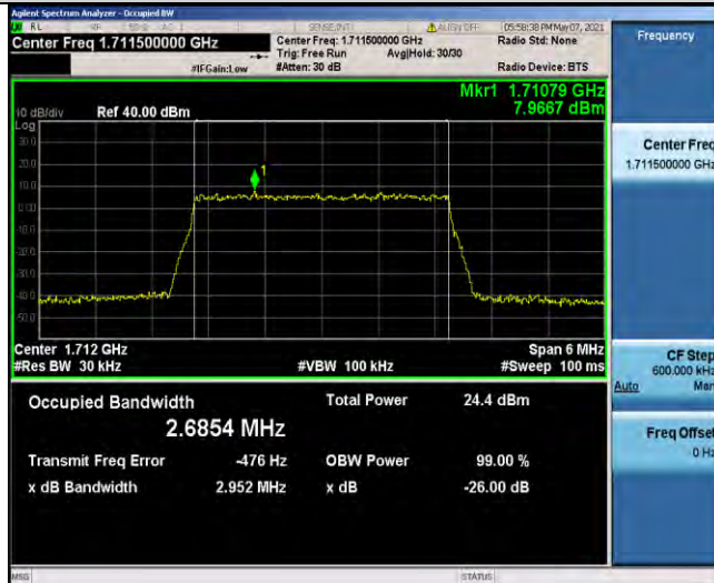
Band66-3MHz-16QAM-131987-15RB#0-2.6854
