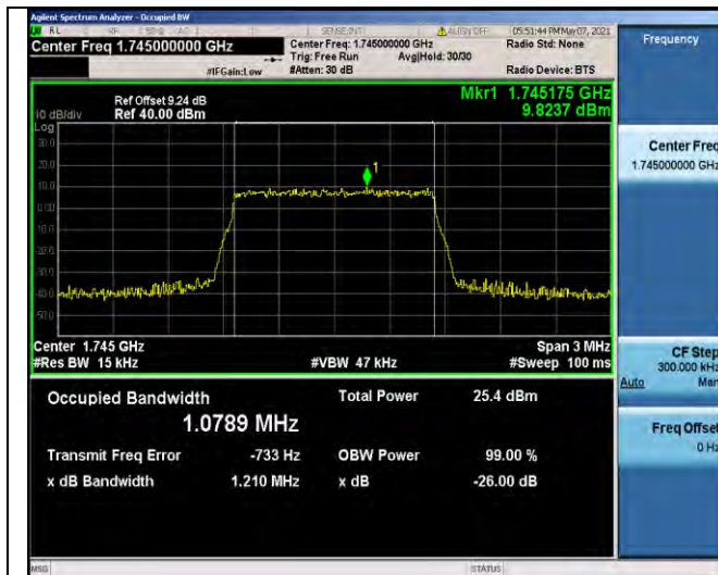
Band66-1.4MHz-QPSK-132322-6RB#0-1.0789
