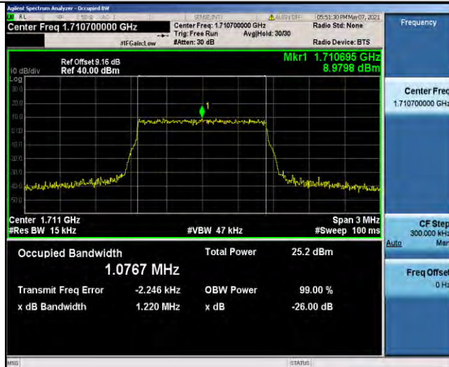
Band66-1.4MHz-16QAM-131979-6RB#0-1.0767
