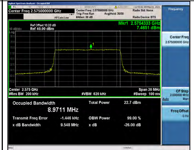
Band38-10MHz-QPSK-37800-50RB#0-8.9711
