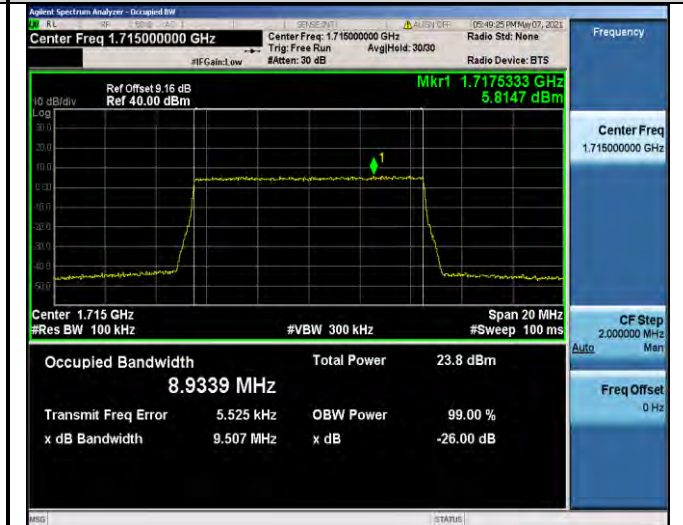
Band66-10MHz-QPSK-132022-50RB#0-8.9339
