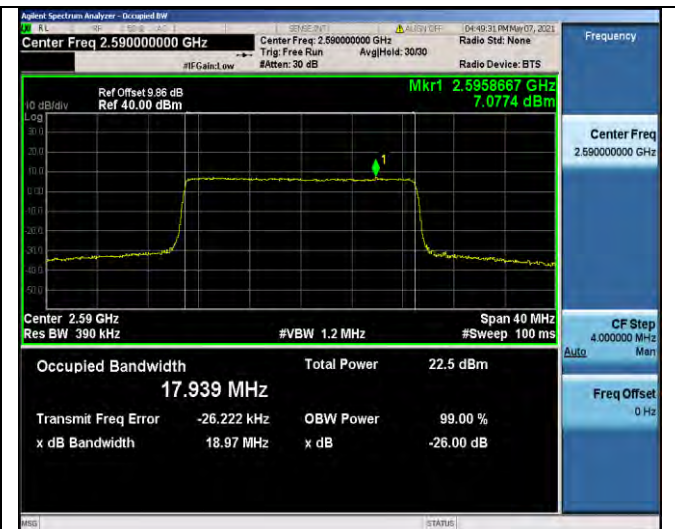
Band41-20MHz-16QAM-40590-100RB#0-17.939
