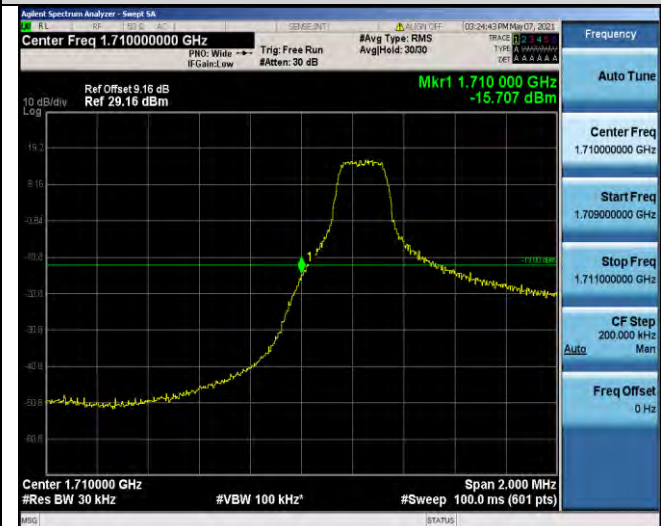
Band4-3MHz-16QAM-19965-1RB#0
