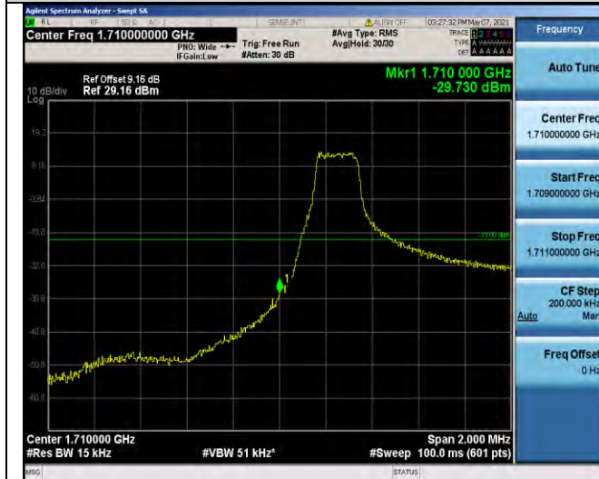
Band4-1.4MHz-16QAM-19957-1RB#0
