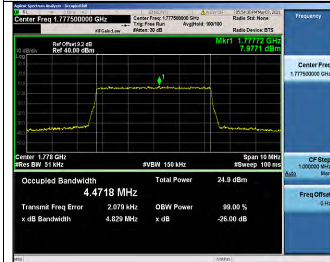
Band66-5MHz-QPSK-132647-25RB#0-4.4718
