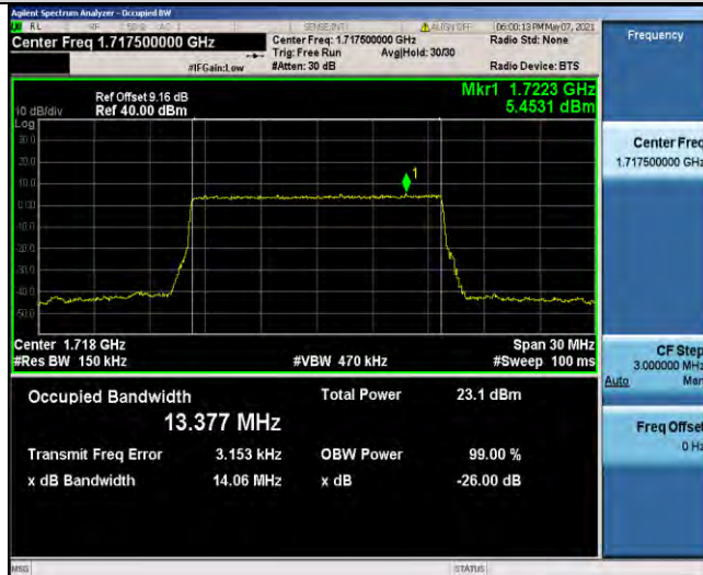
Band66-15MHz-16QAM-132047-75RB#0-13.377
