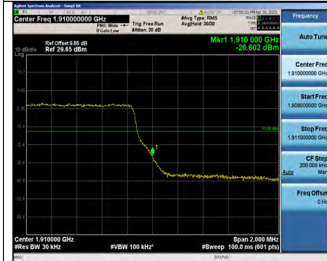
Band2-3MHz-16QAM-19185-15RB#0
