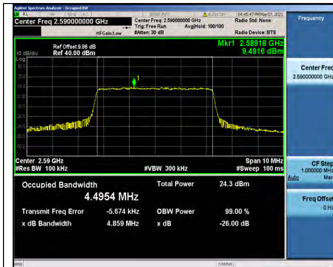
Band41-5MHz-QPSK-40590-25RB#0-4.4954
