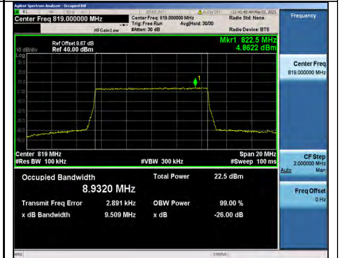
Band26-10MHz-16QAM-26740-50RB#0-8.9320
