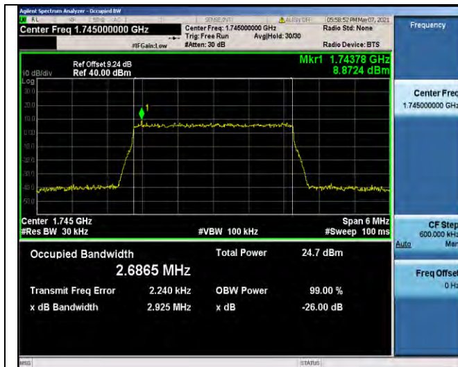
Band66-3MHz-QPSK-132322-15RB#0-2.6865
