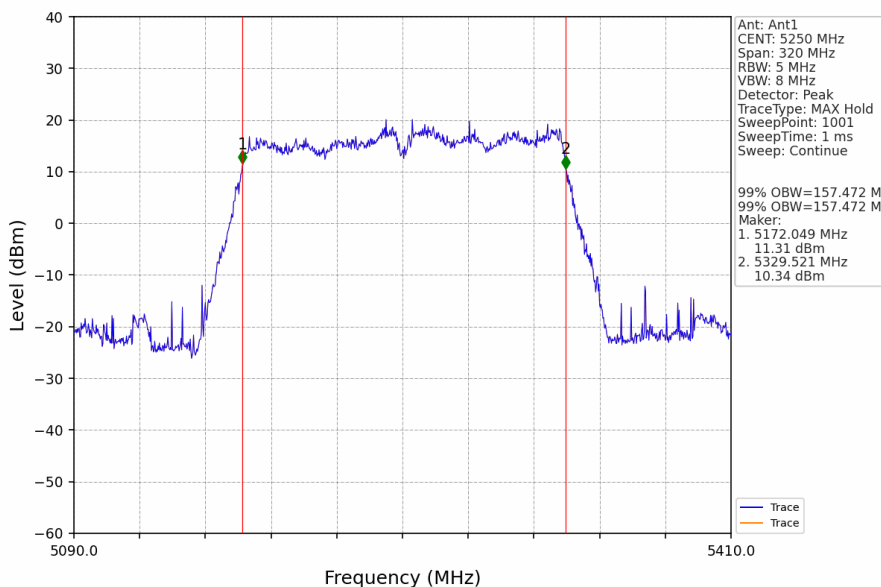
802.11ac(VHT160)_MCH_5250MHz_Ant1_NTNV
