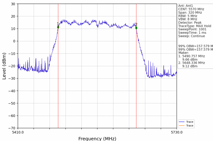
802.11ac(VHT160)_MCH_5570MHz_Ant1_NTNV
