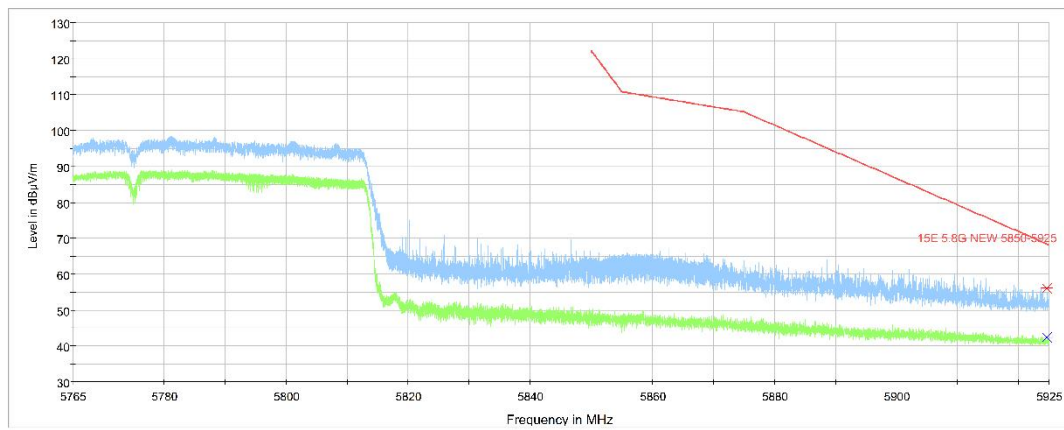
Fig. 12 Band Edges (802.11ac-HT80, 5775MHz)
