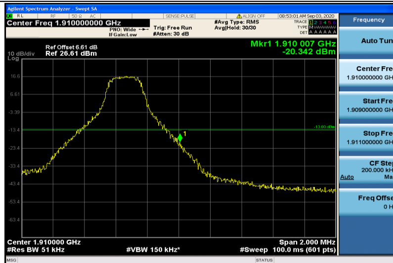
Band2-5MHz-16QAM-19175-1RB#24
