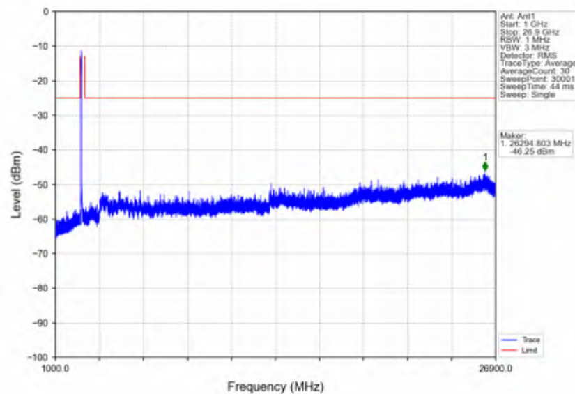
n41_15kHz_SISO_NTNV_40MHz_CP-OFDM QPSK_2516.01MHz_Outer_Full
