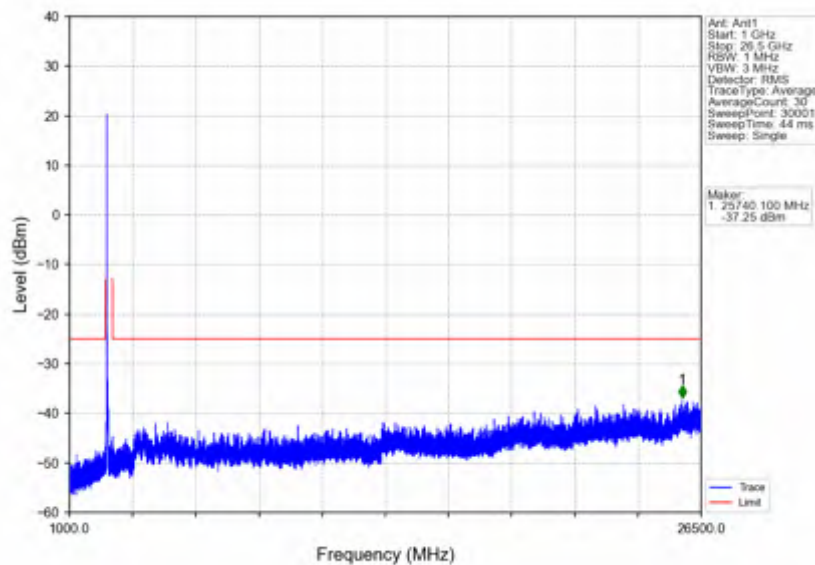
n41_15kHz_SISO_NTNV_40MHz_CP-OFDM QPSK_2516.01MHz_Outer_Full
