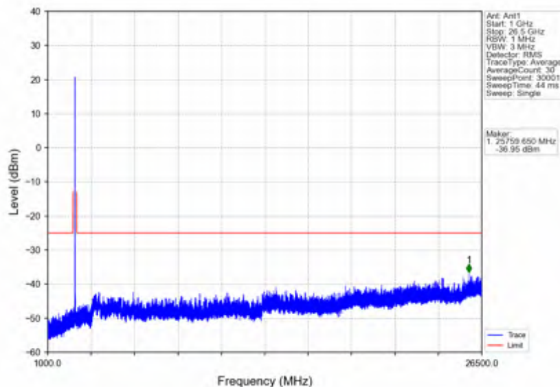
n41_30kHz_SISO_NTNV_15MHz_DFT-s-OFDM QPSK_2682.48MHz_Edge_1RB_Right
