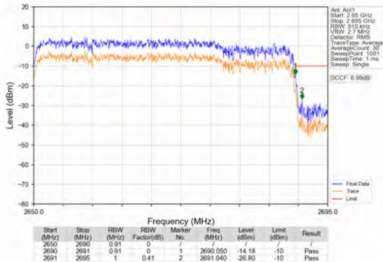
n41_15kHz_SISO_NTNV_40MHz_CP-OFDM QPSK_2670MHz_Outer_Full
