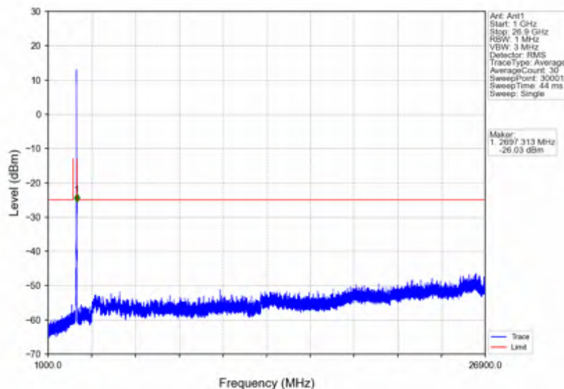
n41_30kHz_SISO_NTNV_15MHz_DFT-s-OFDM QPSK_2682.48MHz_Inner_1RB_Right
