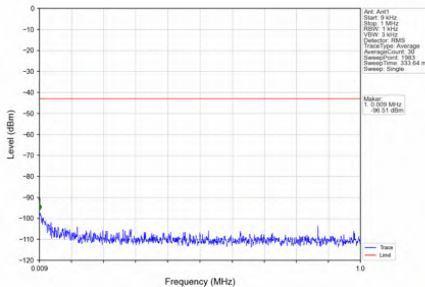
n41_30kHz_SISO_NTNV_10MHz_DFT-s-OFDM QPSK_2501.01MHz_Outer_Full
