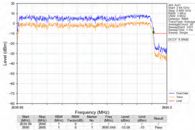
n41_15kHz_SISO_NTNV_50MHz_CP-OFDM QPSK_2664.99MHz_Outer_Full
