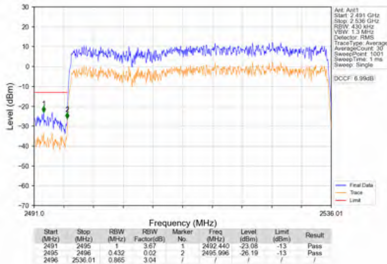
n41_15kHz_SISO_NTNV_40MHz_CP-OFDM QPSK_2516.01MHz_Outer_Full
