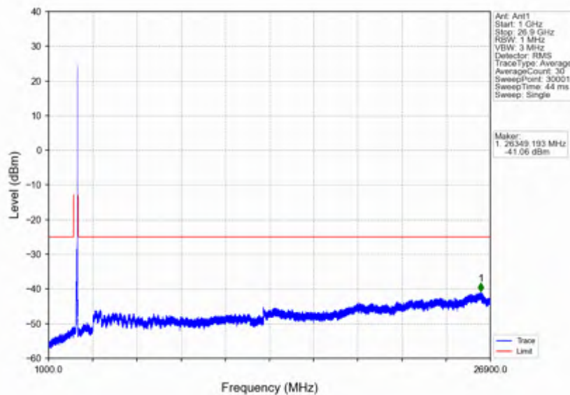
n41_15kHz_SISO_NTNV_40MHz_CP-OFDM QPSK_2670MHz_Outer_Full
