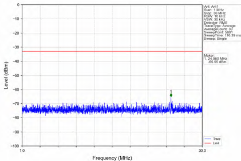
n41_30kHz_SISO_NTNV_15MHz_DFT-s-OFDM QPSK_2592.99MHz_Edge_1RB_Left
