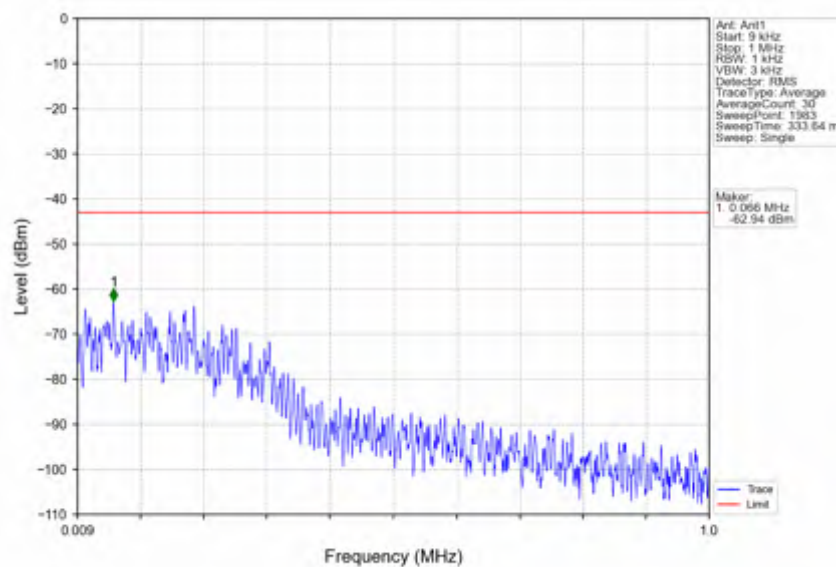
n41_30kHz_SISO_NTNV_10MHz_CP-OFDM_QPSK_2501.01MHz_Edge_1RB_Left
