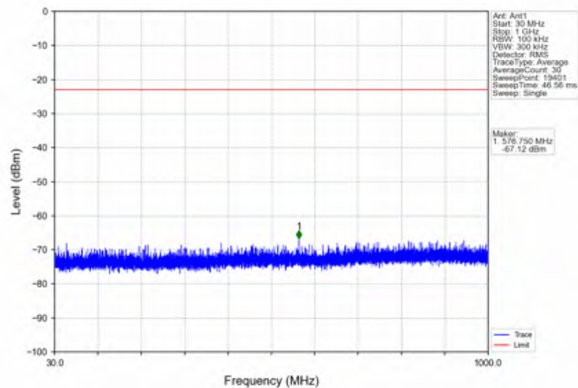
n41_30kHz_SISO_NTNV_15MHz_DFT-s-OFDM QPSK_2682.48MHz_Outer_Full
