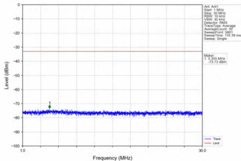
n41_15kHz_SISO_NTNV_40MHz_CP-OFDM QPSK_2670MHz_Edge_1RB_Right
