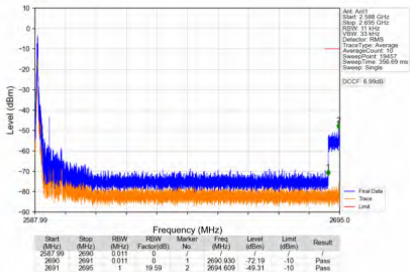
n41_30kHz_SISO_NTNV_10MHz_CP-OFDM QPSK_2592.99MHz_Edge_1RB_Left
