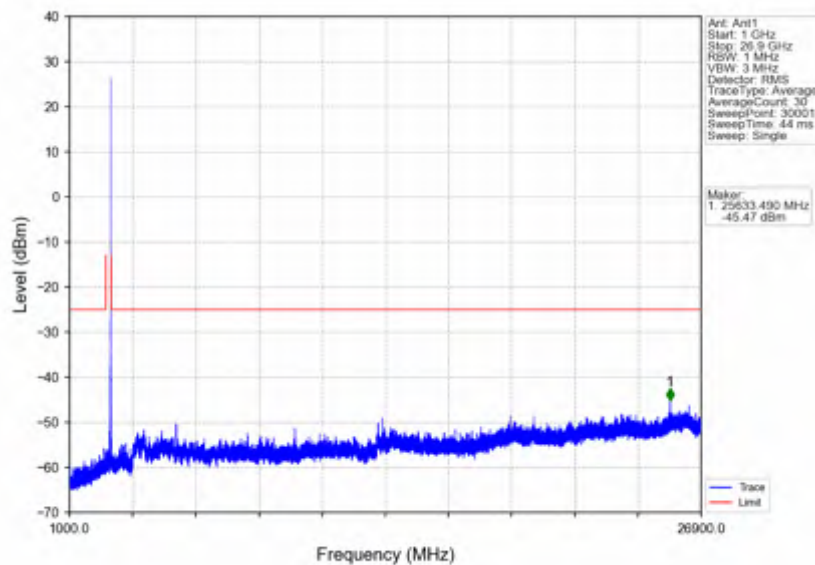
n41_30kHz_SISO_NTNV_10MHz_DFT-s-OFDM_QPSK_2501.01MHz_Edge_1RB_Left
