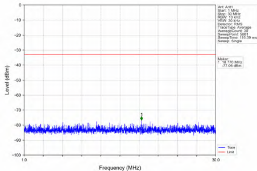
n41_30kHz_SISO_NTNV_10MHz_DFT-s-OFDM QPSK_2685MHz_Outer_Full
