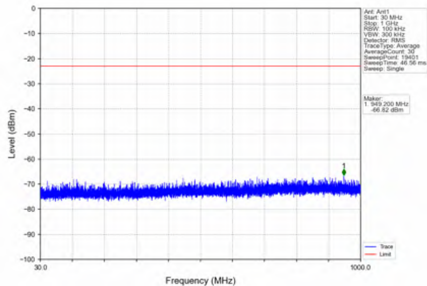
n41_30kHz_SISO_NTNV_10MHz_CP-OFDM QPSK_2685MHz_Outer_Full
