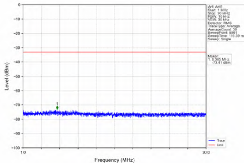
n41_15kHz_SISO_NTNV_50MHz_DFT-s-OFDM QPSK_2664.99MHz_Outer_Full
