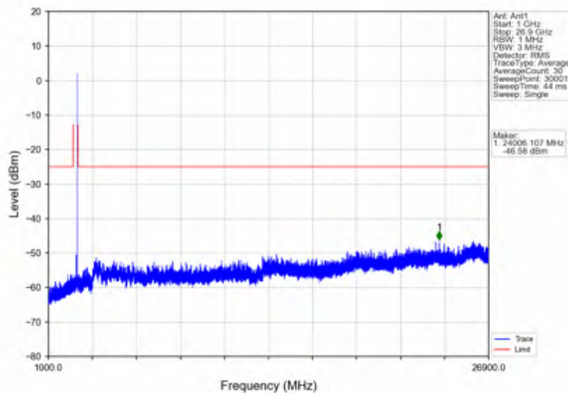
n41_15kHz_SISO_NTNV_50MHz_CP-OFDM QPSK_2664.99MHz_Outer_Full
