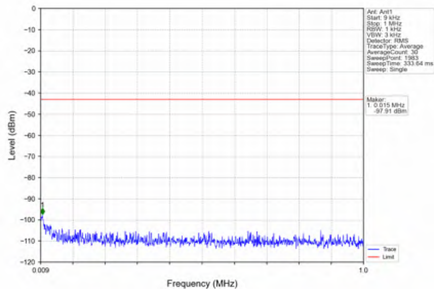
n41_30kHz_SISO_NTNV_15MHz_CP-OFDM QPSK_2503.5MHz_Outer_Full
