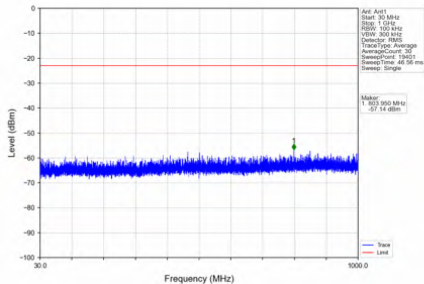
n41_30kHz_SISO_NTNV_15MHz_DFT-s-OFDM_QPSK_2503.5MHz_Edge_1RB_Left
