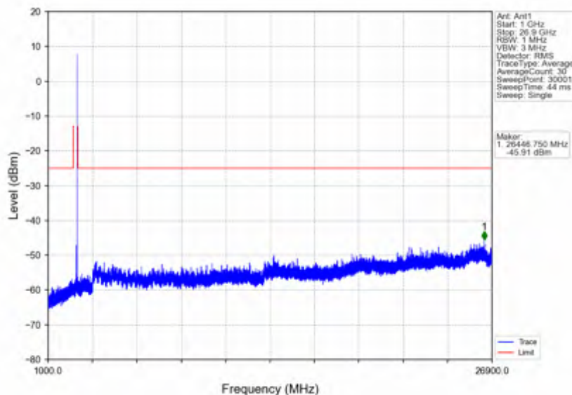
n41_15kHz_SISO_NTNV_40MHz_DFT-s-OFDM QPSK_2516.01MHz_Edge_1RB_Left
