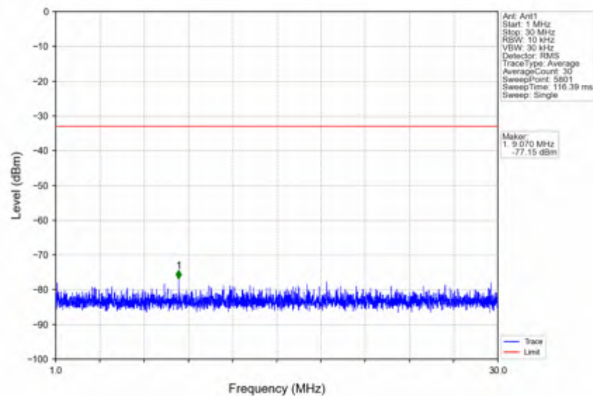
n41_30kHz_SISO_NTNV_15MHz_DFT-s-OFDM QPSK_2682.48MHz_Outer_Full
