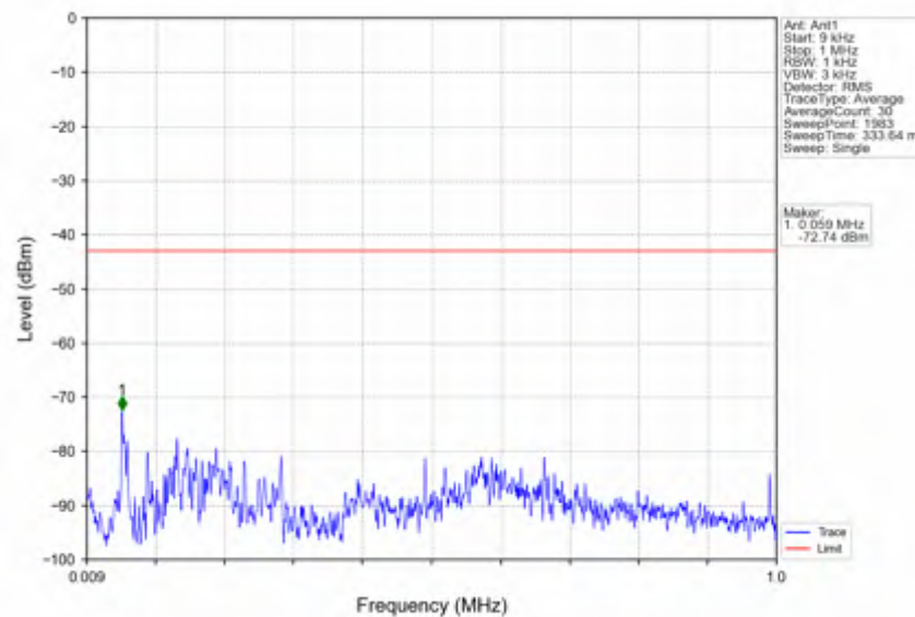
n41_15kHz_SISO_NTNV_50MHz_DFT-s-OFDM_QPSK_2664.99MHz_Outer_Full
