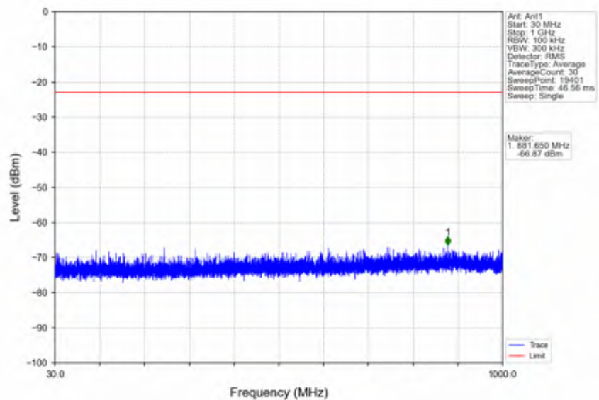
n41_15kHz_SISO_NTNV_50MHz_CP-OFDM QPSK_2664.99MHz_Inner_1RB_Right
