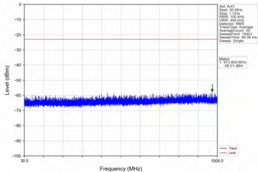
n41_30kHz_SISO_NTNV_10MHz_CP-OFDM QPSK_2501.01MHz_Edge_1RB_Left
