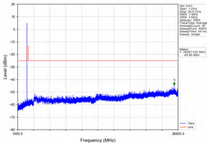
n41_30kHz_SISO_NTNV_15MHz_DFT-s-OFDM_PI/2_BPSK_2592.99MHz_Edge_1RB_Left
