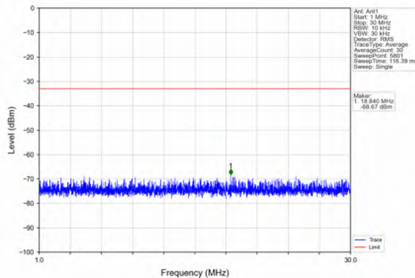
n41_15kHz_SISO_NTNV_50MHz_CP-OFDM QPSK_2664.99MHz_Edge_1RB_Right
