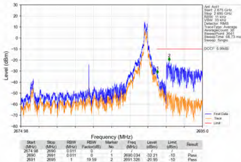
n41_30kHz_SISO_NTNV_15MHz_DFT-s-OFDM QPSK_2682.48MHz_Inner_1RB_Right
