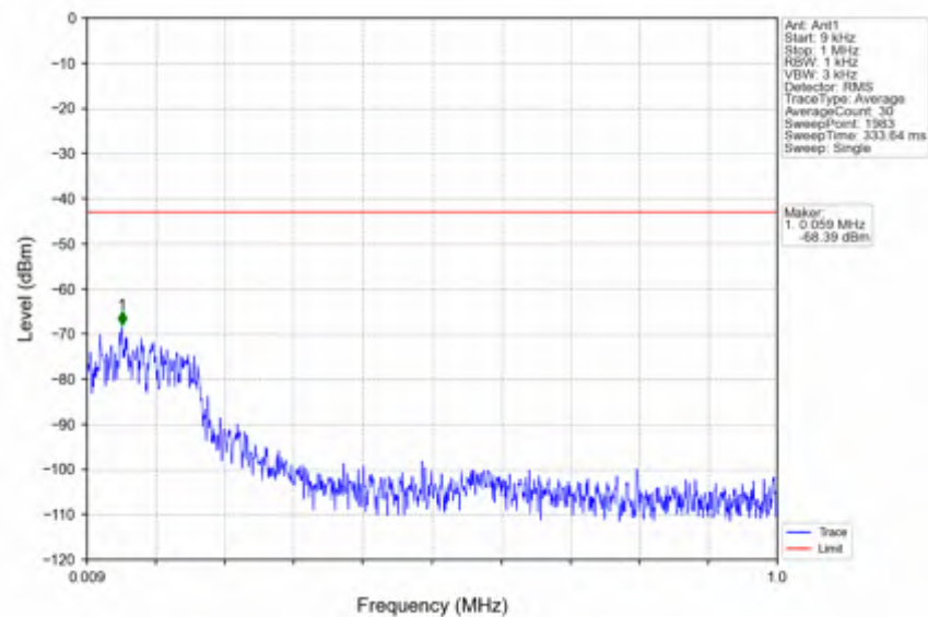
n41_15kHz_SISO_NTNV_40MHz_DFT-s-OFDM QPSK_2670MHz_Edge_1RB_Right
