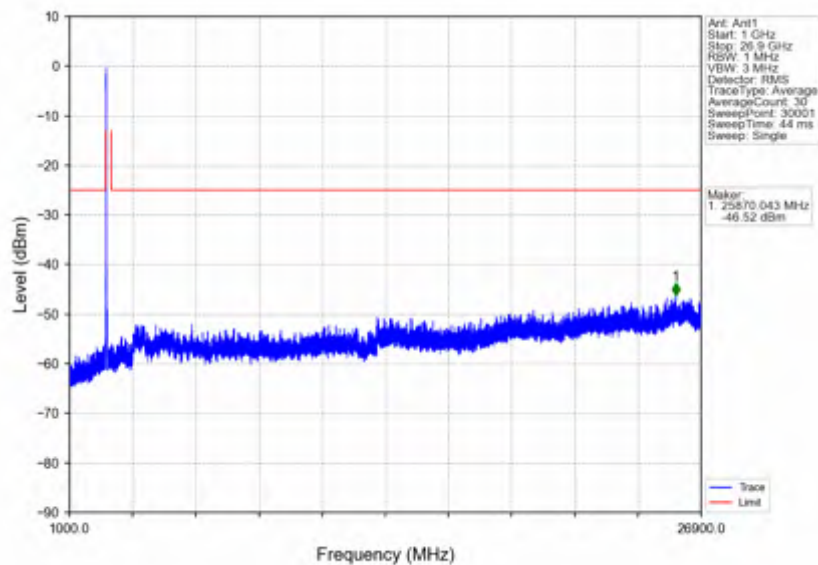
n41_30kHz_SISO_NTNV_15MHz_DFT-s-OFDM_QPSK_2503.5MHz_Inner_1RB_Left
