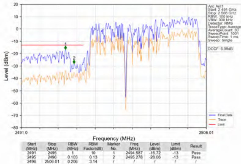
n41_30kHz_SISO_NTNV_10MHz_CP-OFDM QPSK_2501.01MHz_Outer_Full
