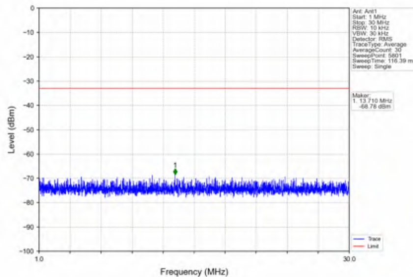
n41_30kHz_SISO_NTNV_10MHz_DFT-s-OFDM QPSK_2685MHz_Edge_1RB_Right
