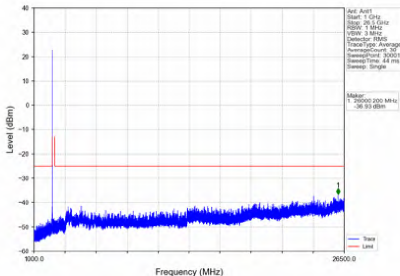
n41_30kHz_SISO_NTV_15MHz_CP-OFDM QPSK_2503.5MHz_Outer_Full
