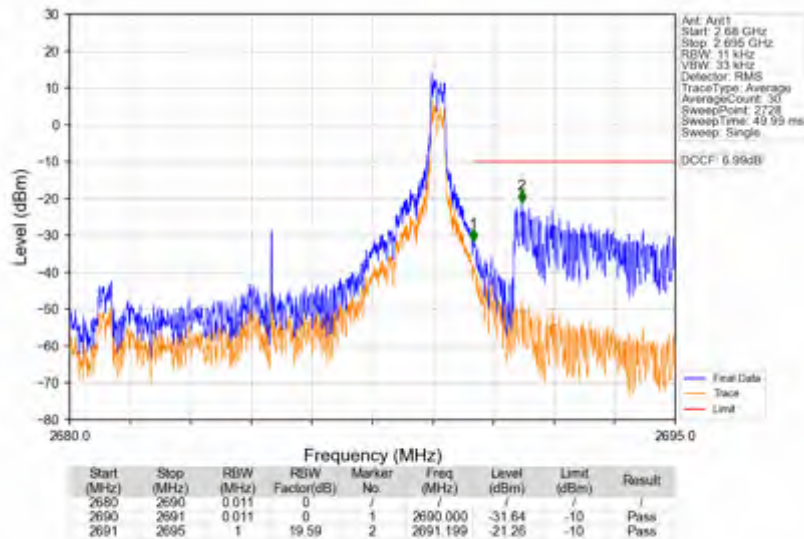
n41_30kHz_SISO_NTNV_10MHz_DFT-s-OFDM QPSK_2685MHz_Edge_1RB_Right
