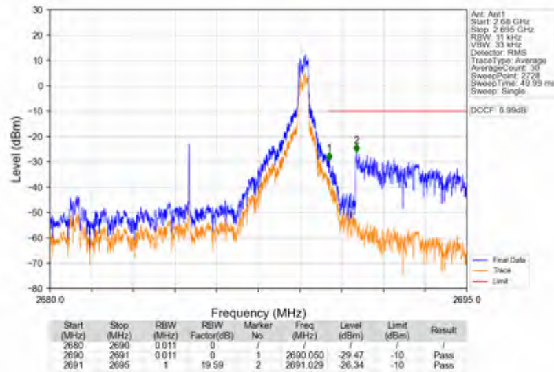
n41_30kHz_SISO_NTNV_10MHz_CP-OFDM_QPSK_2685MHz_Edge_1RB_Right
