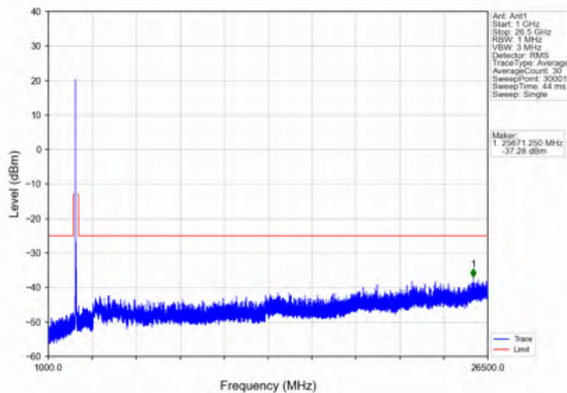
n41_15kHz_SISO_NTNV_50MHz_DFT-s-OFDM QPSK_2664.99MHz_Edge_1RB_Right
