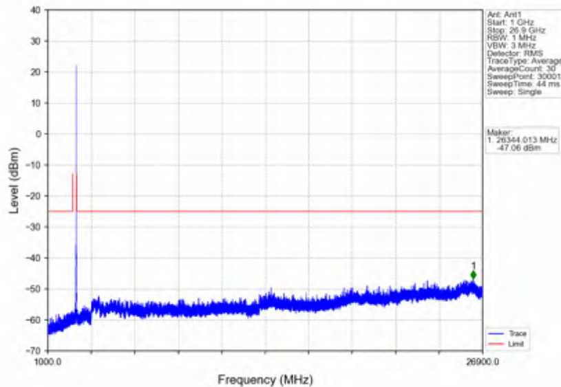
n41_30kHz_SISO_NTV_15MHz_DFT-s-OFDM_QPSK_2682.48MHz_Edge_1RB_Right
