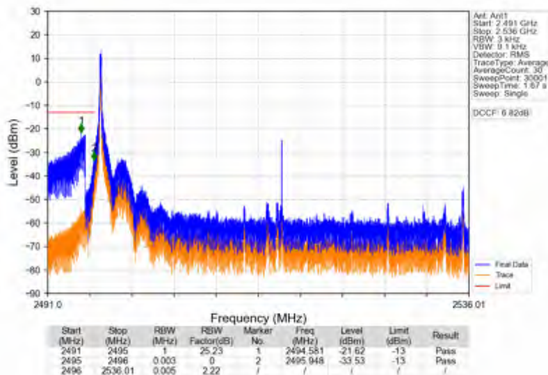
n41_15kHz_SISO_NTNV_40MHz_DFT-s-OFDM QPSK_2516.01MHz_Edge_1RB_Left
