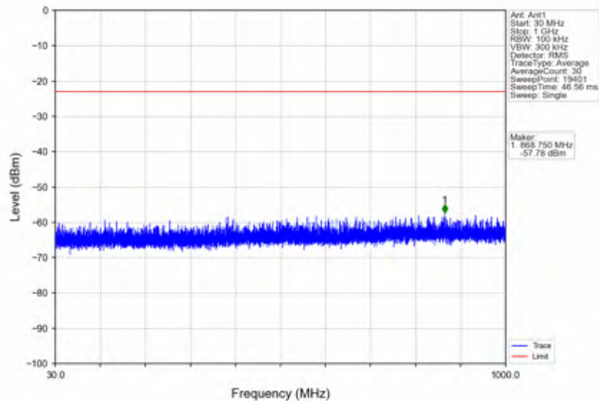
n41_30kHz_SISO_NTV_15MHz_DFT-s-OFDM_QPSK_2682.48MHz_Edge_1RB_Right
