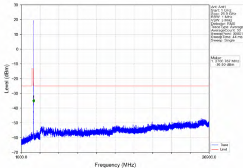
n41_30kHz_SISO_NTNV_10MHz_DFT-s-OFDM_PI/2_BPSK_2685MHz_Outer_Full
