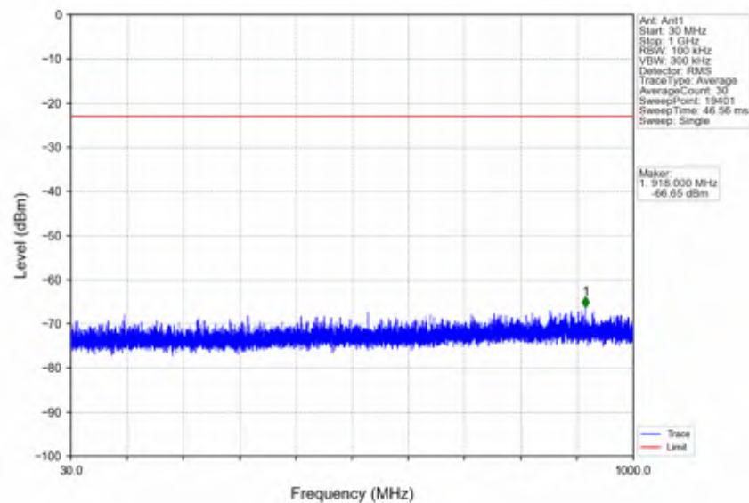
n41_30kHz_SISO_NTNV_10MHz_DFT-s-OFDM QPSK_2501.01MHz_Outer_Full
