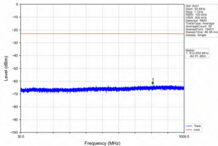
n41_15kHz_SISO_NTNV_50MHz_CP-OFDM QPSK_2664.99MHz_Outer_Full
