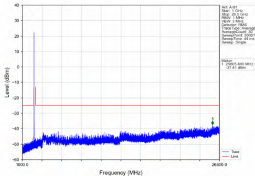
n41_30kHz_SISO_NTNV_15MHz_DFT-s-OFDM_QPSK_2503.5MHz_Edge_1RB_Left
