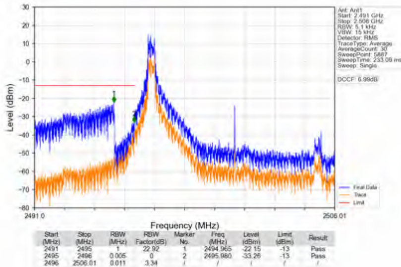
n41_30kHz_SISO_NTNV_10MHz_DFT-s-OFDM_QPSK_2501.01MHz_Edge_1RB_Left
