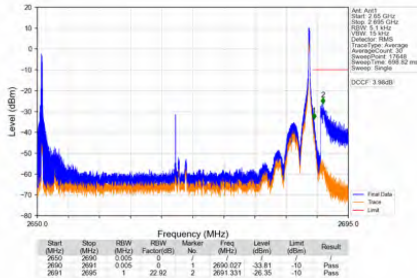
n41_15kHz_SISO_NTNV_40MHz_CP-OFDM_QPSK_2670MHz_Edge_1RB_Right
