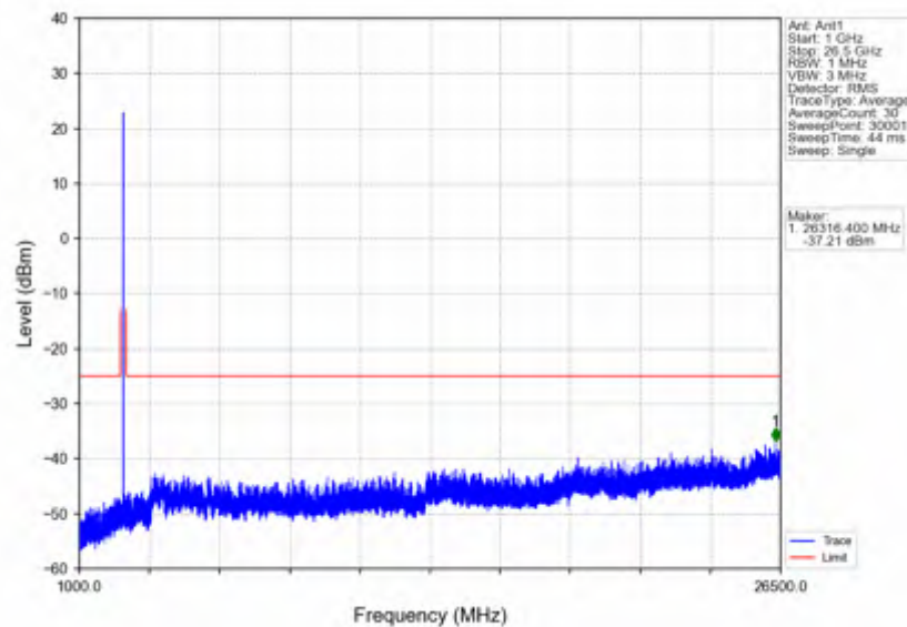
n41_30kHz_SISO_NTNV_10MHz_CP-OFDM QPSK_2592.99MHz_Edge_1RB_Left
