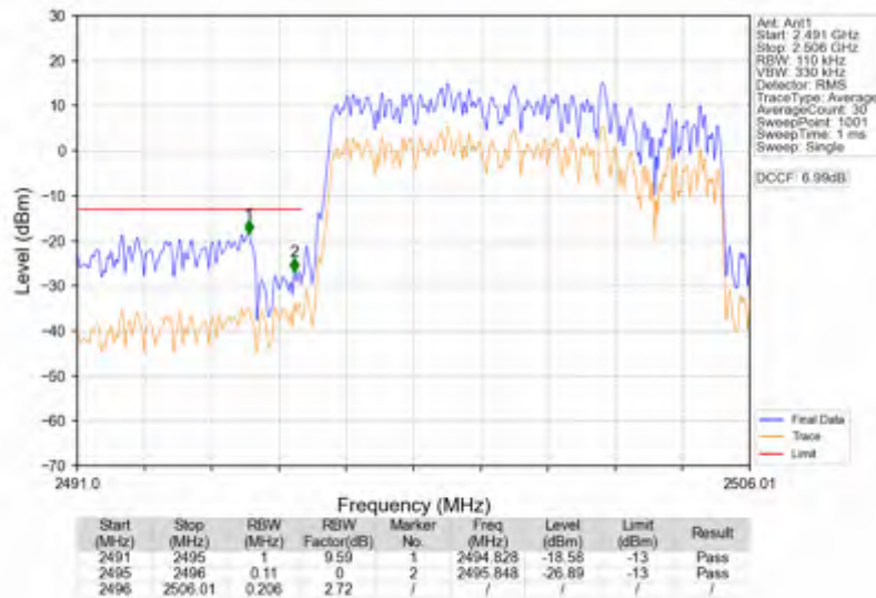
n41_30kHz_SISO_NTNV_10MHz_DFT-s-OFDM QPSK_2501.01MHz_Outer_Full
