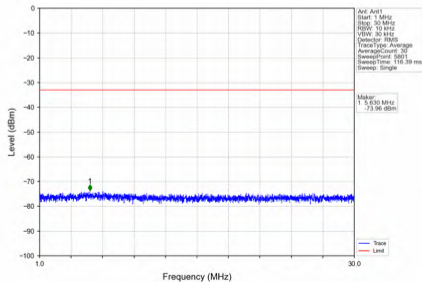
n41_15kHz_SISO_NTNV_50MHz_CP-OFDM QPSK_2664.99MHz_Outer_Full
