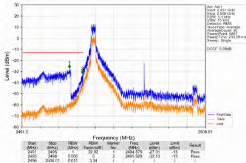
n41_30kHz_SISO_NTNV_10MHz_CP-OFDM_QPSK_2501.01MHz_Edge_1RB_Left
