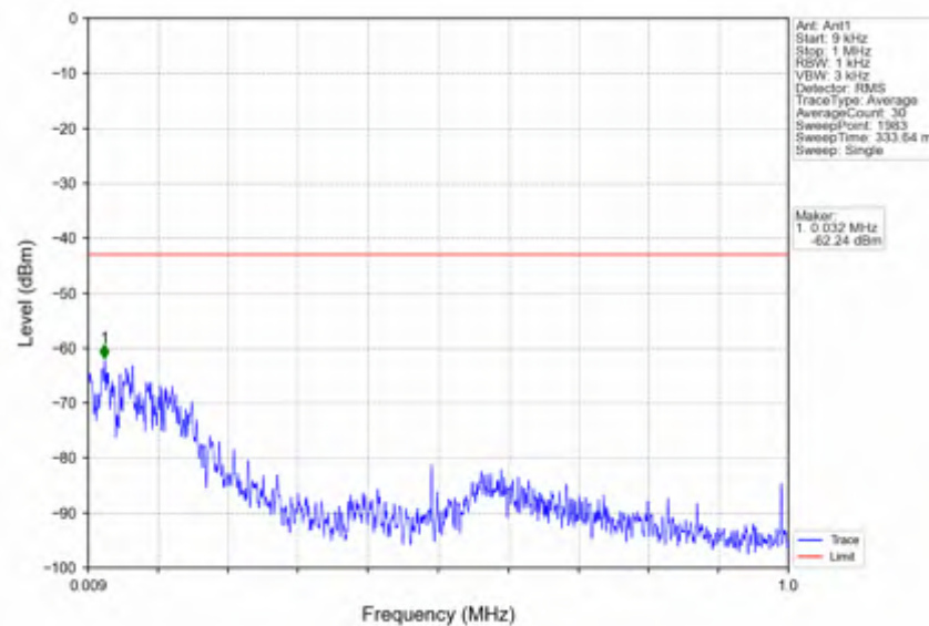
n41_15kHz_SISO_NTNV_40MHz_CP-OFDM_QPSK_2670MHz_Edge_1RB_Right
