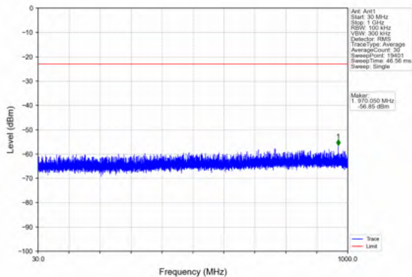
n41_30kHz_SISO_NTNV_10MHz_DFT-s-OFDM QPSK_2592.99MHz_Edge_1RB_Left
