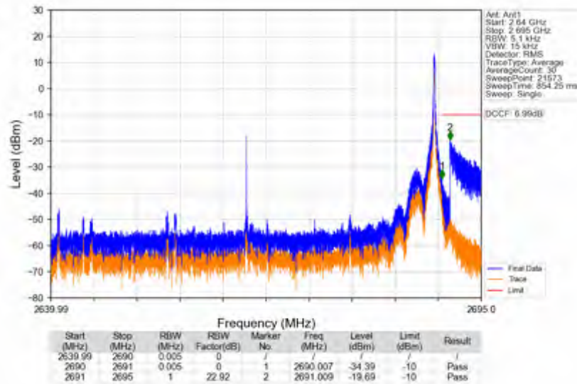
n41_15kHz_SISO_NTNV_50MHz_CP-OFDM_QPSK_2664.99MHz_Inner_1RB_Right
