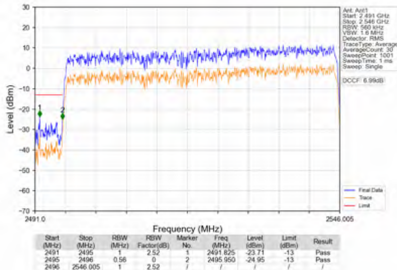
n41_15kHz_SISO_NTNV_50MHz_CP-OFDM QPSK_2521.005MHz_Outer_Full
