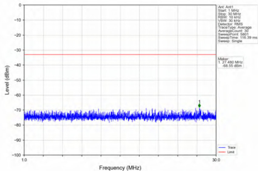
n41_30kHz_SISO_NTNV_10MHz_CP-OFDM QPSK_2592.99MHz_Edge_1RB_Left
