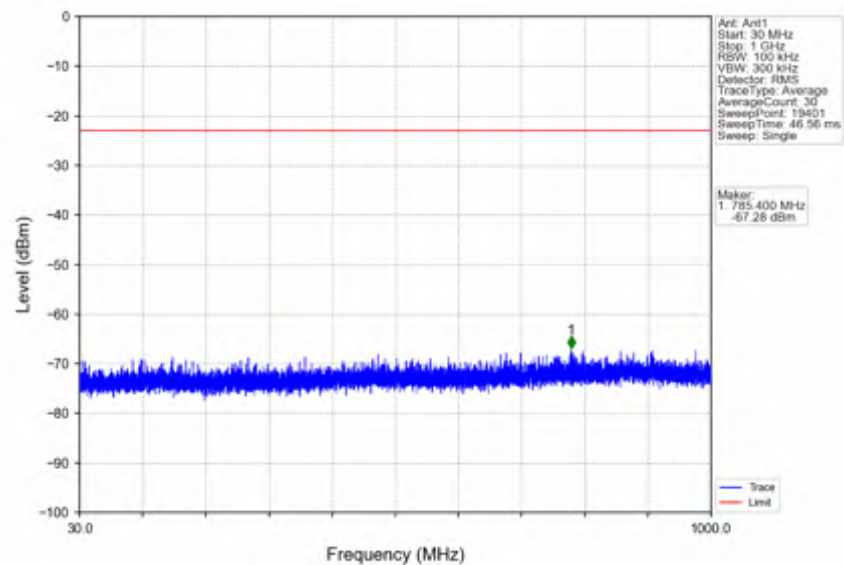
n41_15kHz_SISO_NTNV_40MHz_DFT-s-OFDM QPSK_2516.01MHz_Outer_Full
