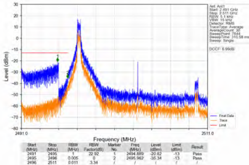
n41_30kHz_SISO_NTNV_15MHz_DFT-s-OFDM_QPSK_2503.5MHz_Inner_1RB_Left
