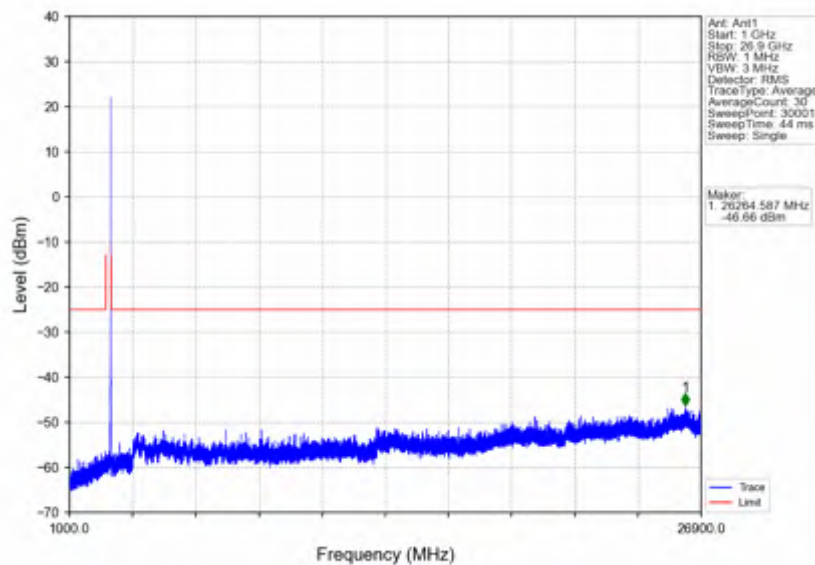
n41_30kHz_SISO_NTNV_10MHz_CP-OFDM QPSK_2685MHz_Outer_Full
