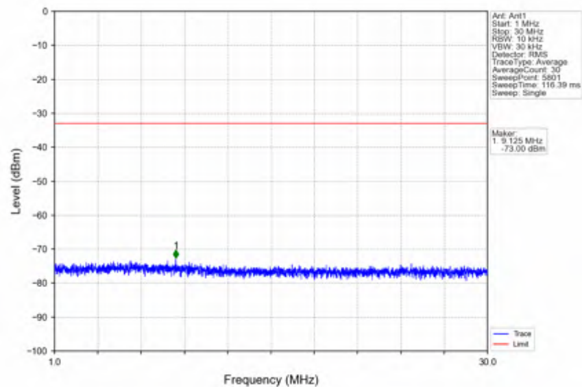
n41_15kHz_SISO_NTNV_40MHz_CP-OFDM_QPSK_2670MHz_Outer_Full
