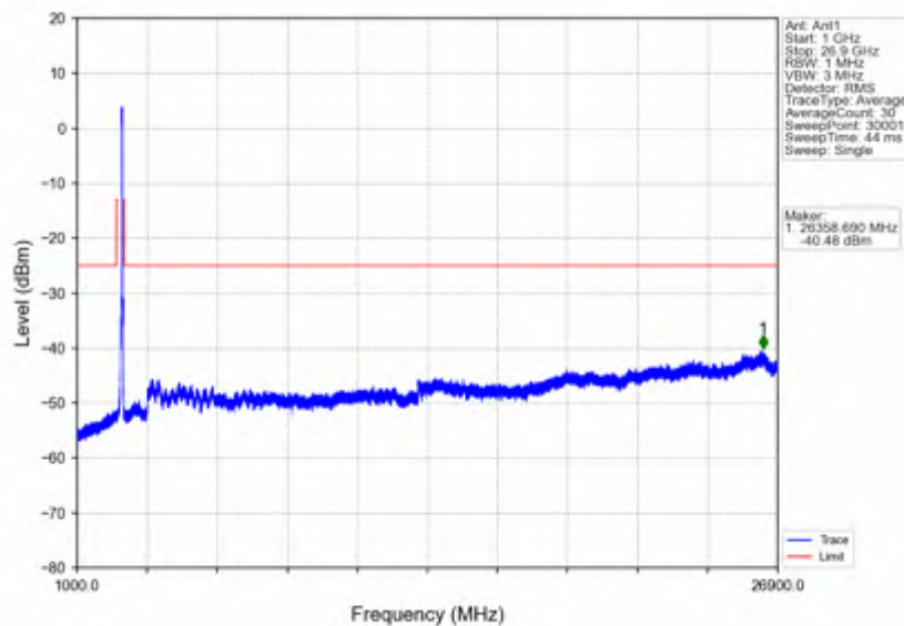
n41_15kHz_SISO_NTNV_50MHz_DFT-s-OFDM QPSK_2664.99MHz_Inner_1RB_Right
