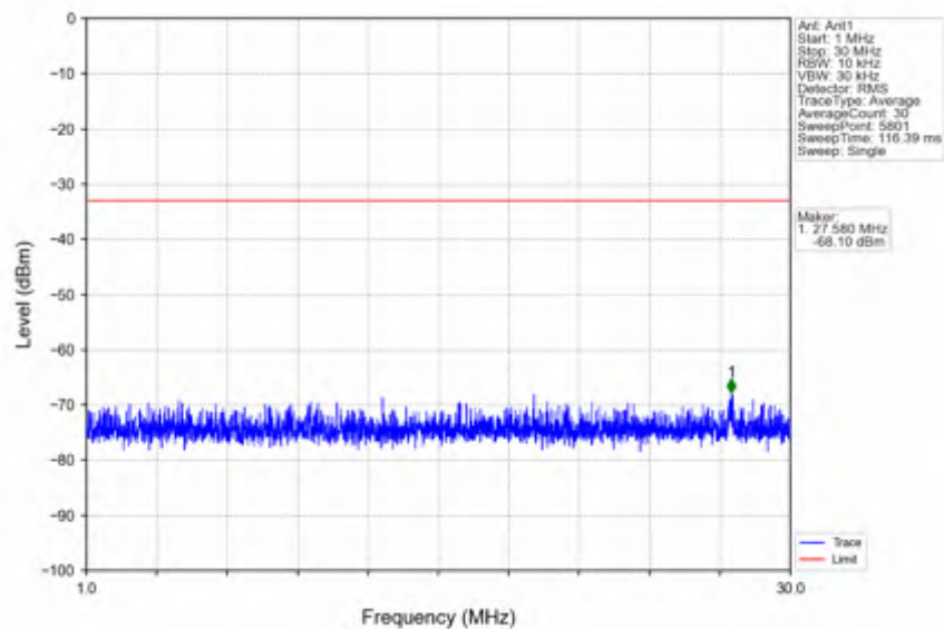
n41_30kHz_SISO_NTNV_10MHz_DFT-s-OFDM QPSK_2592.99MHz_Edge_1RB_Left
