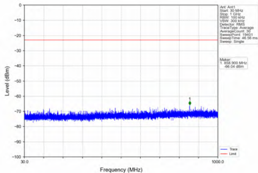
n41_15kHz_SISO_NTNV_40MHz_CP-OFDM QPSK_2516.01MHz_Outer_Full
