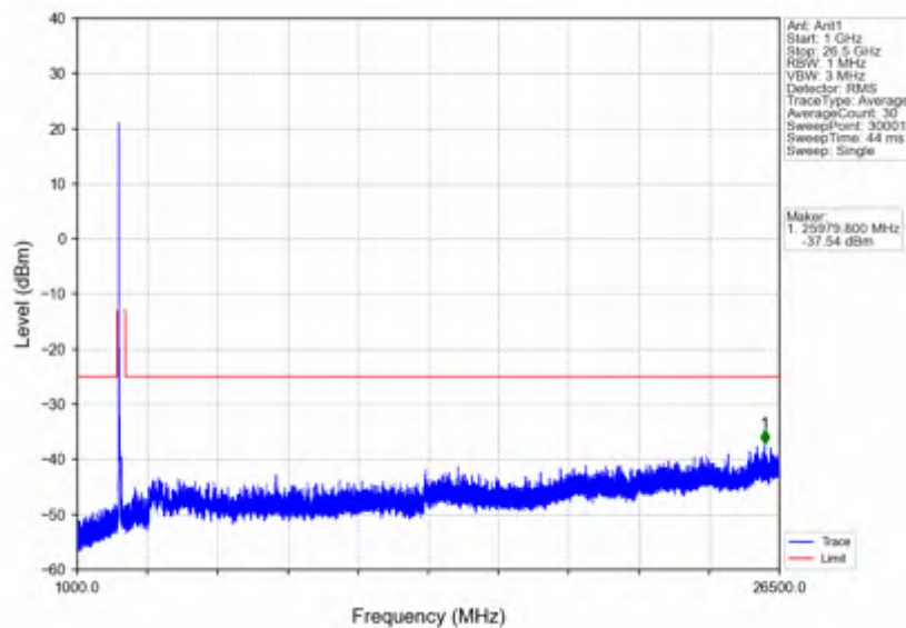
n41_15kHz_SISO_NTNV_50MHz_CP-OFDM QPSK_2521.005MHz_Outer_Full
