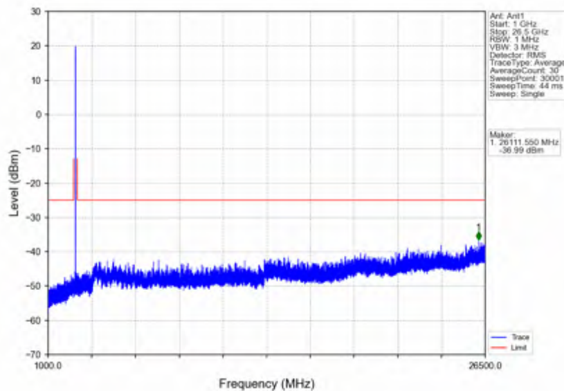
n41_30kHz_SISO_NTNV_10MHz_DFT-s-OFDM QPSK_2685MHz_Edge_1RB_Right
