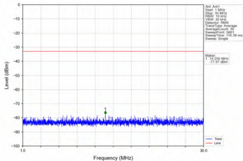
n41_30kHz_SISO_NTNV_10MHz_CP-OFDM QPSK_2501.01MHz_Outer_Full
