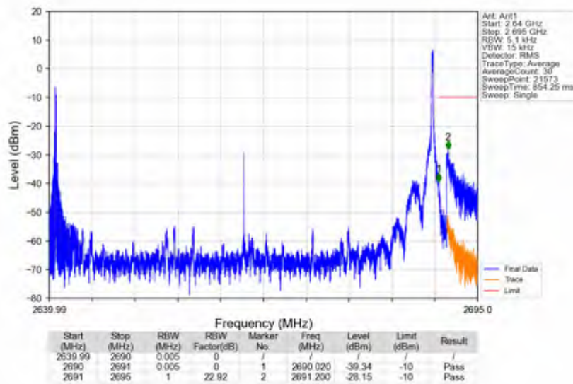
n41_15kHz_SISO_NTNV_50MHz_DFT-s-OFDM QPSK_2664.99MHz_Edge_1RB_Right
