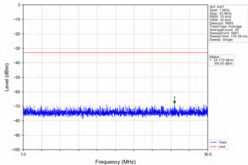
n41_30kHz_SISO_NTNV_10MHz_DFT-s-OFDM QPSK_2501.01MHz_Edge_1RB_Left
