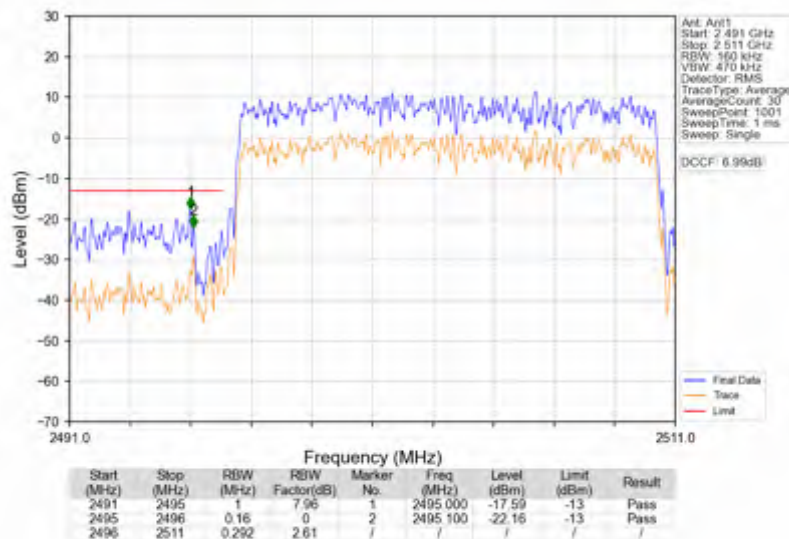
n41_30kHz_SISO_NTV_15MHz_CP-OFDM QPSK_2503.5MHz_Outer_Full
