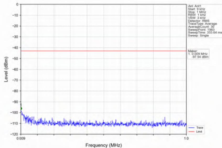
n41_15kHz_SISO_NTNV_40MHz_CP-OFDM QPSK_2516.01MHz_Outer_Full
