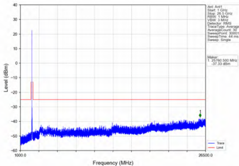
n41_15kHz_SISO_NTNV_40MHz_DFT-s-OFDM QPSK_2670MHz_Edge_1RB_Right
