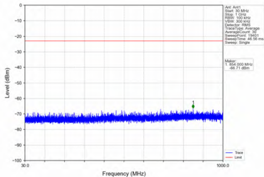
n41_30kHz_SISO_NTNV_10MHz_DFT-s-OFDM_PI/2_BPSK_2685MHz_Outer_Full
