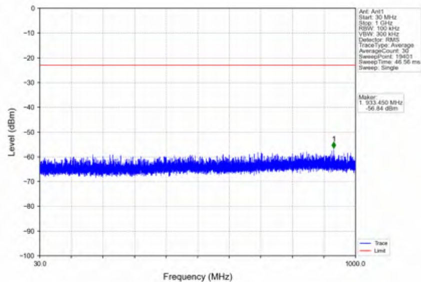
n41_30kHz_SISO_NTNV_10MHz_CP-OFDM QPSK_2592.99MHz_Edge_1RB_Left
