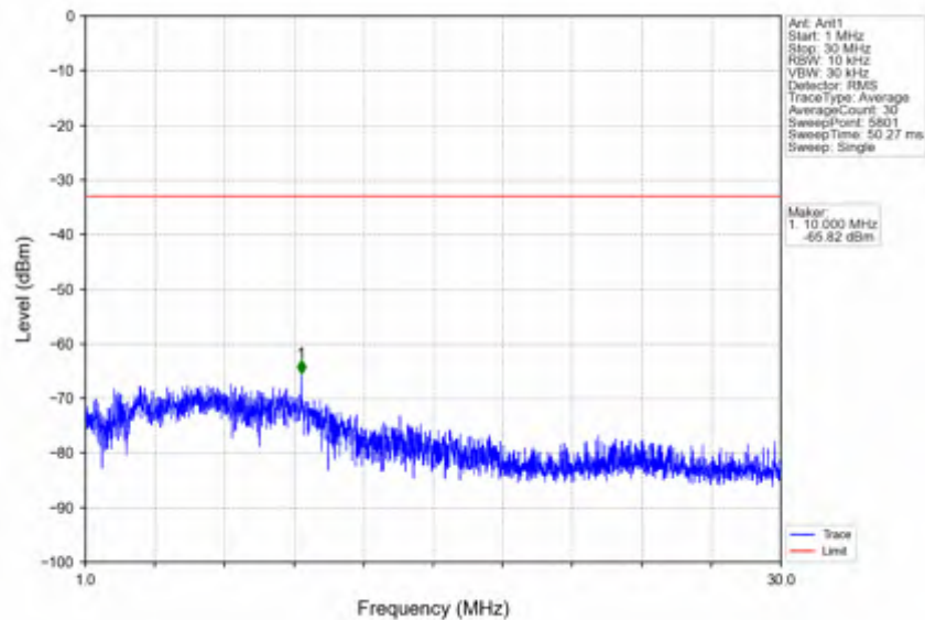
n41_15kHz_SISO_NTNV_40MHz_DFT-s-OFDM_PI/2_BPSK_2670MHz_Outer_Full
