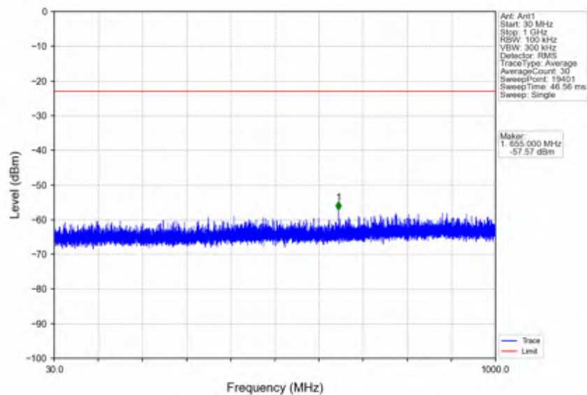
n41_15kHz_SISO_NTNV_50MHz_DFT-s-OFDM QPSK_2664.99MHz_Edge_1RB_Right
