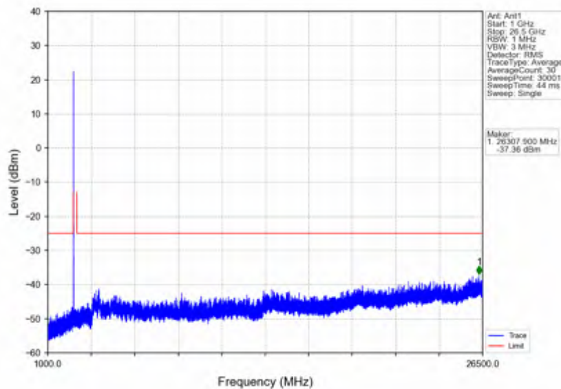
n41_30kHz_SISO_NTNV_10MHz_CP-OFDM QPSK_2501.01MHz_Outer_Full
