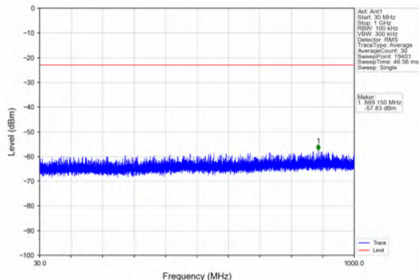
n41_30kHz_SISO_NTV_15MHz_CP-OFDM_QPSK_2503.5MHz_Edge_1RB_Left
