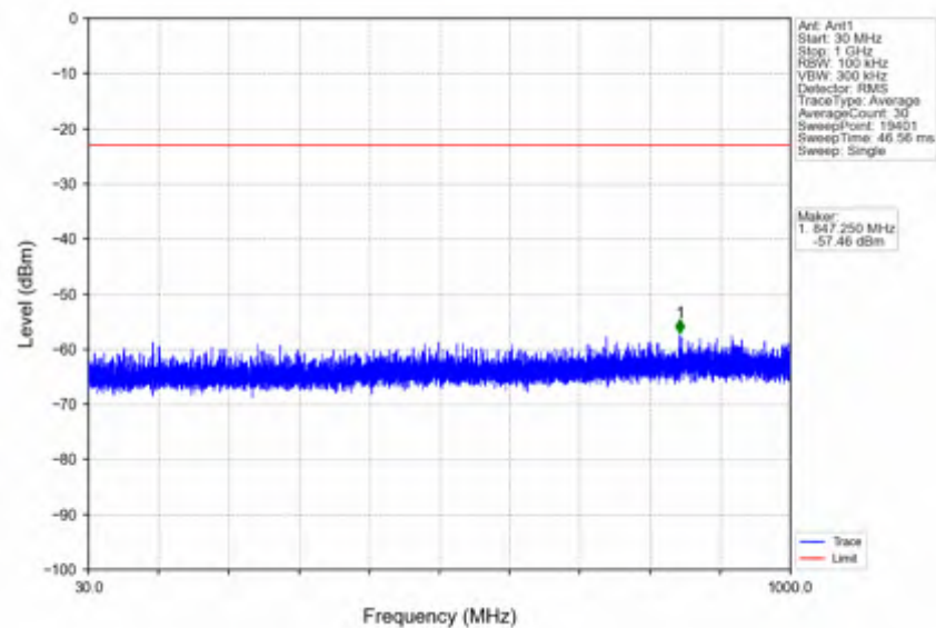
n41_15kHz_SISO_NTNV_40MHz_DFT-s-OFDM_QPSK_2670MHz_Edge_1RB_Right
