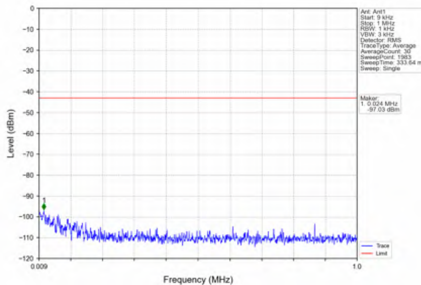
n41_15kHz_SISO_NTNV_50MHz_CP-OFDM_QPSK_2664.99MHz_Inner_1RB_Right
