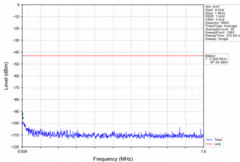
n41_30kHz_SISO_NTNV_15MHz_DFT-s-OFDM_QPSK_2682.48MHz_Outer_Full
