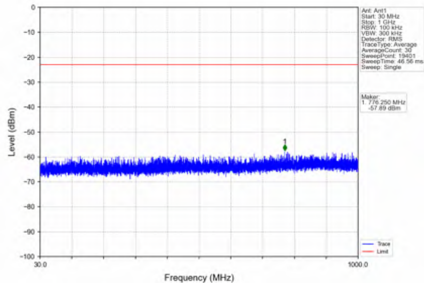
n41_30kHz_SISO_NTNV_10MHz_DFT-s-OFDM QPSK_2685MHz_Edge_1RB_Right
