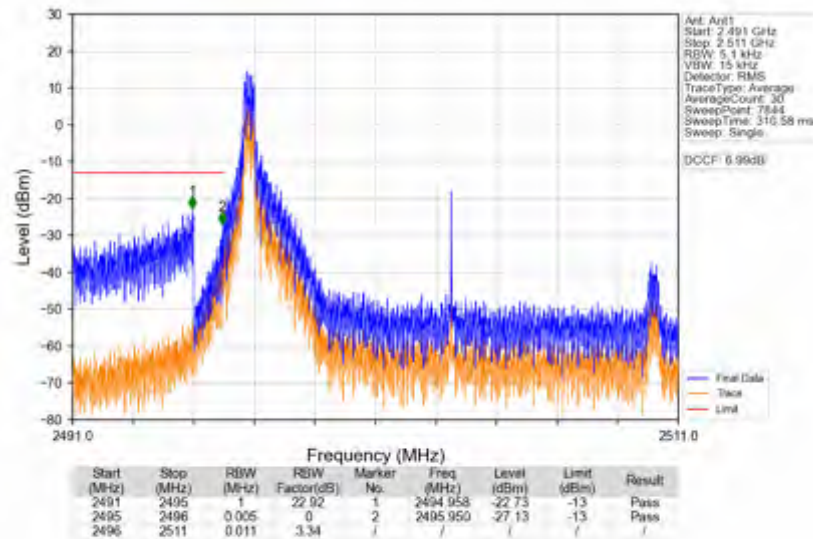
n41_30kHz_SISO_NTNV_15MHz_CP-OFDM_QPSK_2503.5MHz_Edge_1RB_Left
