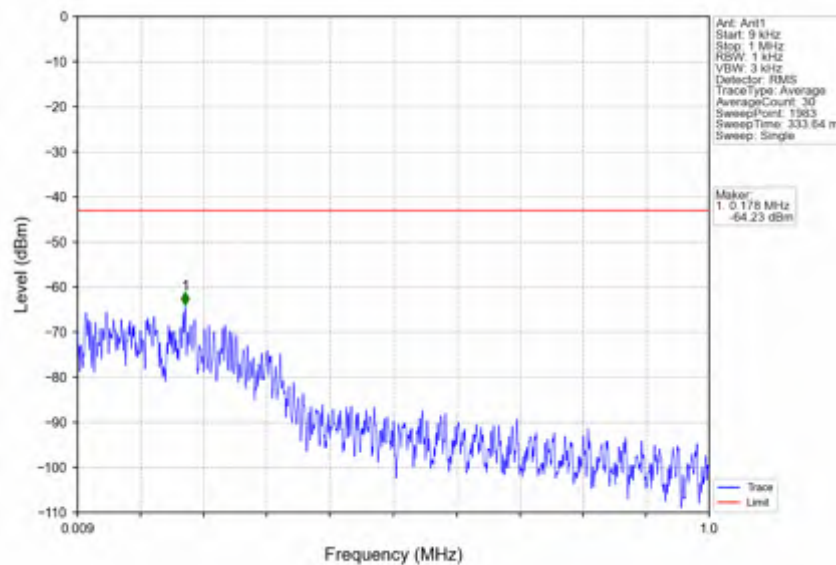
n41_30kHz_SISO_NTNV_15MHz_CP-OFDM_QPSK_2503.5MHz_Edge_1RB_Left
