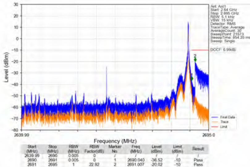
n41_15kHz_SISO_NTNV_50MHz_DFT-s-OFDM QPSK_2664.99MHz_Inner_1RB_Right
