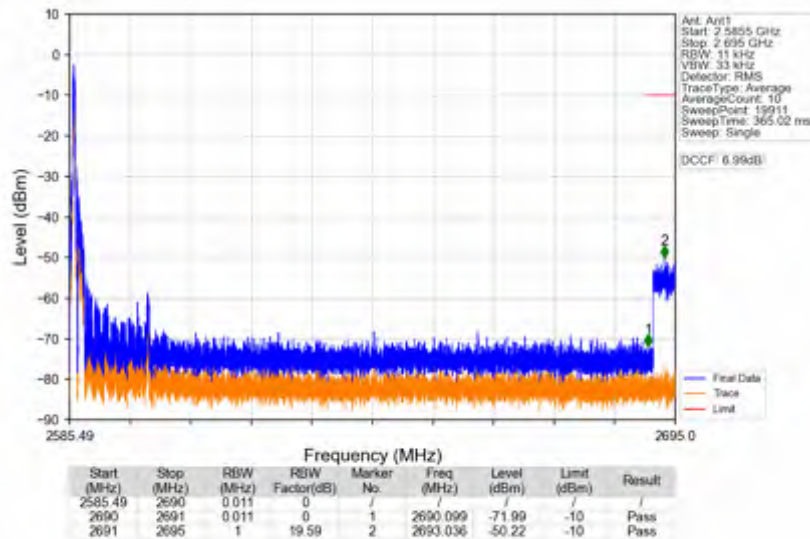
n41_30kHz_SISO_NTNV_15MHz_DFT-s-OFDM_PI/2_BPSK_2592.99MHz_Edge_1RB_Left
