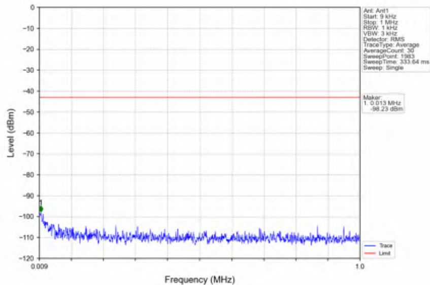
n41_30kHz_SISO_NTNV_10MHz_CP-OFDM QPSK_2685MHz_Outer_Full
