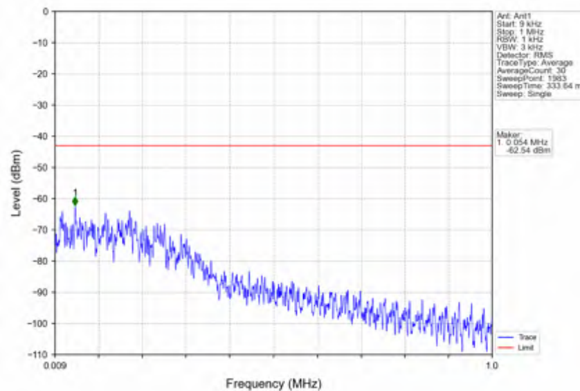
n41_30kHz_SISO_NTNV_10MHz_CP-OFDM_QPSK_2685MHz_Edge_1RB_Right
