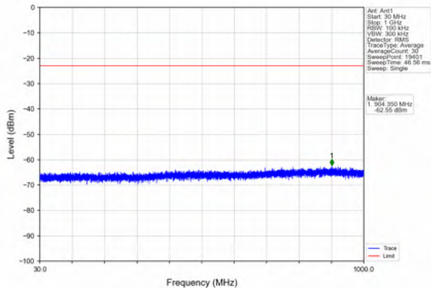
n41_15kHz_SISO_NTNV_40MHz_CP-OFDM_QPSK_2670MHz_Outer_Full
