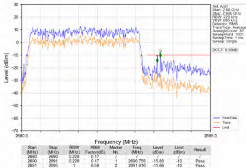
n41_30kHz_SISO_NTNV_10MHz_CP-OFDM QPSK_2685MHz_Outer_Full
