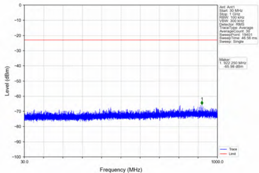
n41_30kHz_SISO_NTNV_15MHz_DFT-s-OFDM_QPSK_2503.5MHz_Outer_Full
