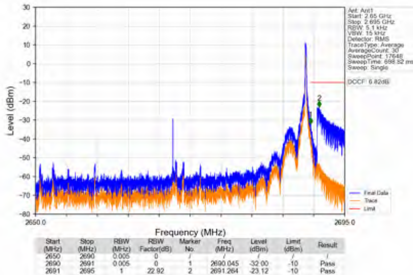
n41_15kHz_SISO_NTNV_40MHz_DFT-s-OFDM QPSK_2670MHz_Edge_1RB_Right
