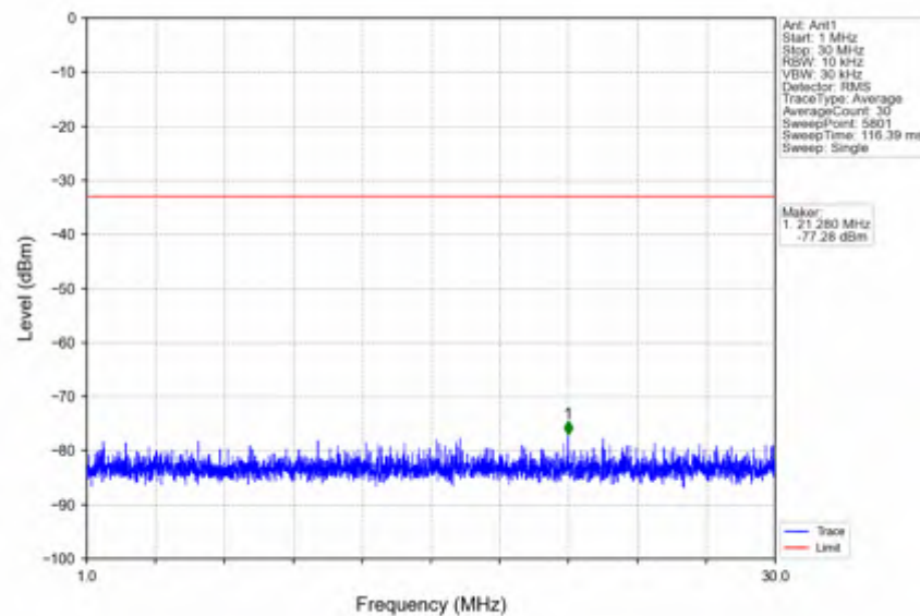
n41_15kHz_SISO_NTNV_50MHz_DFT-s-OFDM QPSK_2521.005MHz_Outer_Full
