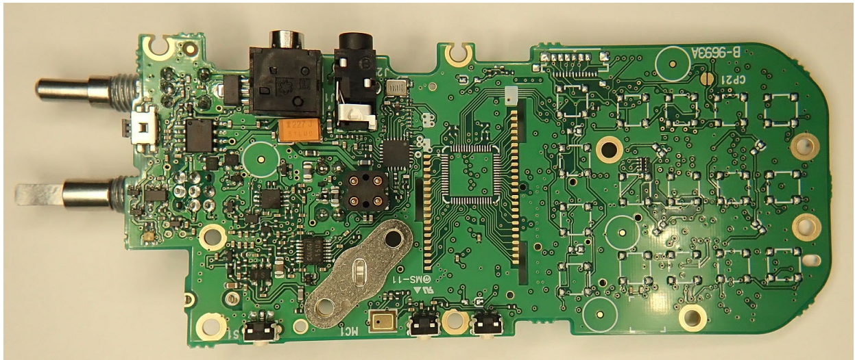
IC-V10MR MAIN SIDE A
