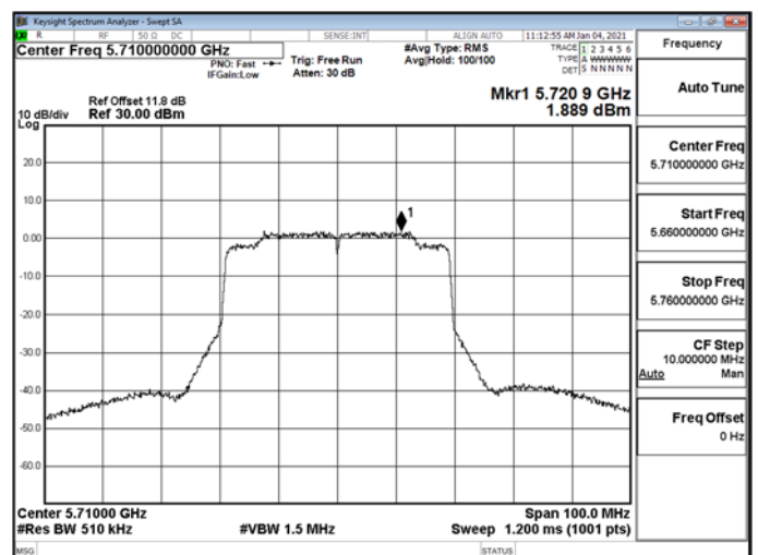
802.11ax_40MHz_5710MHz_UNII 3
