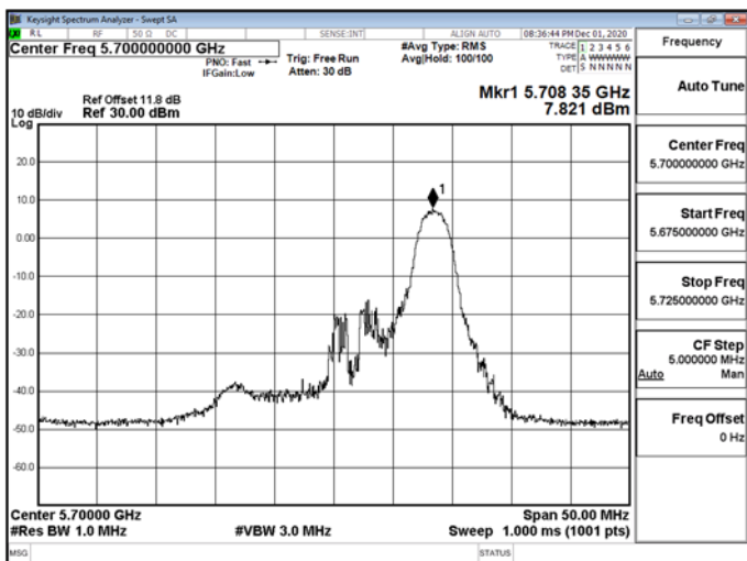
802.11ax_20MHz_RU_52_40_5700MHz-5700
