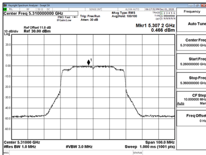
802.11ax_40MHz_RU_242_62_5310MHz-5310
