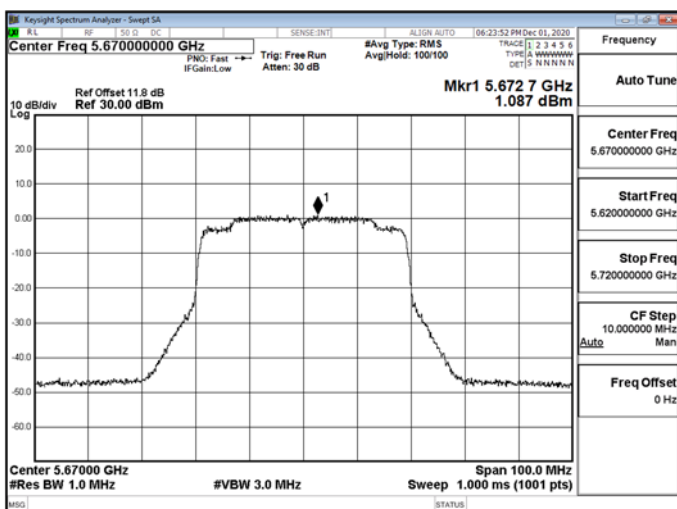
802.11ax_40MHz_5670MHz-5670
