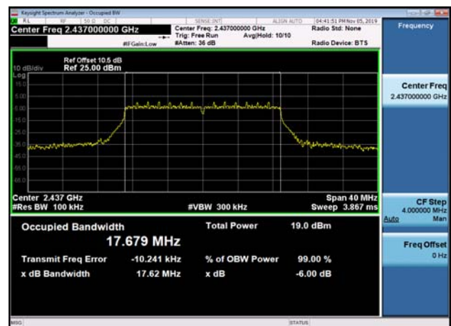
6dB Bandwidth-802.11n(HT20),2437MHz
