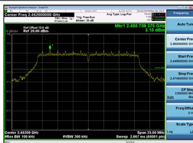
,Plot 1,Reference Level-802.11g ,2462MHz
