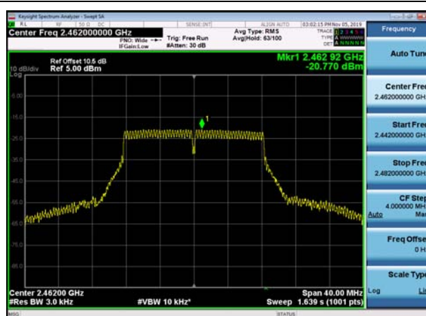
Power spectral density-802.11g ,2462MHz
