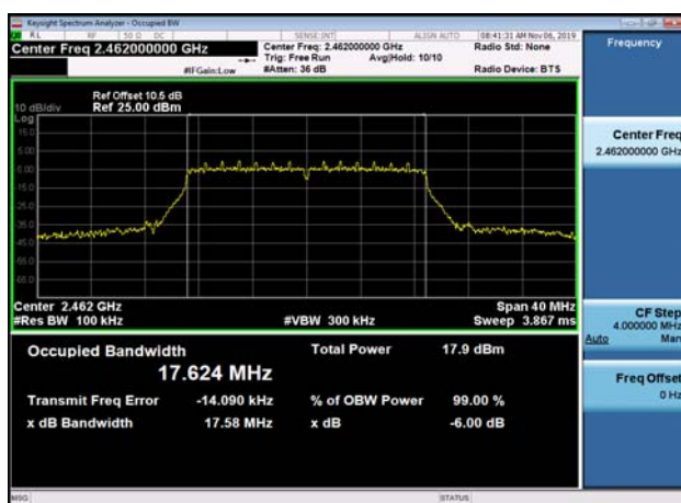
6dB Bandwidth-802.11n(HT20),2462MHz
