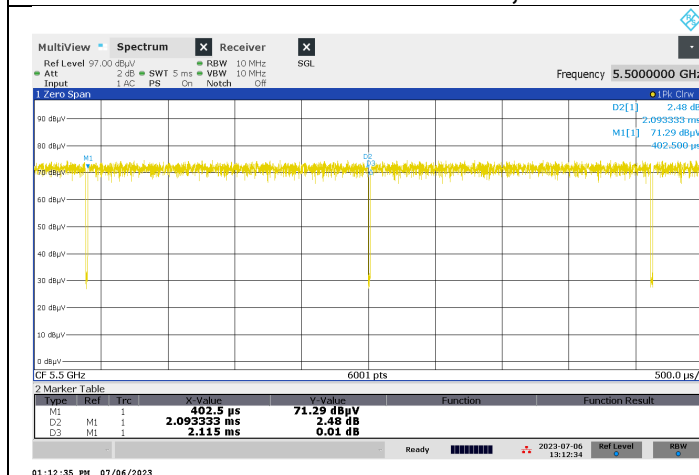
DUTY CYCLE 802.11a, 6Mbps
