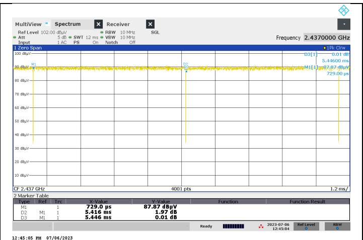
DUTY CYCLE 802.11n HT20
