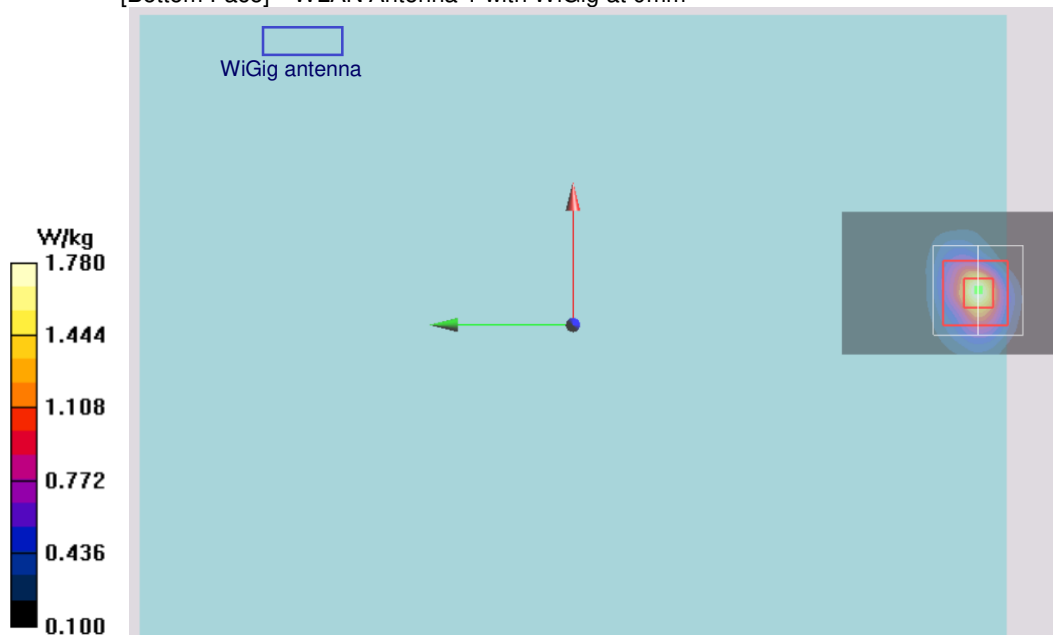
[Bottom Face] WLAN Antenna 1 with WiGig at 0mm
