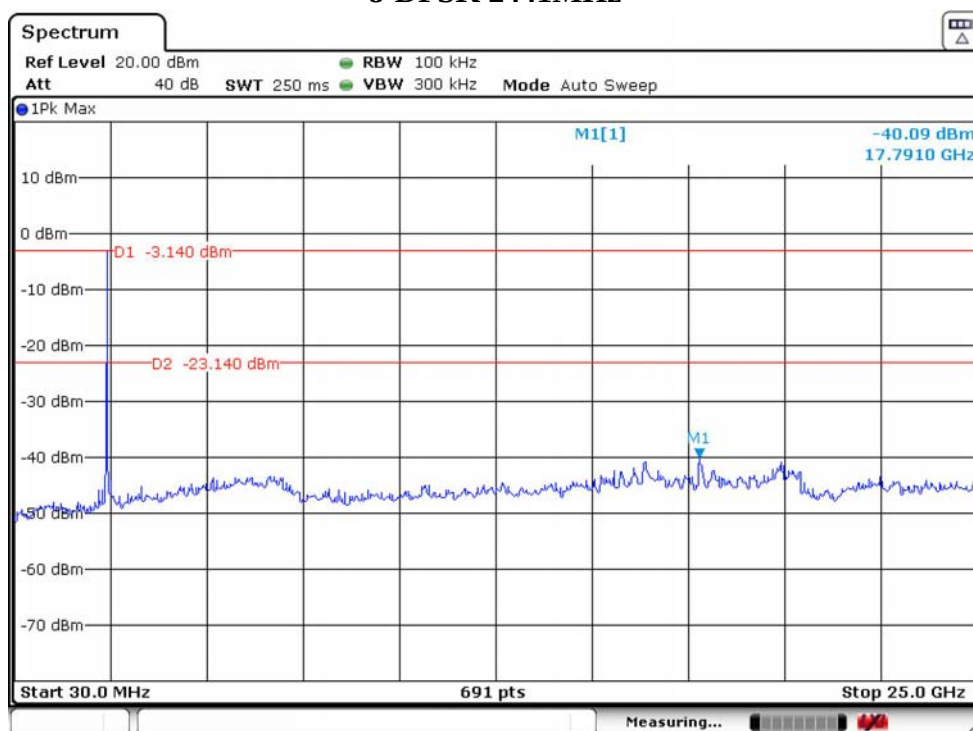
8-DPSK 2441MHz
