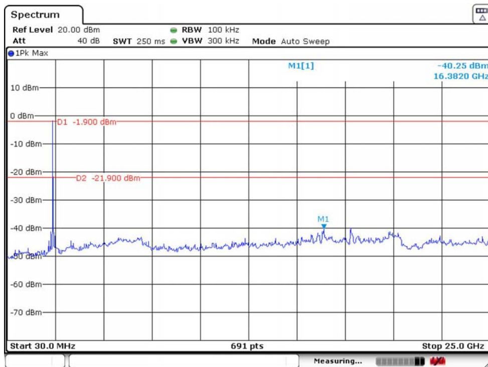
8-DPSK 2402MHz
