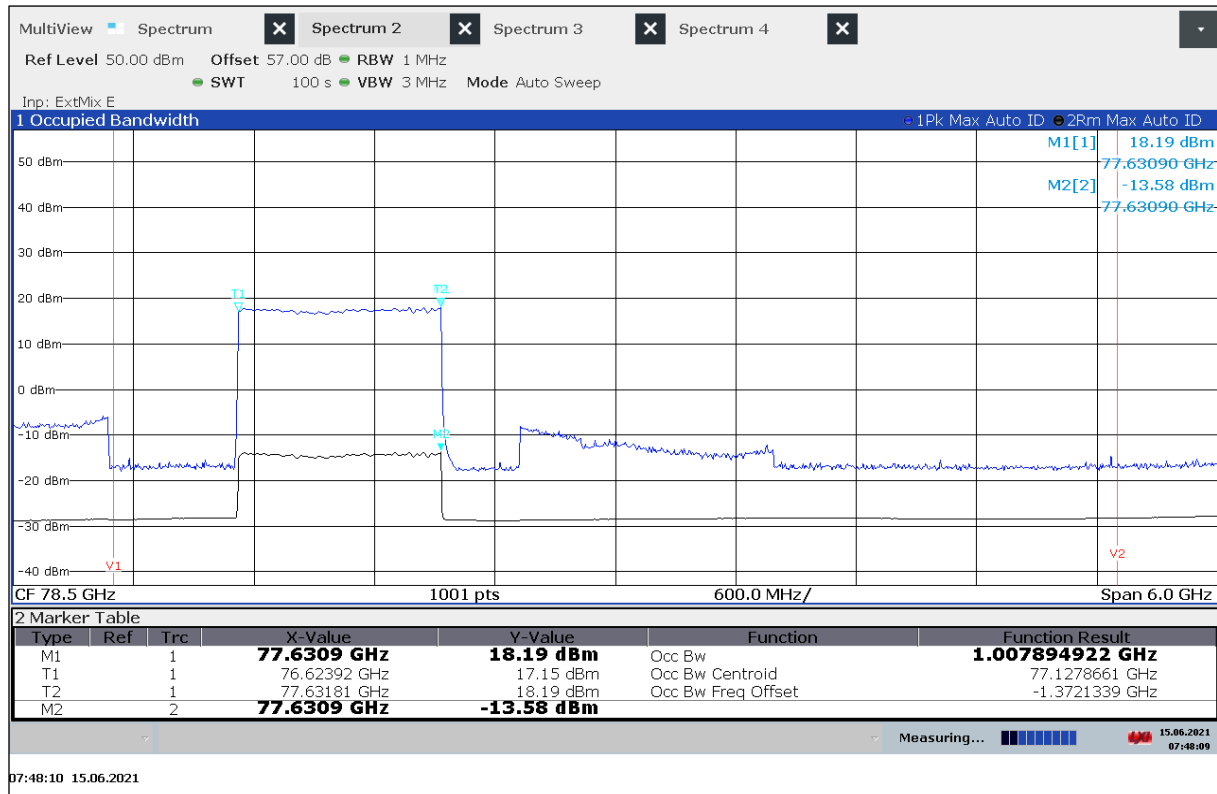
Plot 20: OBW, 30 °C / V_{\text{nom}}
