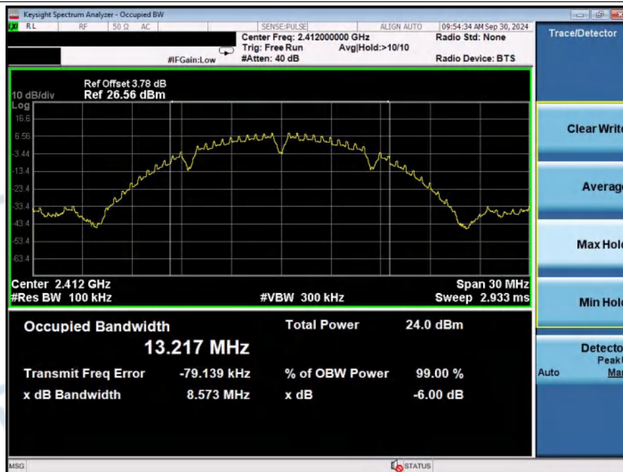
-6dB_Bandwidth_NVNT_ANT1_802_11b_2412
