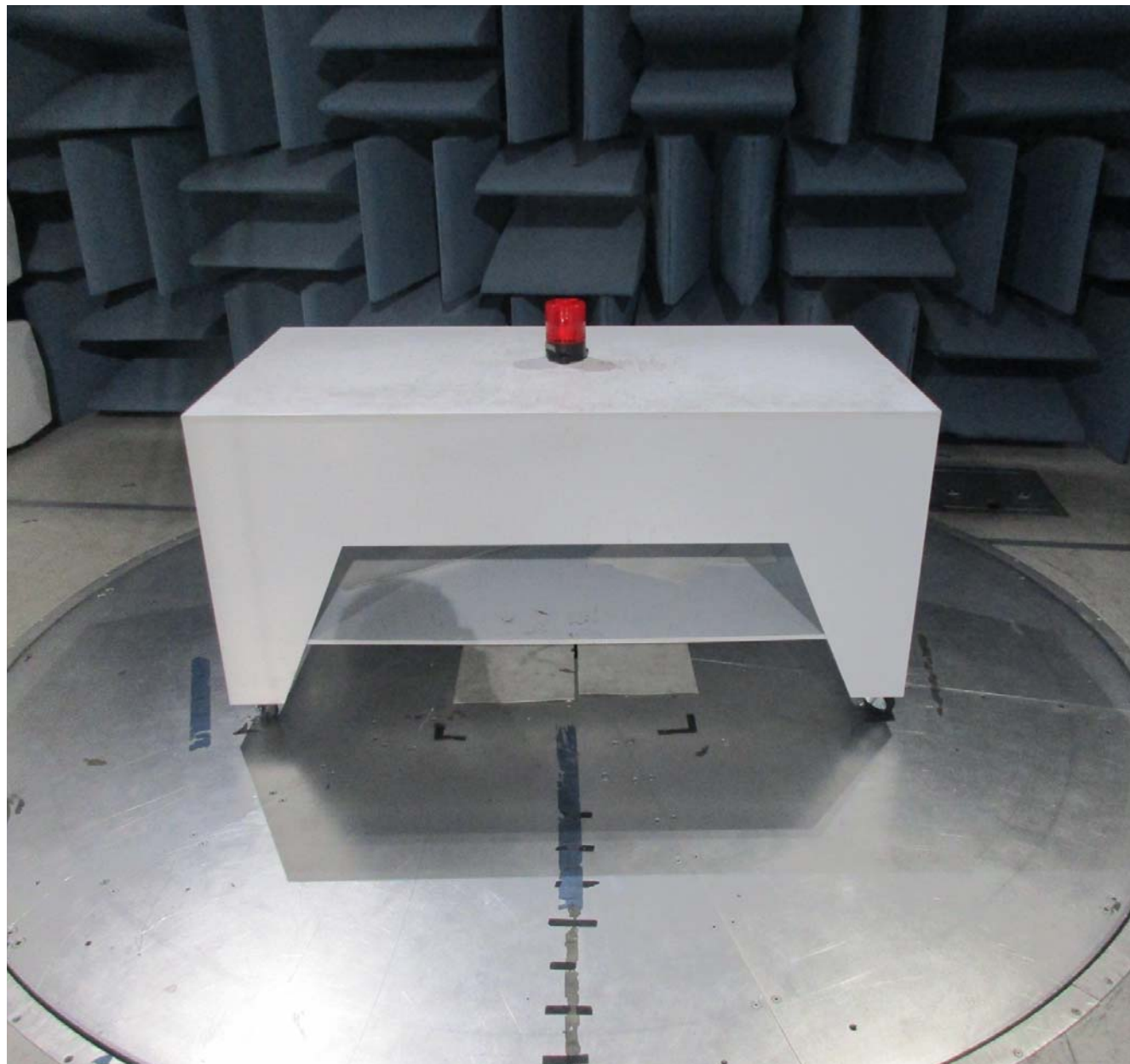
FRONT VIEW FCC Class A - Radiated Emissions (<1GHz)
