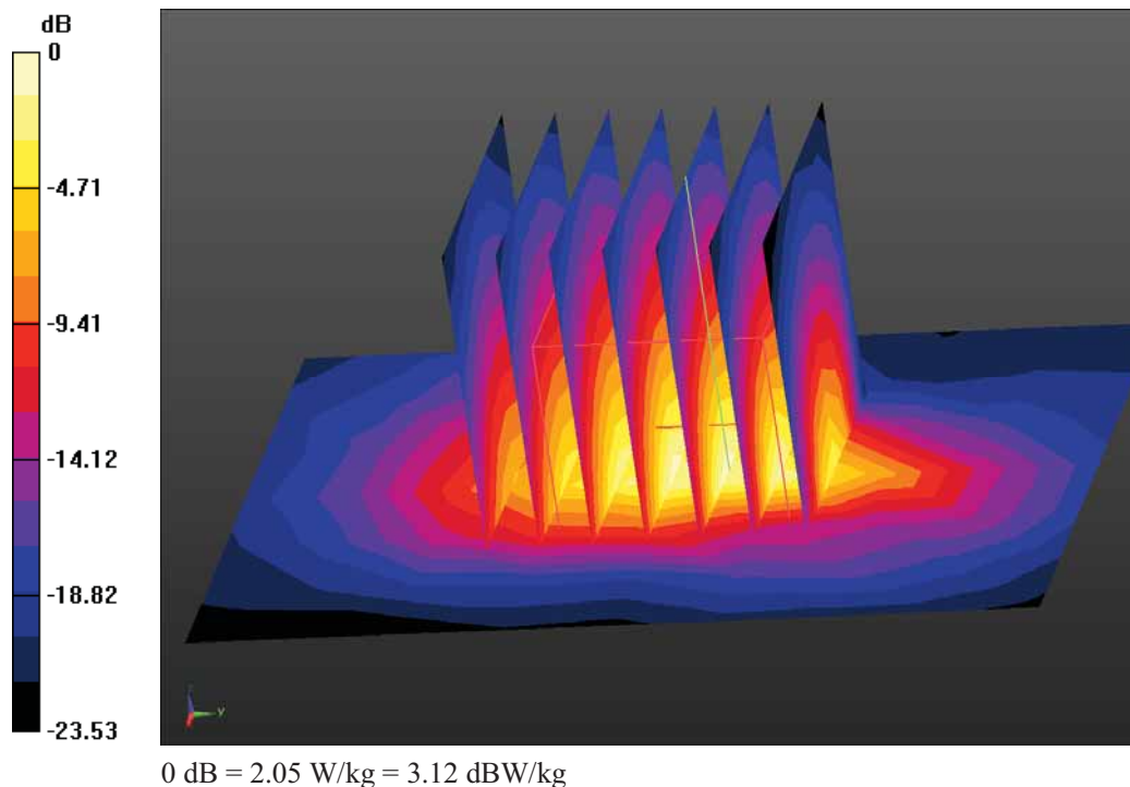
Fig. 2 - Up Side Low 802.11b Channel 1
