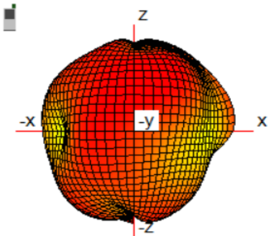
3D Radiation Pattern @ 2400 MHz
