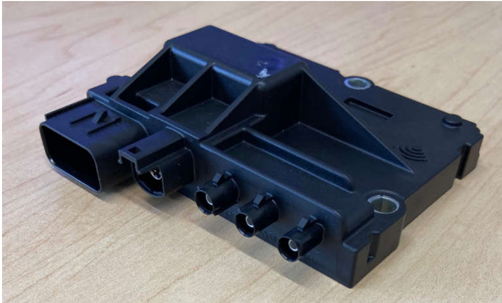
Parshall-External Photos
