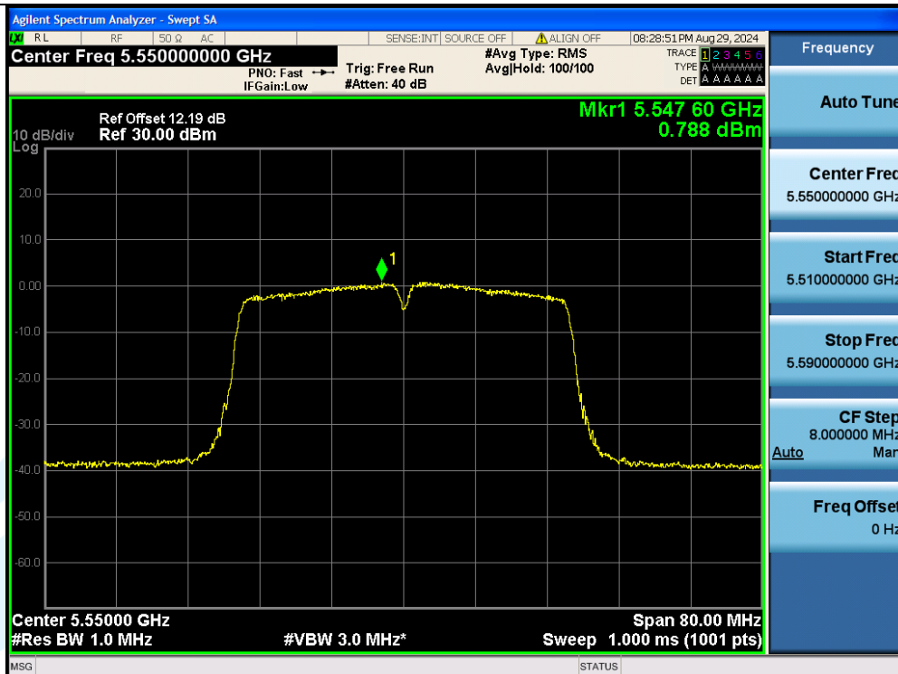
11AC40MIMO-Ant2-5550-PASS
