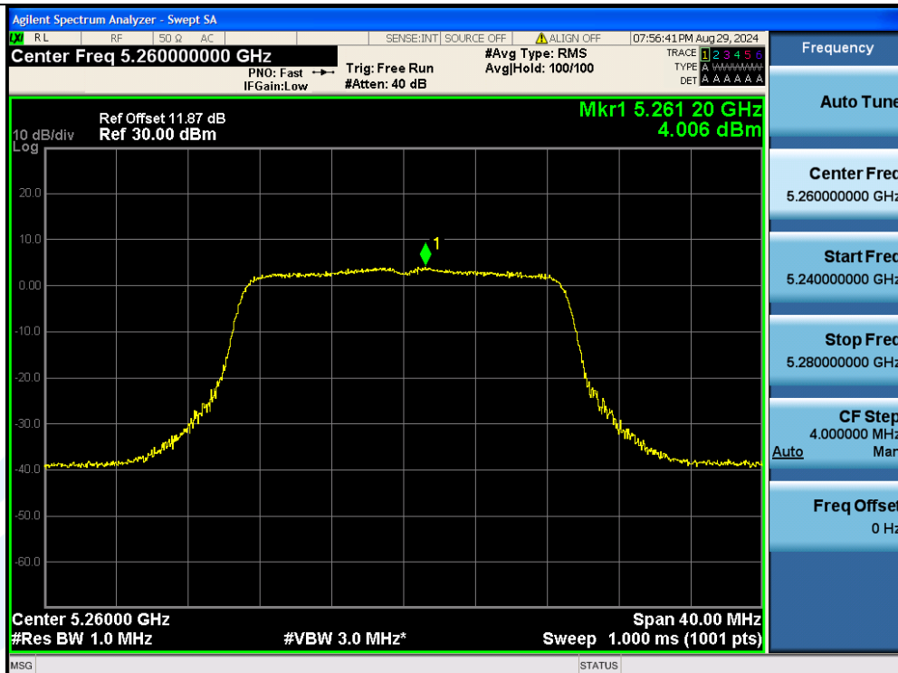
11N20MIMO-Ant2-5260-PASS
