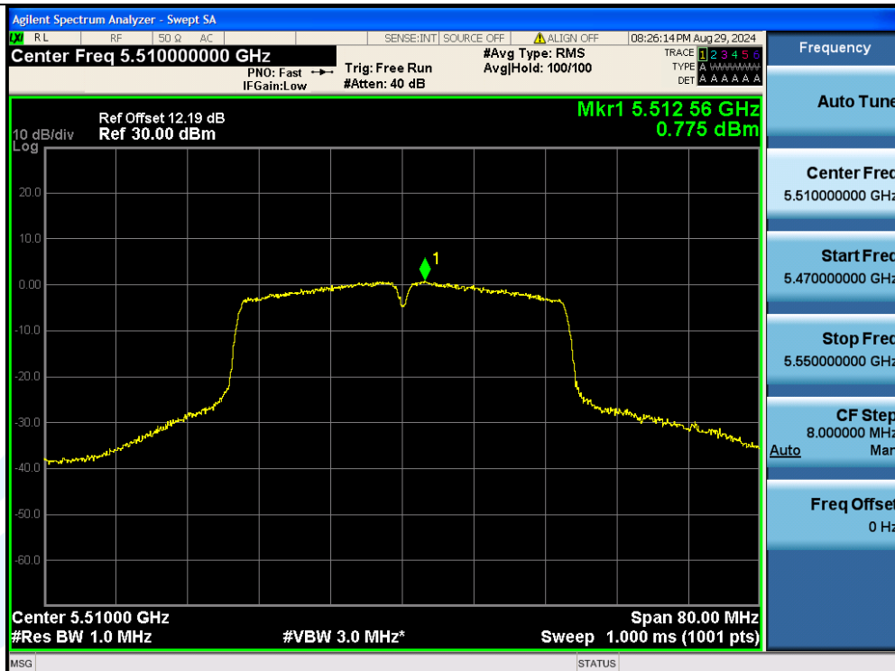
11AC40MIMO-Ant2-5510-PASS
