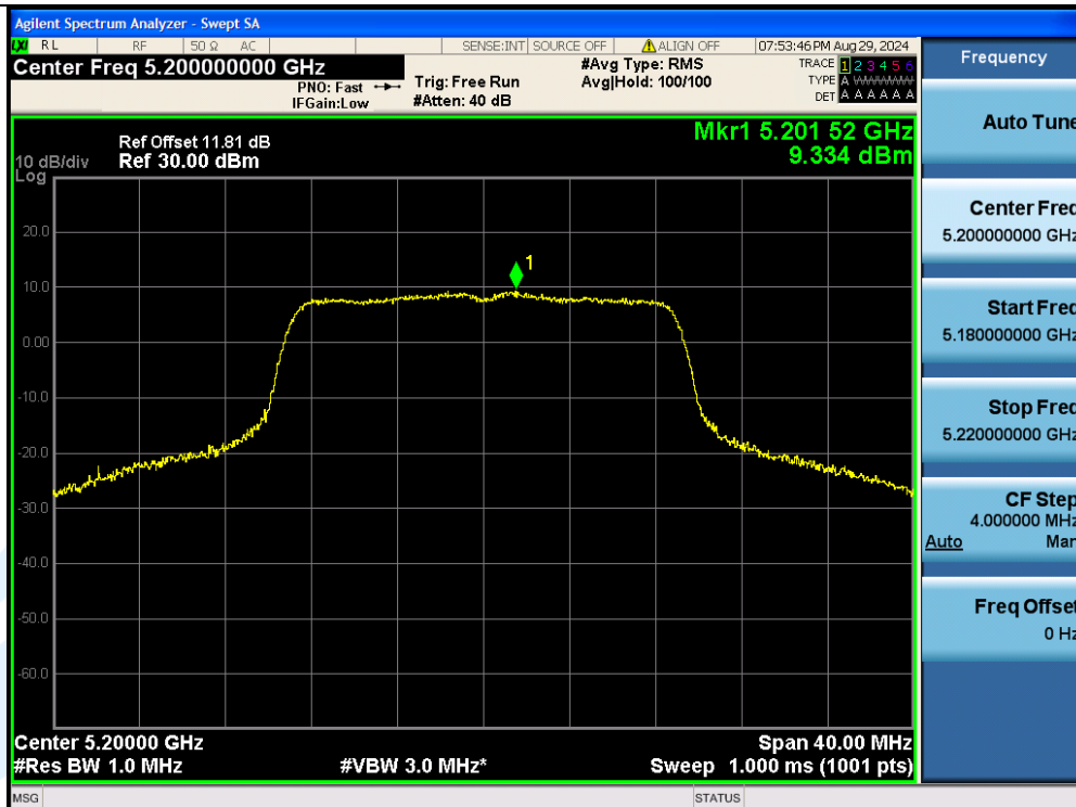
11N20MIMO-Ant2-5200-PASS
