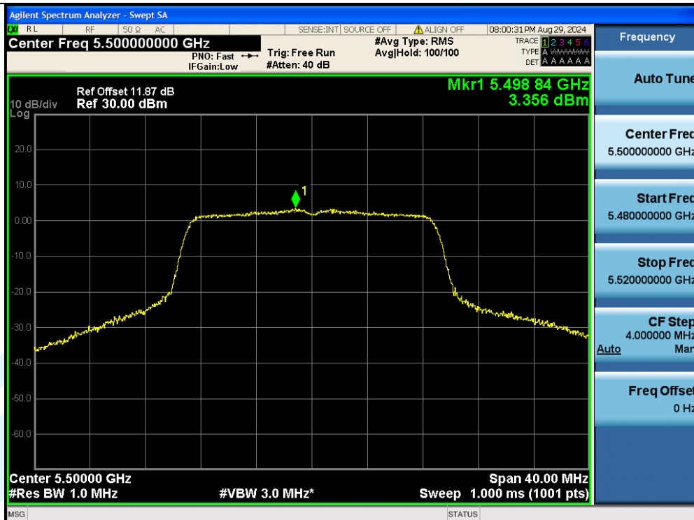
11N20MIMO-Ant2-5500-PASS
