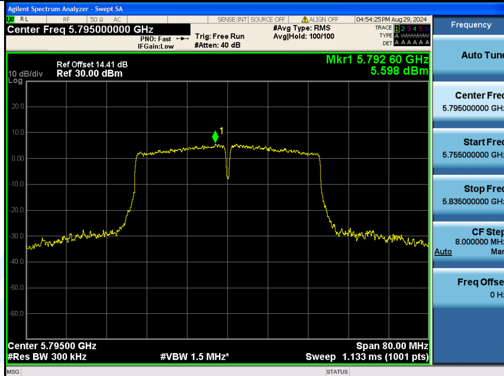
11AC40MIMO-Ant2-5795-PASS
