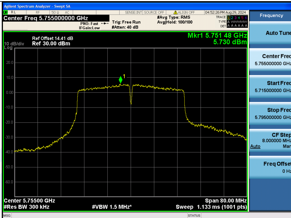
11AC40MIMO-Ant2-5755-PASS
