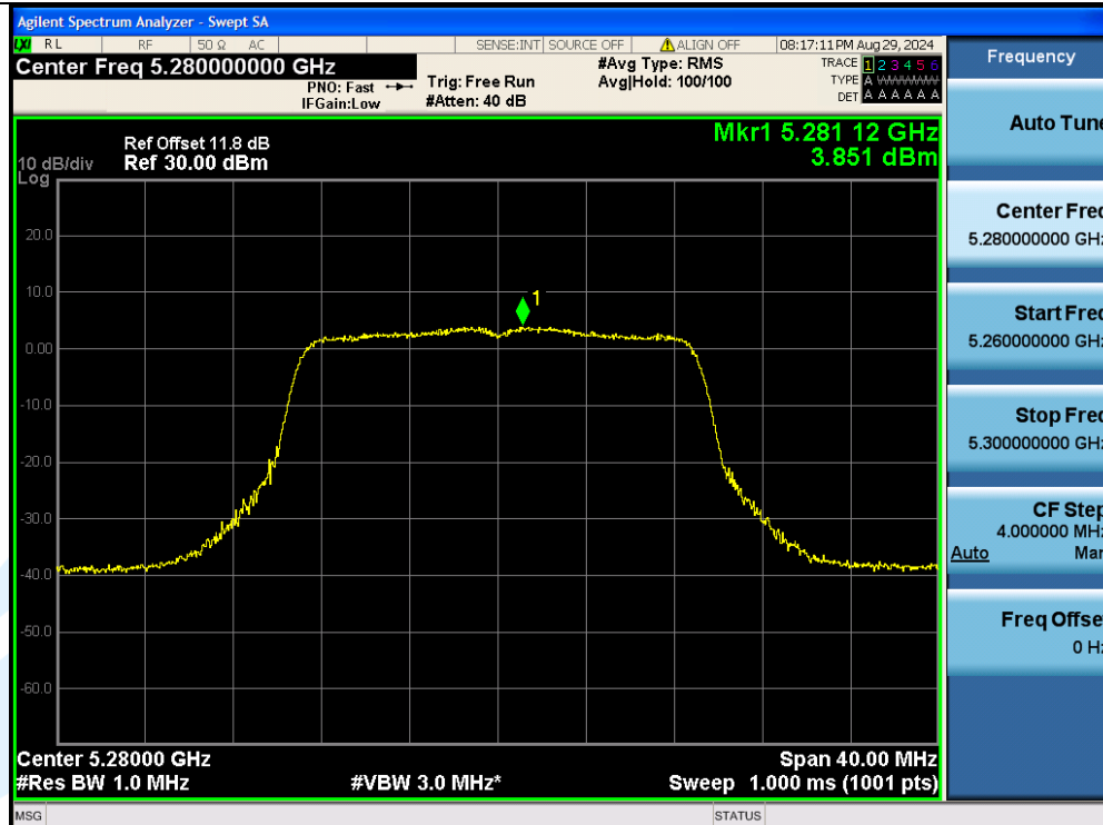
11AC20MIMO-Ant2-5280-PASS
