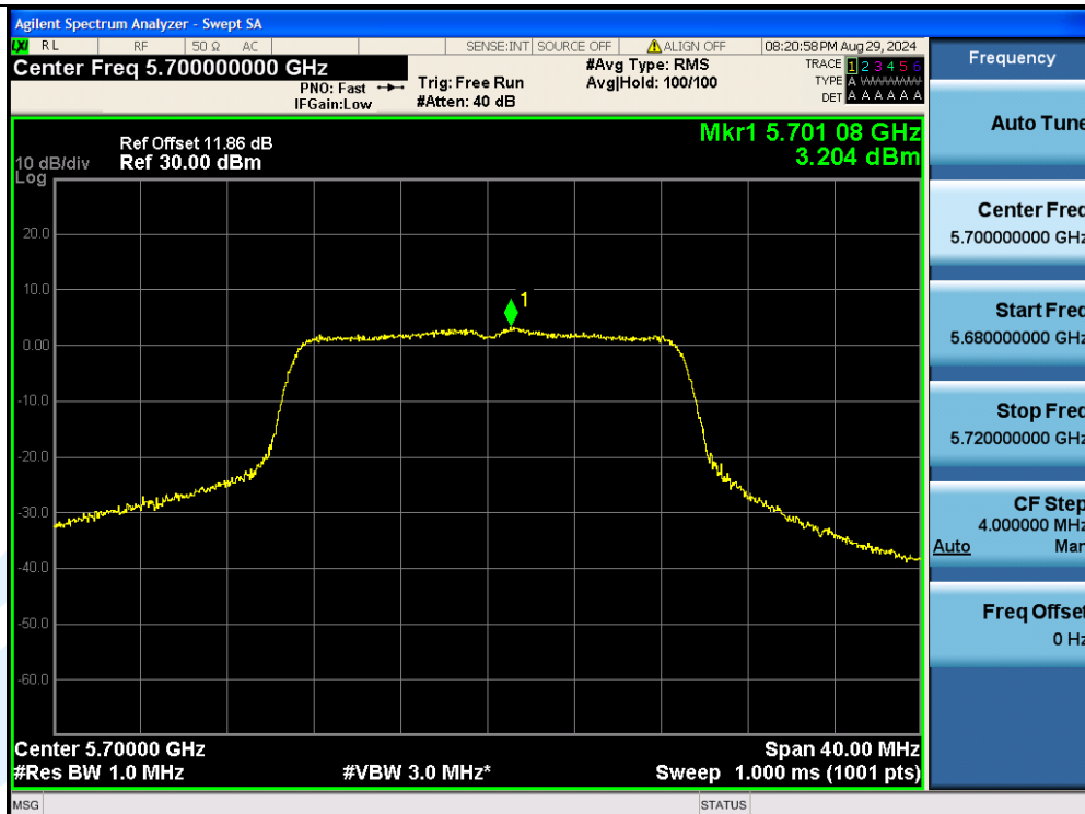
11AC20MIMO-Ant2-5700-PASS
