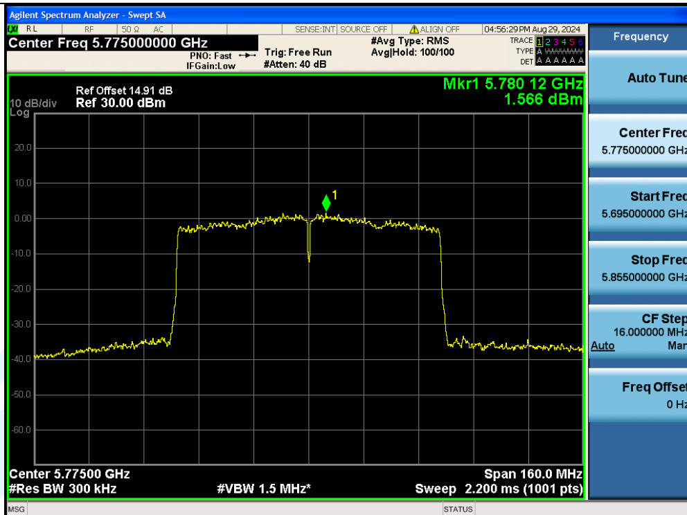
11AC80MIMO-Ant2-5775-PASS
