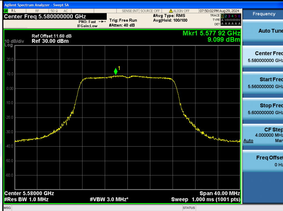
11A-Ant2-5580-PASS
