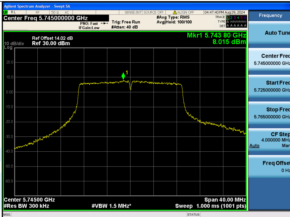
11AC20MIMO-Ant2-5745-PASS
