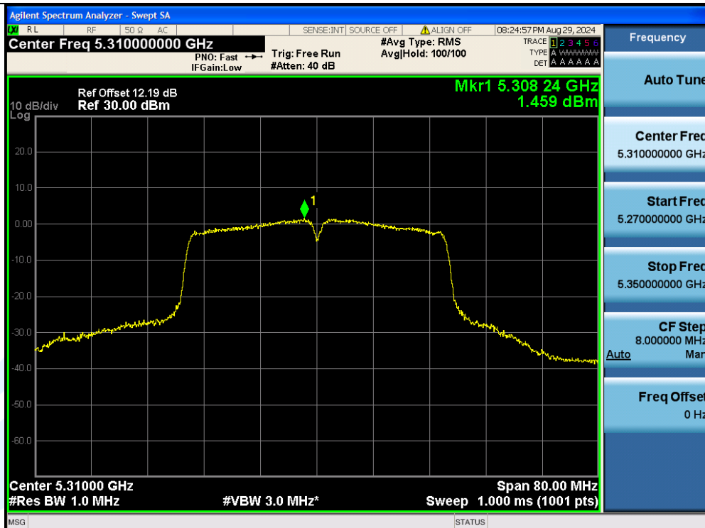
11AC40MIMO-Ant2-5310-PASS
