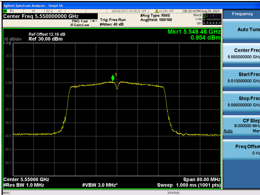
11N40MIMO-Ant2-5550-PASS
