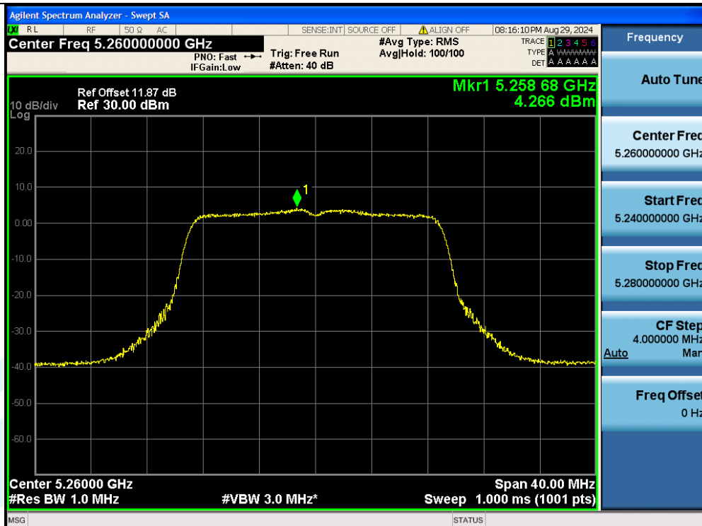
11AC20MIMO-Ant2-5260-PASS
