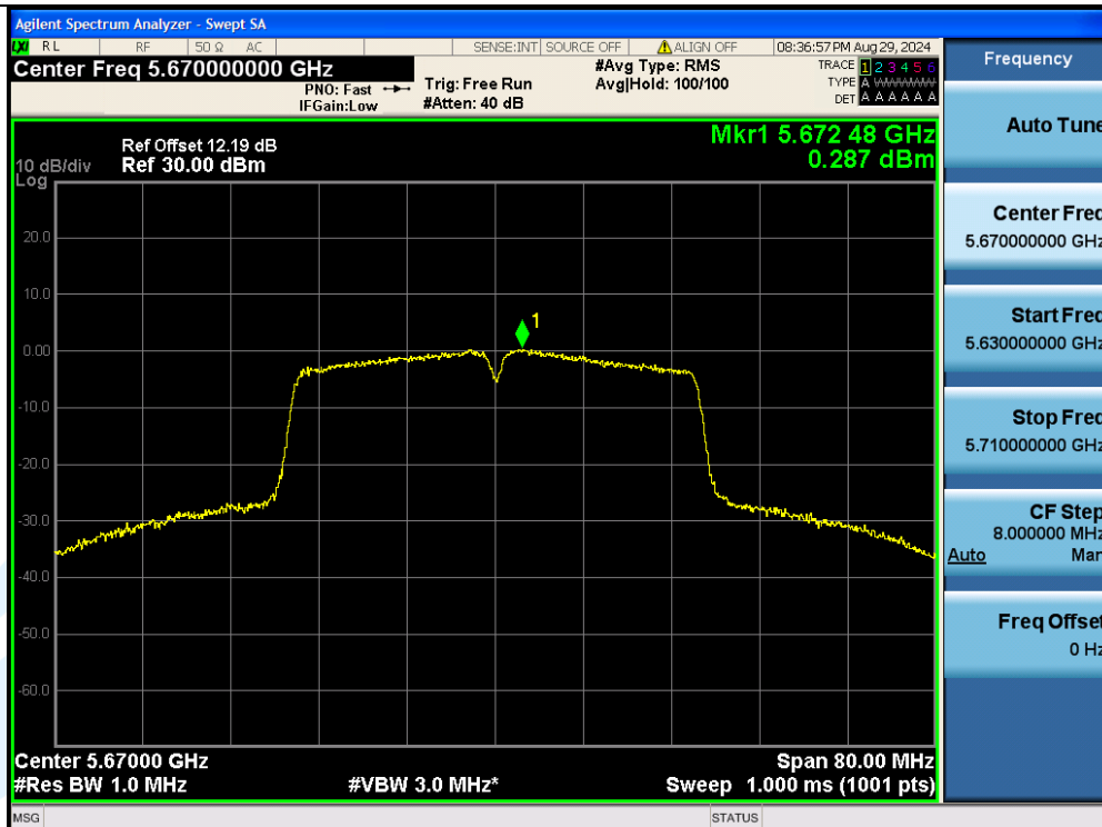
11AC40MIMO-Ant2-5670-PASS
