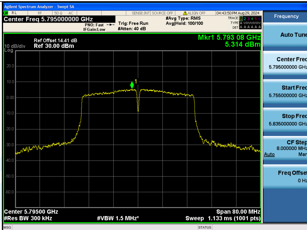
11N40MIMO-Ant2-5795-PASS
