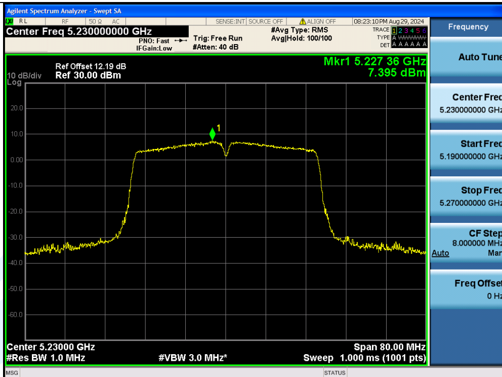
11AC40MIMO-Ant2-5230-PASS
