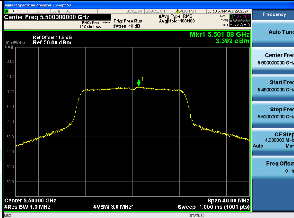
11AC20MIMO-Ant2-5500-PASS
