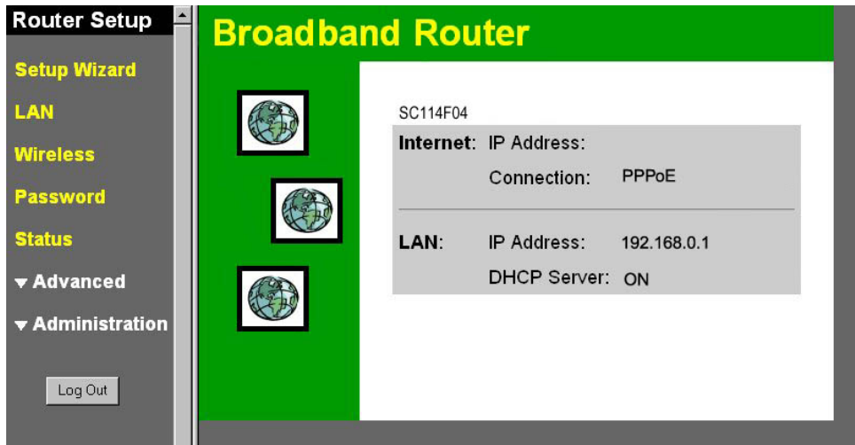
Figure 5: Home Screen
