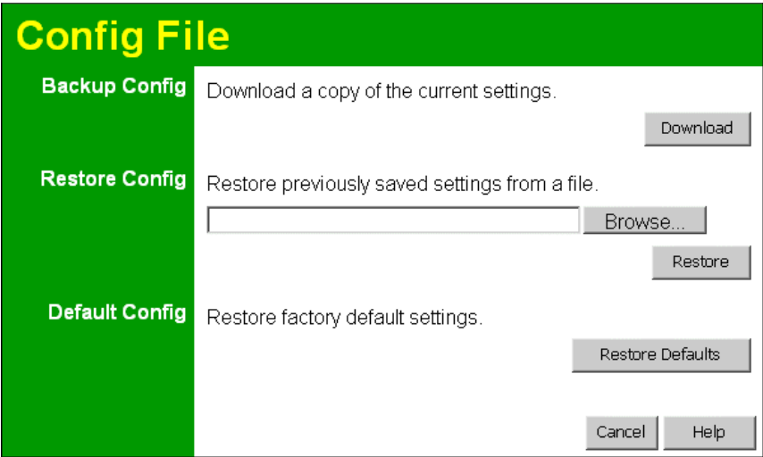
Figure 41: Config Screen
