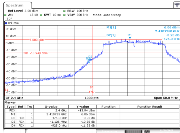
BE-NR, MIMO-B, 802.11n20-HT8 Ch1
