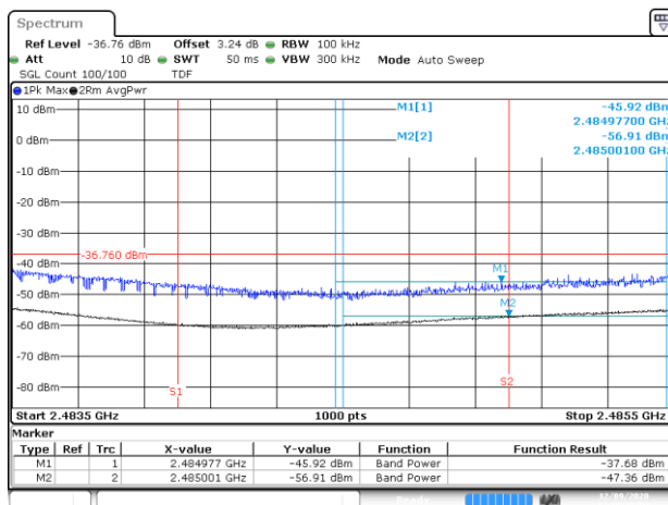
BE-R-HIGH-2MHz, SISO-B, 802.11ax40-HE0, Ch13
