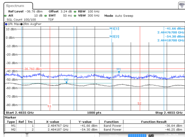
BE-R-HIGH-2MHz, MIMO-B, 802.11n20-HT8, Ch11
