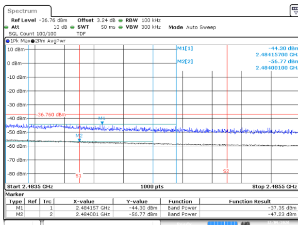
BE-R-HIGH-2MHz, SISO-B, 802.11ax40-HE0, Ch12
