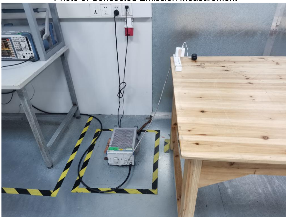
FCC ID: 2AJQ7TUNESMITH Photo of Conducted Emission Measurement
