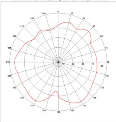
Far-field Power Distribution(H+V) on X-Z Plane Plot Peak Gain(H+V)= 1.33 dBi; Plot AvgGain(H+V)= -3.83dBi @2.44000 GHz
