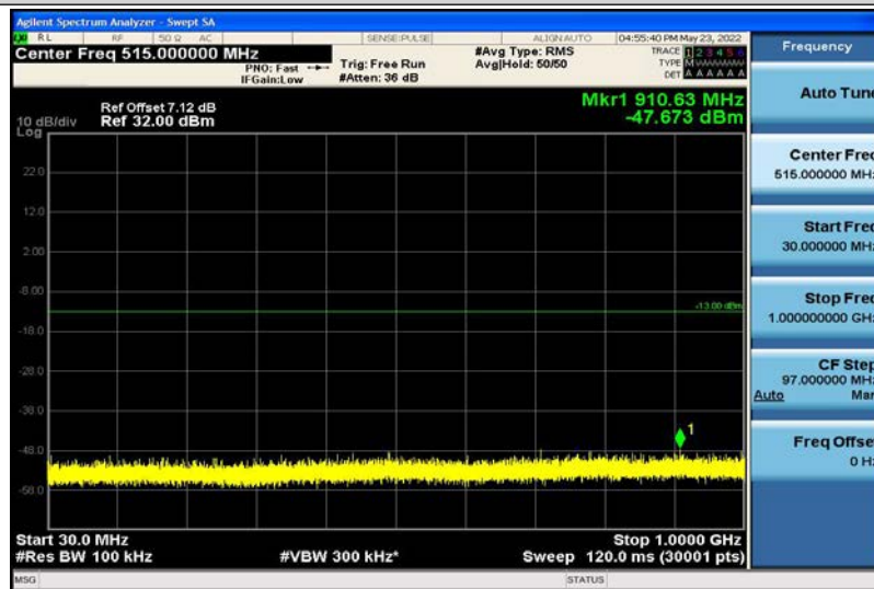
Band2-3MHz-16QAM-18615-1RB#0-30~1000MHz
