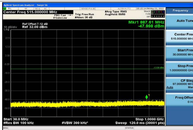
Band2-5MHz-16QAM-18900-1RB#0-30~1000MHz
