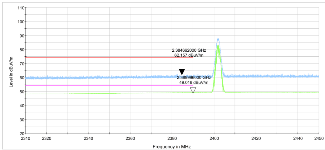
Fig.17. Frequency Band Edges: 8DPSK, Channel 0, 2.31 GHz - 2.45GHz
