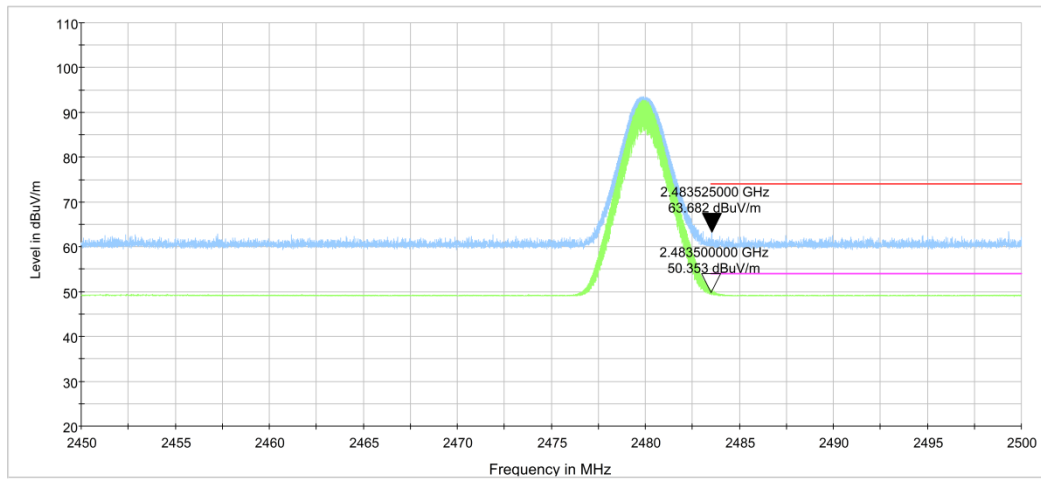
Fig.14. Frequency Band Edges: GFSK, Channel 78, Hopping Off, ch11, 2.45 GHz - 2.50GHz
