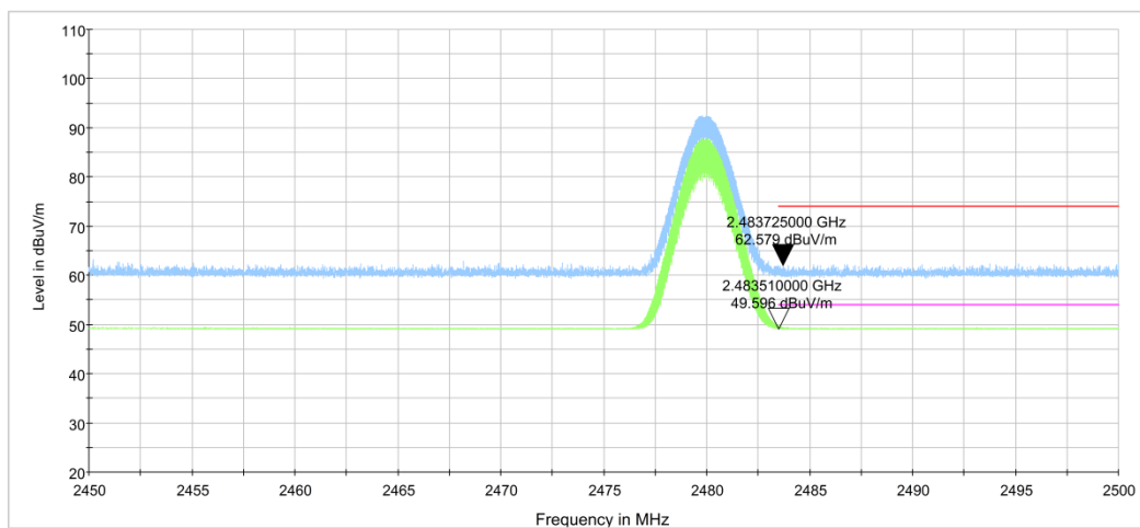
Fig.16. Frequency Band Edges: \pi/4 DQPSK, Channel 78, Hopping Off, 2.45 GHz - 2.50GHz
