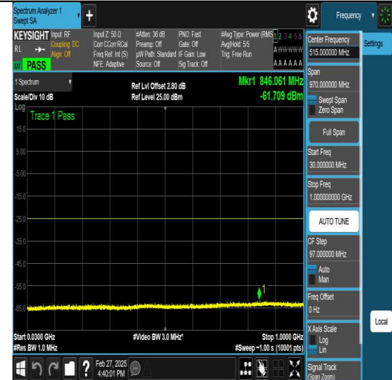
NTVN-N7-PC3-15-20-H-DFT-QPSK-Edge_1RB_Left-Ant1-
