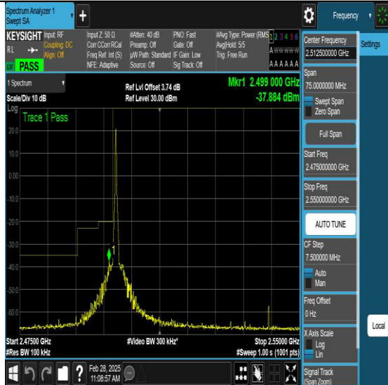
NTNV-N7-PC3-15-50-L-DFT-QPSK-Edge_1RB_Left-Ant1- PASS
