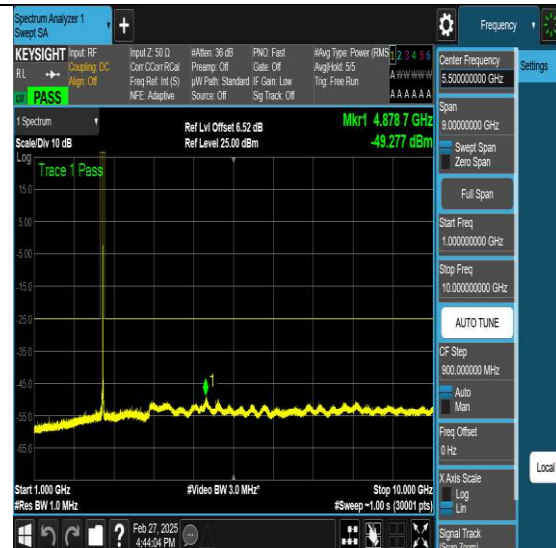
NTV-N7-PC3-15-25-H-DFT-QPSK-Edge_1RB_Left-Ant1- PASS
