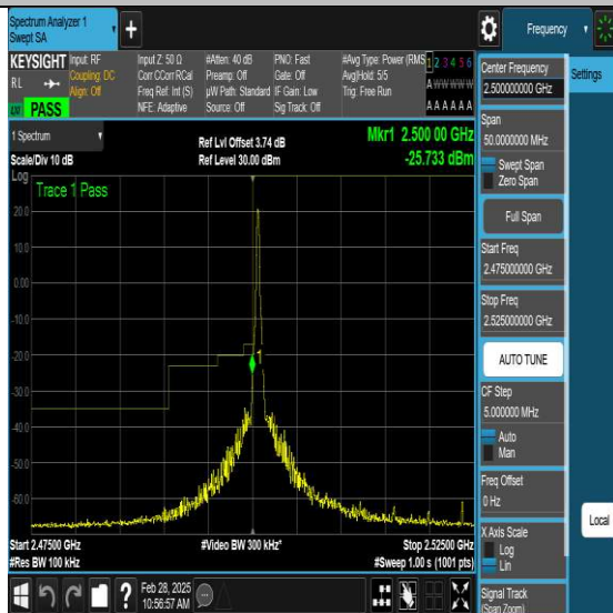
NTN-N7-PC3-15-25-L-DFT-QPSK-Edge_1RB_Left-Ant1-
