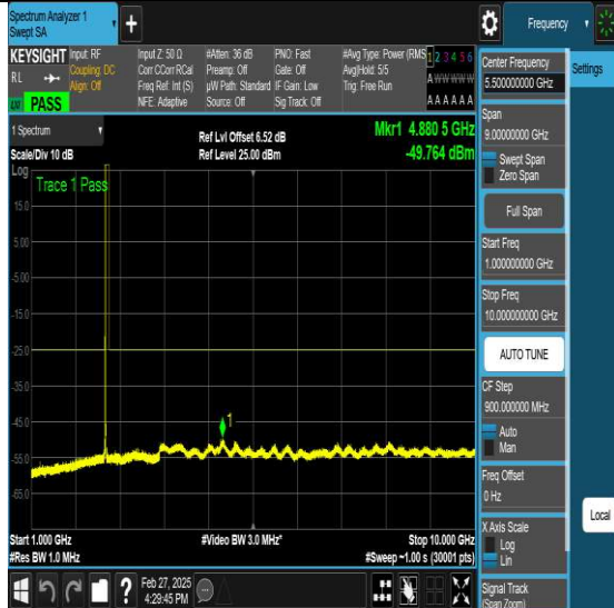
NTNV-N7-PC3-15-10-L-DFT-QPSK-Edge_1RB_Left-Ant1-PASS
