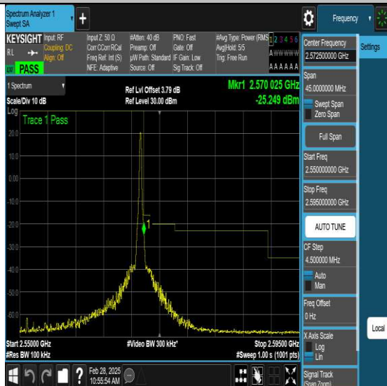
NTN-N7-PC3-15-20-H-DFT-QPSK-Edge_1RB_Right-Ant1-PASS
