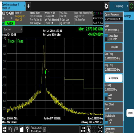
NTNV-N7-PC3-15-10-H-DFT-QPSK-Edge_1RB_Right-Ant1-PASS
