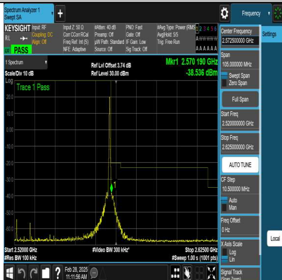
NTNV-N7-PC3-15-50-L-DFT-QPSK-Outer_Full-Ant1-PASS
