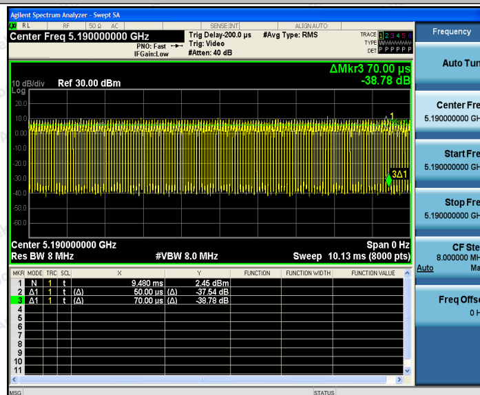
11AC40SISO_Ant2_5190
