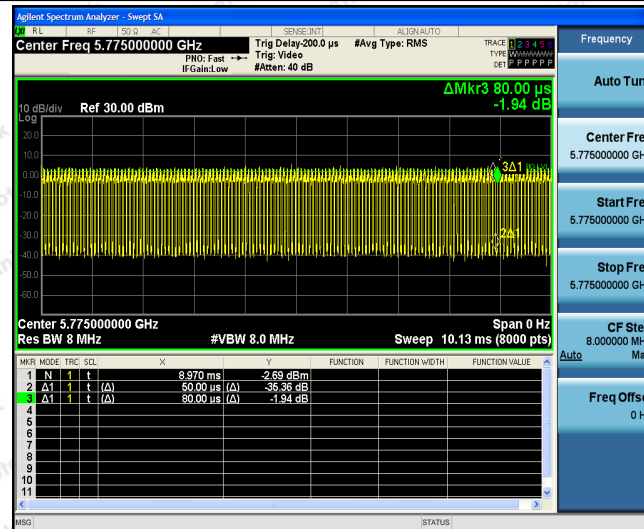
11AC80SISO_Ant2_5775
