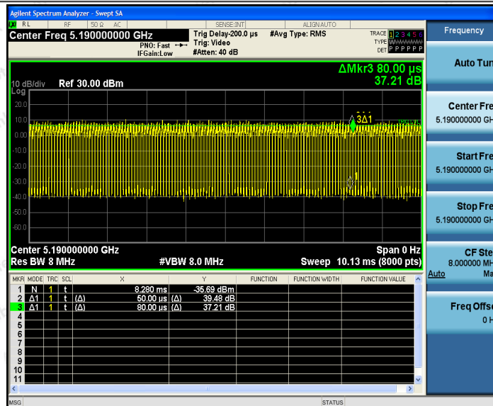
11N40SISO_Ant2_5190
