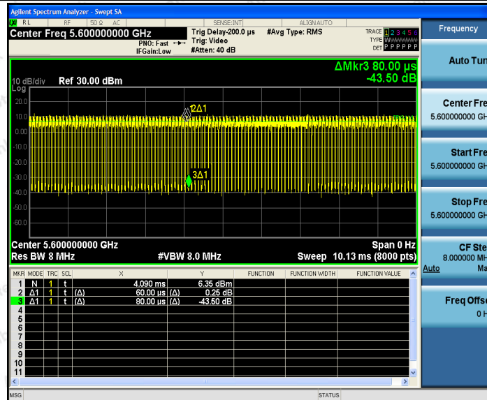
11AC20SISO_Ant2_5600
