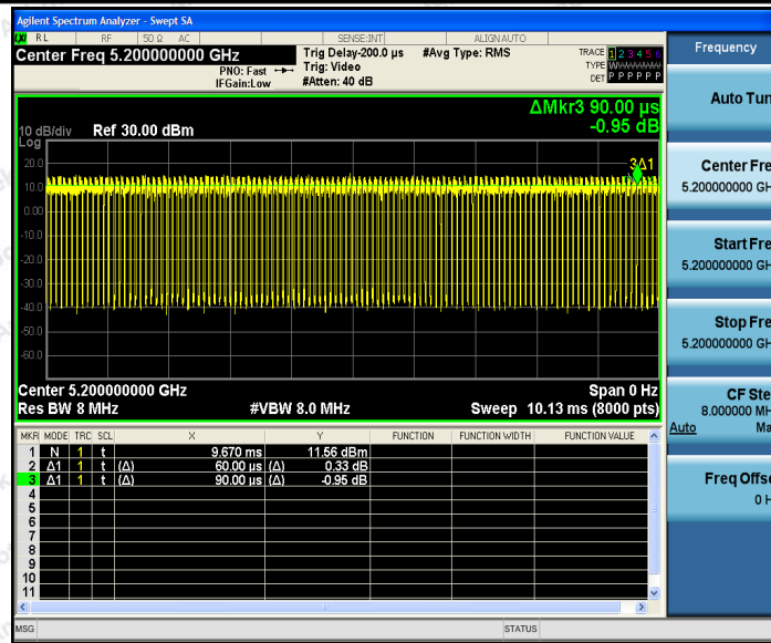
11AC20SISO_Ant2_5200
