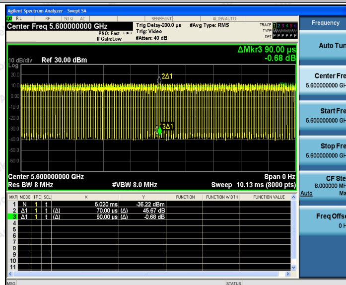
11AC20SISO_Ant2_5600
