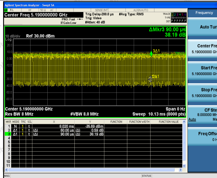
11AC40SISO_Ant2_5190
