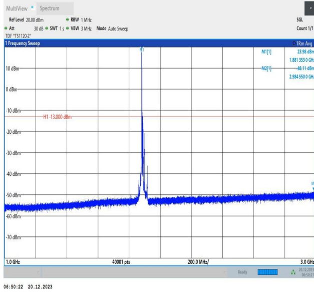
2-2-10MHz-20MHz-16QAM-16QAM-18956-19100-1RB#0-0RB #0-1000~3000MHz-PASS
