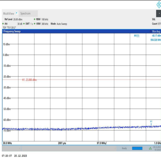
2-2-10MHz-20MHz-16QAM-16QAM-18956-19100-50RB#0-10 ORB#0-30~1000MHz-PASS
