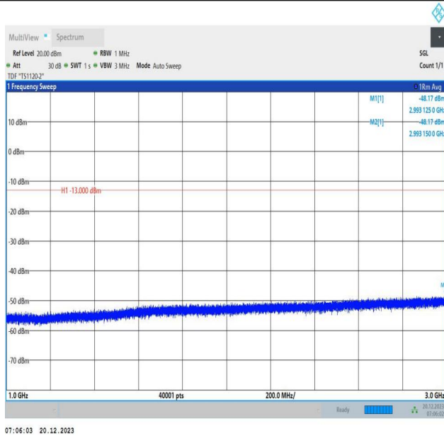
2-2-10MHz-20MHz-64QAM-64QAM-18956-19100-1RB#49-0R B#0-1000~3000MHz-PASS
