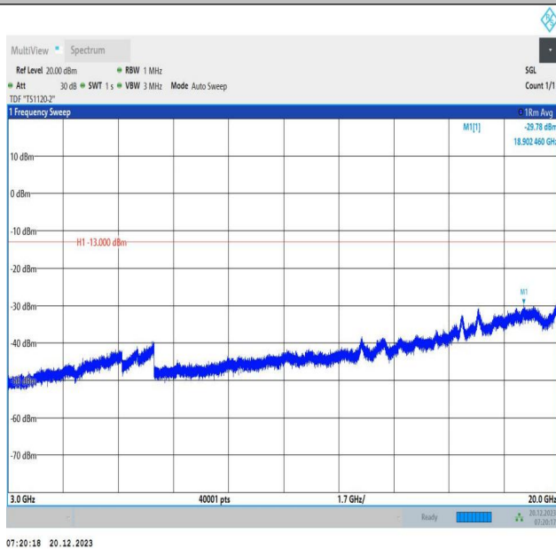
2-2-10MHz-20MHz-16QAM-16QAM-18956-19100-50RB#0-10 ORB#0-3000~20000MHz-PASS
