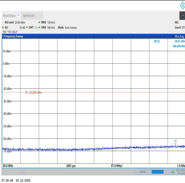
2-2-20MHz-10MHz-64QAM-64QAM-18700-18844-1RB#0-1RB #49-30~1000MHz-PASS
