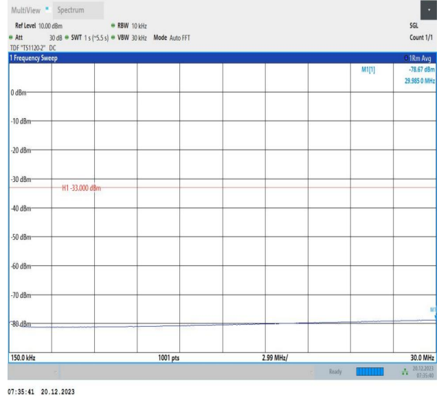
2-2-20MHz-10MHz-64QAM-64QAM-18700-18844-1RB#0-1RB #49-0.15~30MHz-PASS
