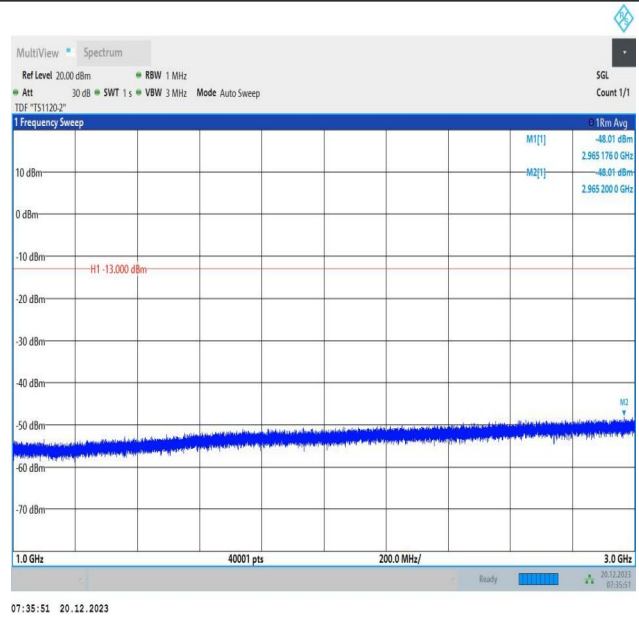
2-2-20MHz-10MHz-64QAM-64QAM-18700-18844-1RB#0-1RB #49-1000~3000MHz-PASS
