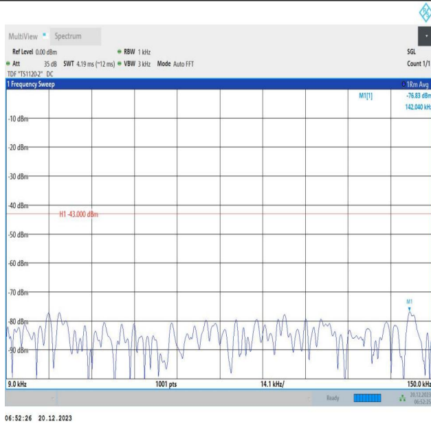
2-2-10MHz-20MHz-64QAM-64QAM-18956-19100-1RB#0-0RB #0-0.009~0.15MHz-PASS
