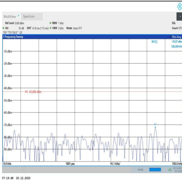
2-2-10MHz-20MHz-16QAM-16QAM-18956-19100-50RB#0-10 ORB#0-0.009~0.15MHz-PASS
