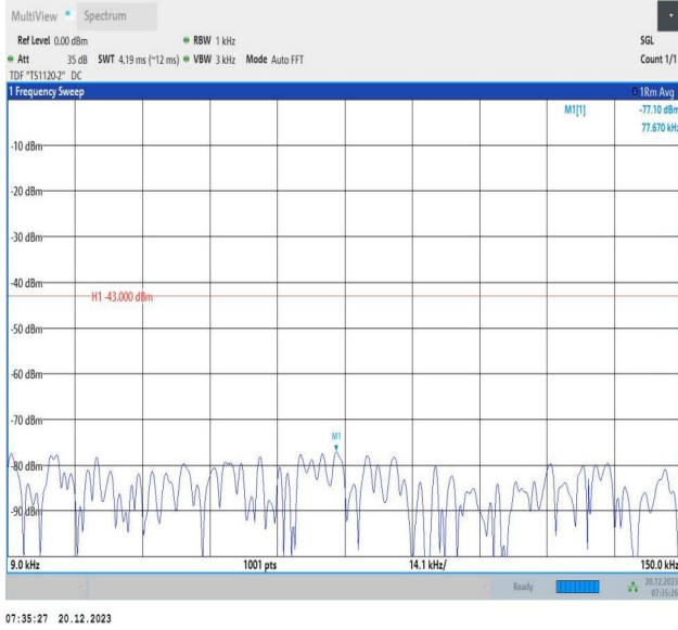
2-2-20MHz-10MHz-64QAM-64QAM-18700-18844-1RB#0-1RB #49-0.009~0.15MHz-PASS
