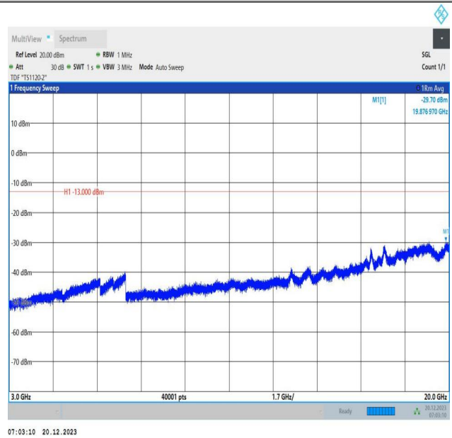
2-2-10MHz-20MHz-QPSK-QPSK-18956-19100-1RB#49-0RB# 0-3000~20000MHz-PASS
