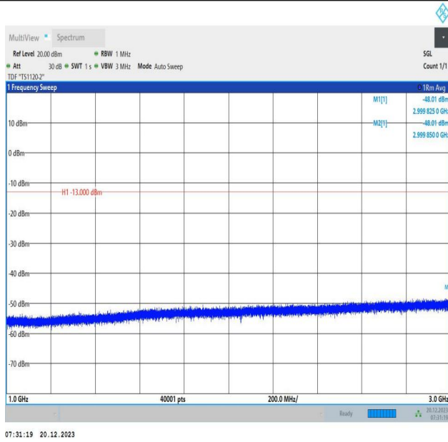
2-2-20MHz-10MHz-64QAM-64QAM-18700-18844-1RB#99-0R B#0-1000~3000MHz-PASS
