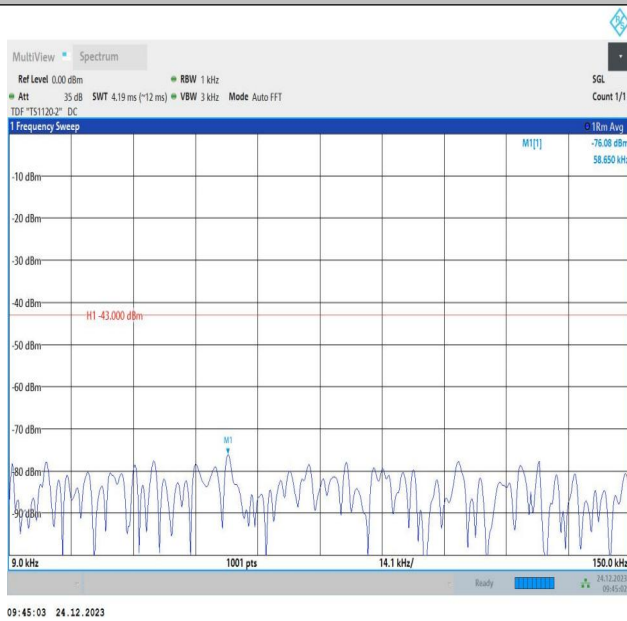
2-2-20MHz-10MHz-QPSK-QPSK-18700-18844-1RB#0-1RB#4 9-0.009~0.15MHz-PASS
