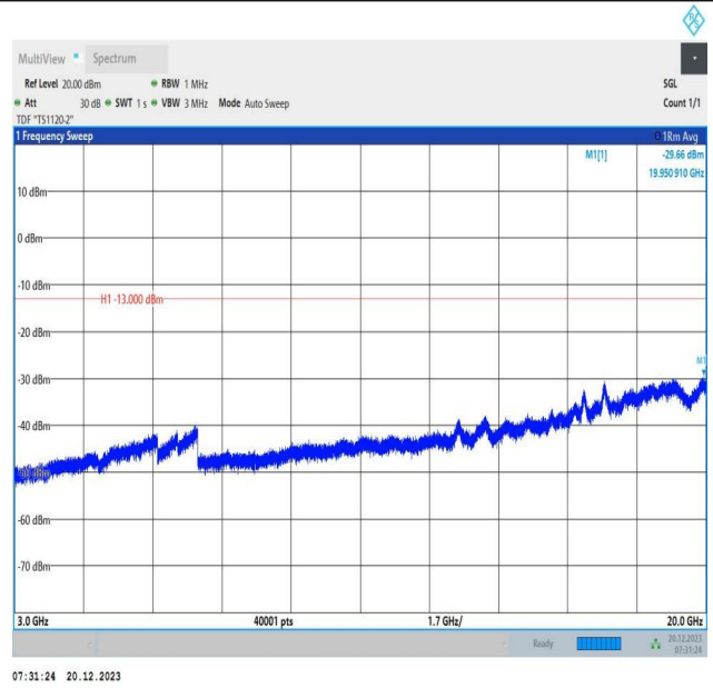
2-2-20MHz-10MHz-64QAM-64QAM-18700-18844-1RB#99-0R B#0-3000~20000MHz-PASS
