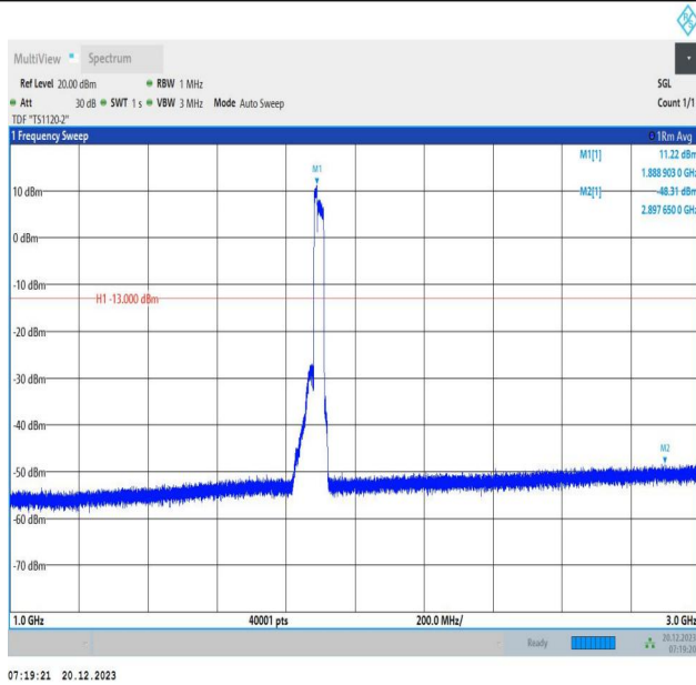
2-2-10MHz-20MHz-QPSK-QPSK-18956-19100-50RB#0-100R B#0-1000~3000MHz-PASS
