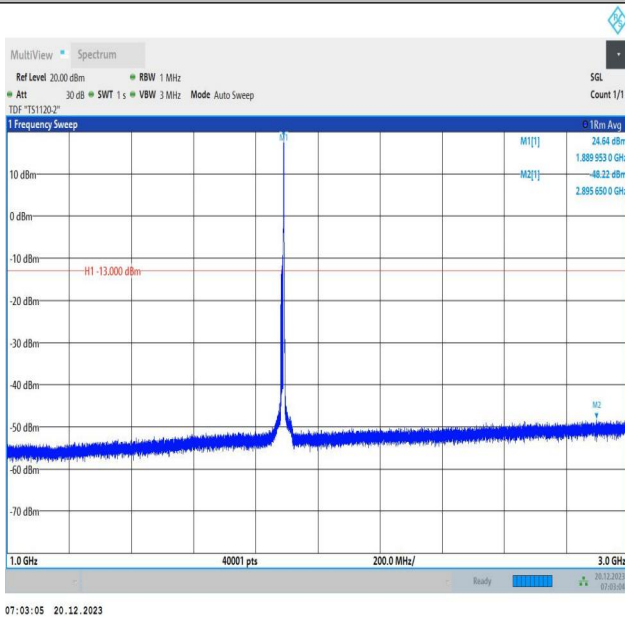
2-2-10MHz-20MHz-QPSK-QPSK-18956-19100-1RB#49-0RB# 0-1000~3000MHz-PASS
