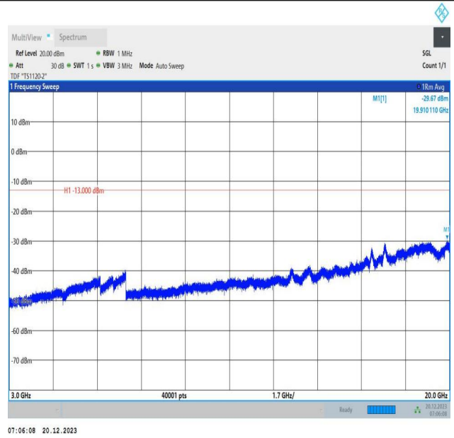
2-2-10MHz-20MHz-64QAM-64QAM-18956-19100-1RB#49-0R B#0-3000~20000MHz-PASS
