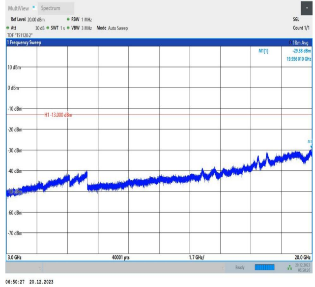
2-2-10MHz-20MHz-16QAM-16QAM-18956-19100-1RB#0-0RB #0-3000~20000MHz-PASS
