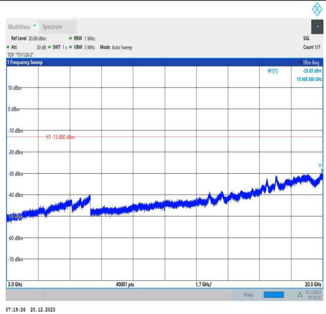
2-2-10MHz-20MHz-QPSK-QPSK-18956-19100-50RB#0-100R B#0-3000~20000MHz-PASS
