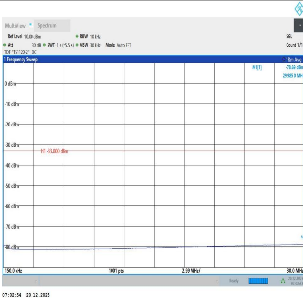
2-2-10MHz-20MHz-QPSK-QPSK-18956-19100-1RB#49-0RB# 0-0.15~30MHz-PASS
