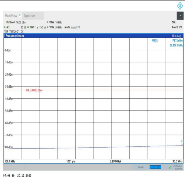
2-2-10MHz-20MHz-QPSK-QPSK-18956-19100-1RB#0-1RB#9 9-0.15~30MHz-PASS
