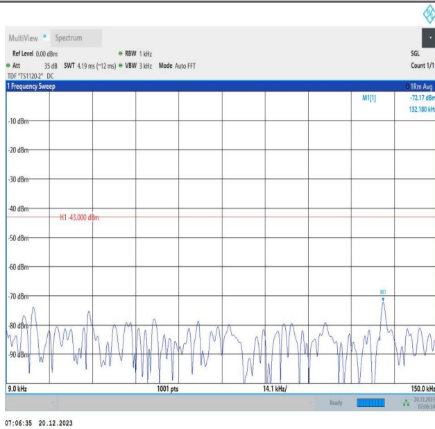
2-2-10MHz-20MHz-QPSK-QPSK-18956-19100-1RB#0-1RB#9 9-0.009~0.15MHz-PASS
