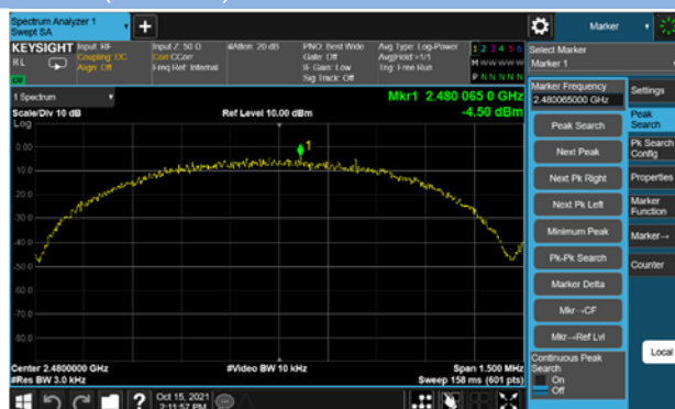
GFSK (BLE 1M) HIGH CHANNEL
