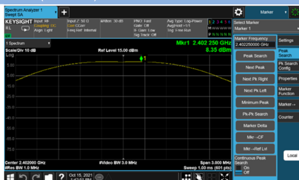
GFSK(BLE 1M ) LOW CHANNEL
