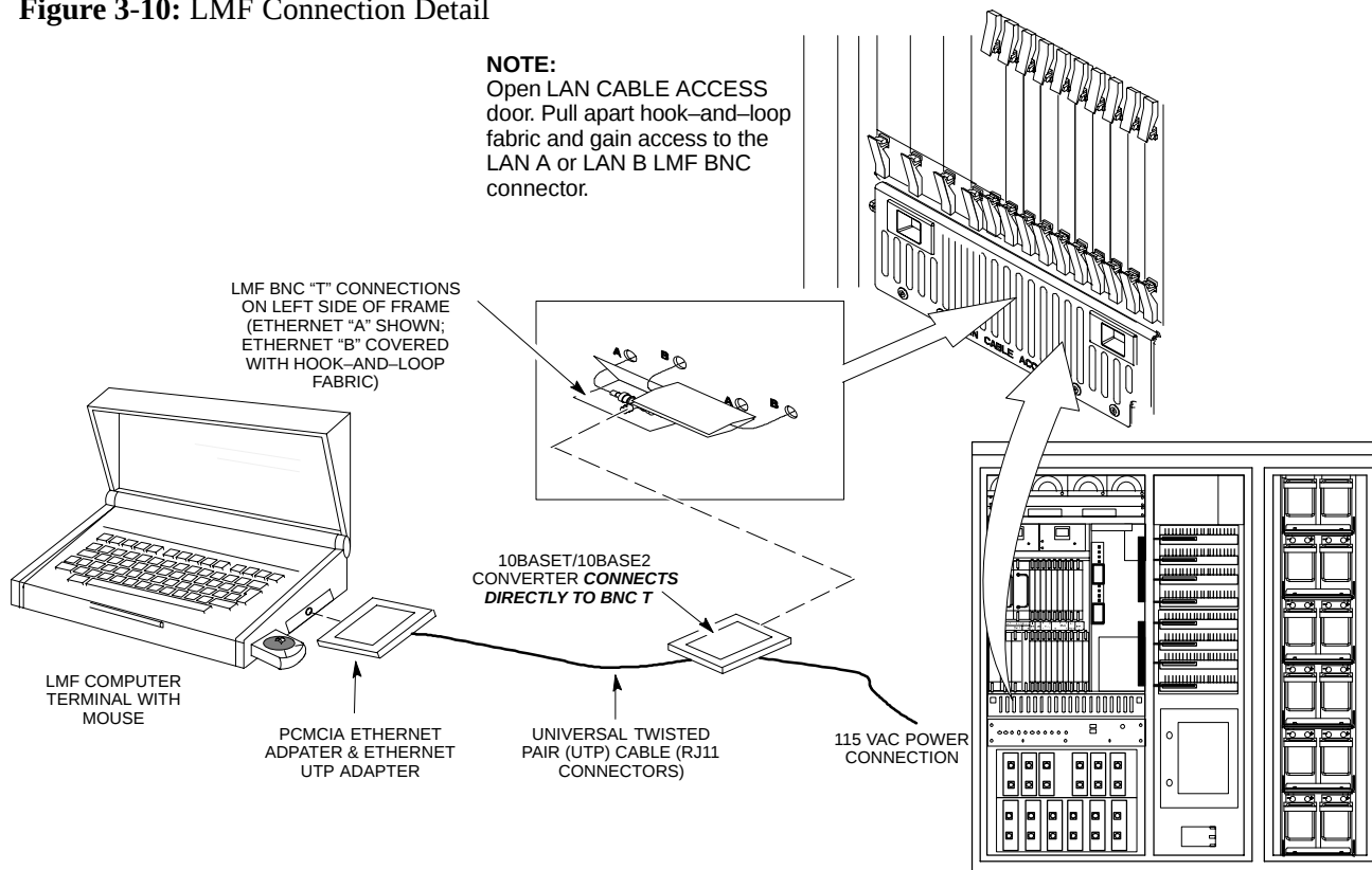
Figure 3-10: LMF Connection Detail
