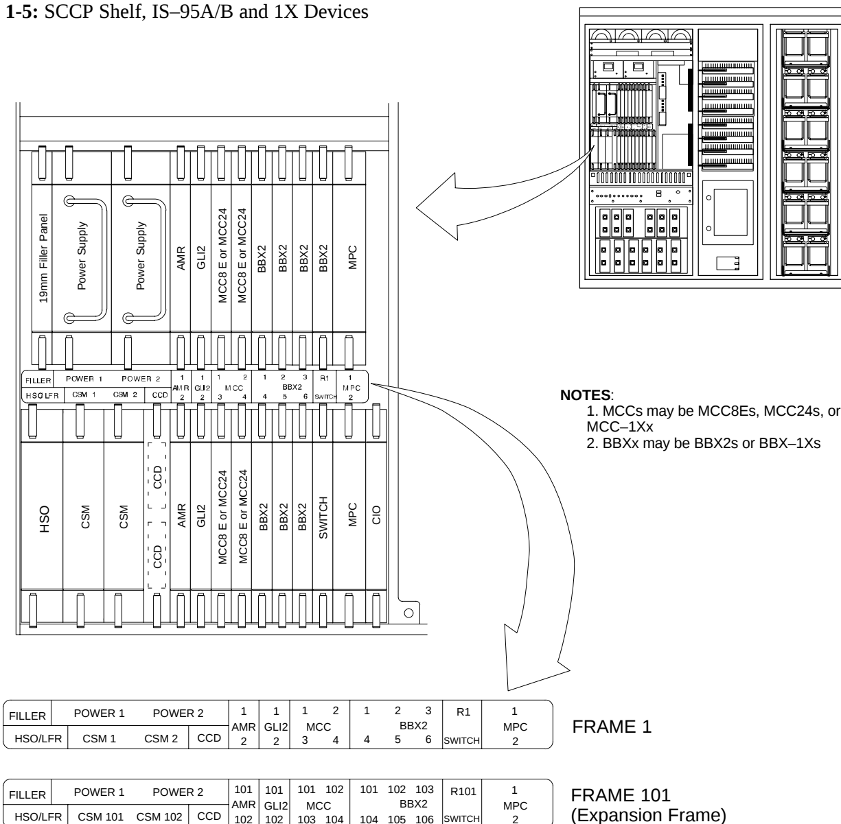
Figure 1-5: SCCP Shelf, IS-95A/B and 1X Devices
