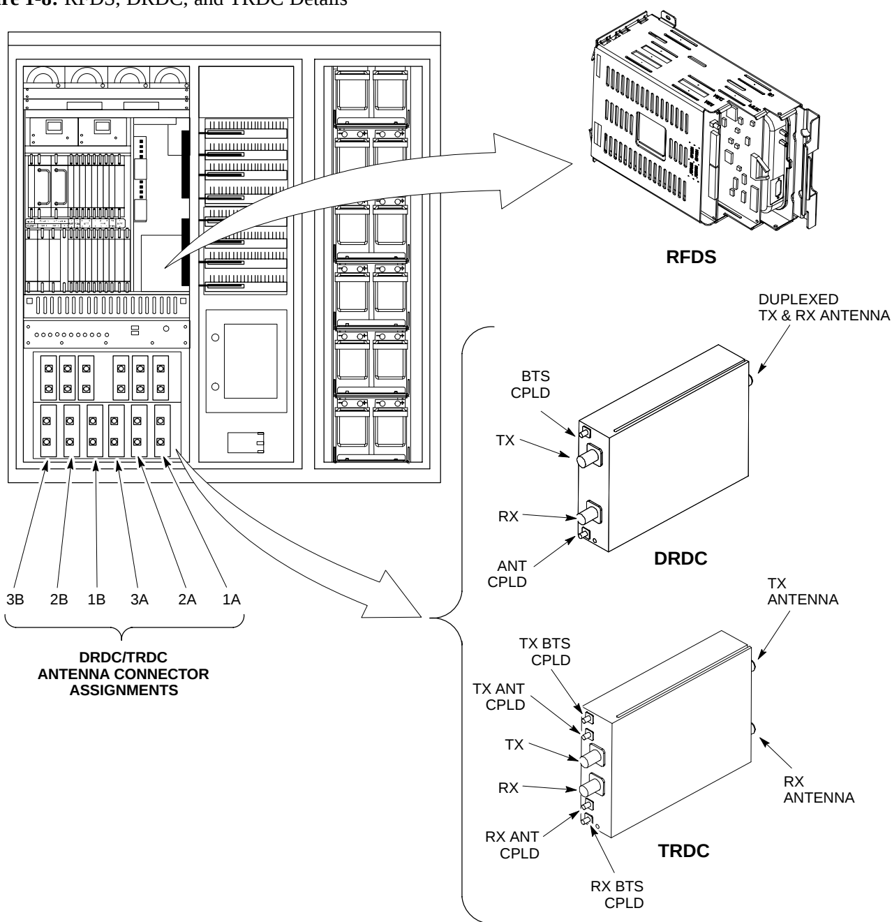
Figure 1-8: RFDS, DRDC, and TRDC Details
