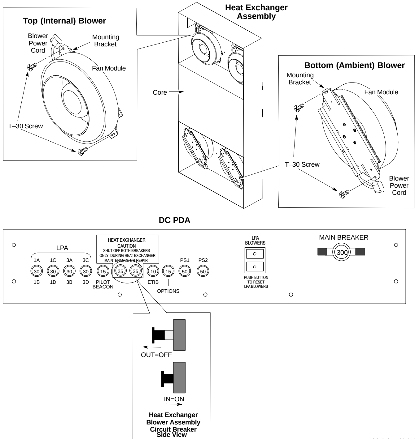
Figure 2-10: Heat Exchanger Blower Assembly and Circuit Breakers
