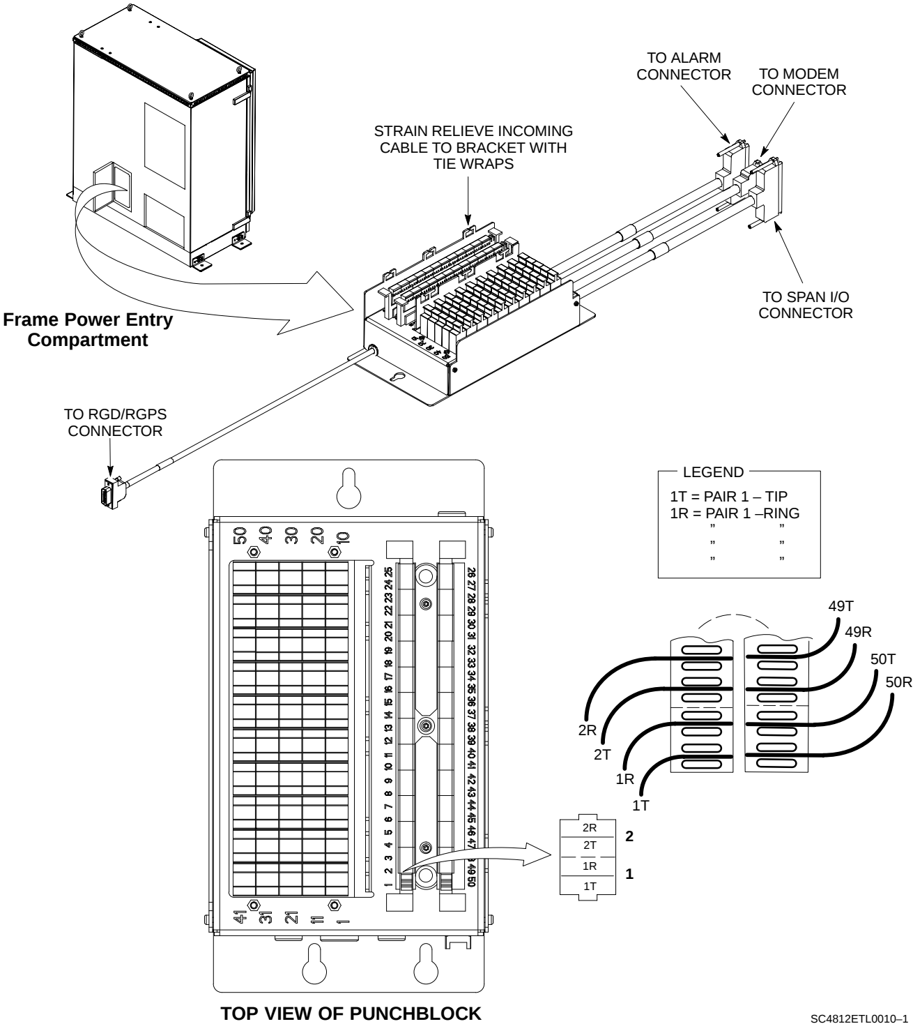
Figure 3-9: 50-Pair Punchblock
