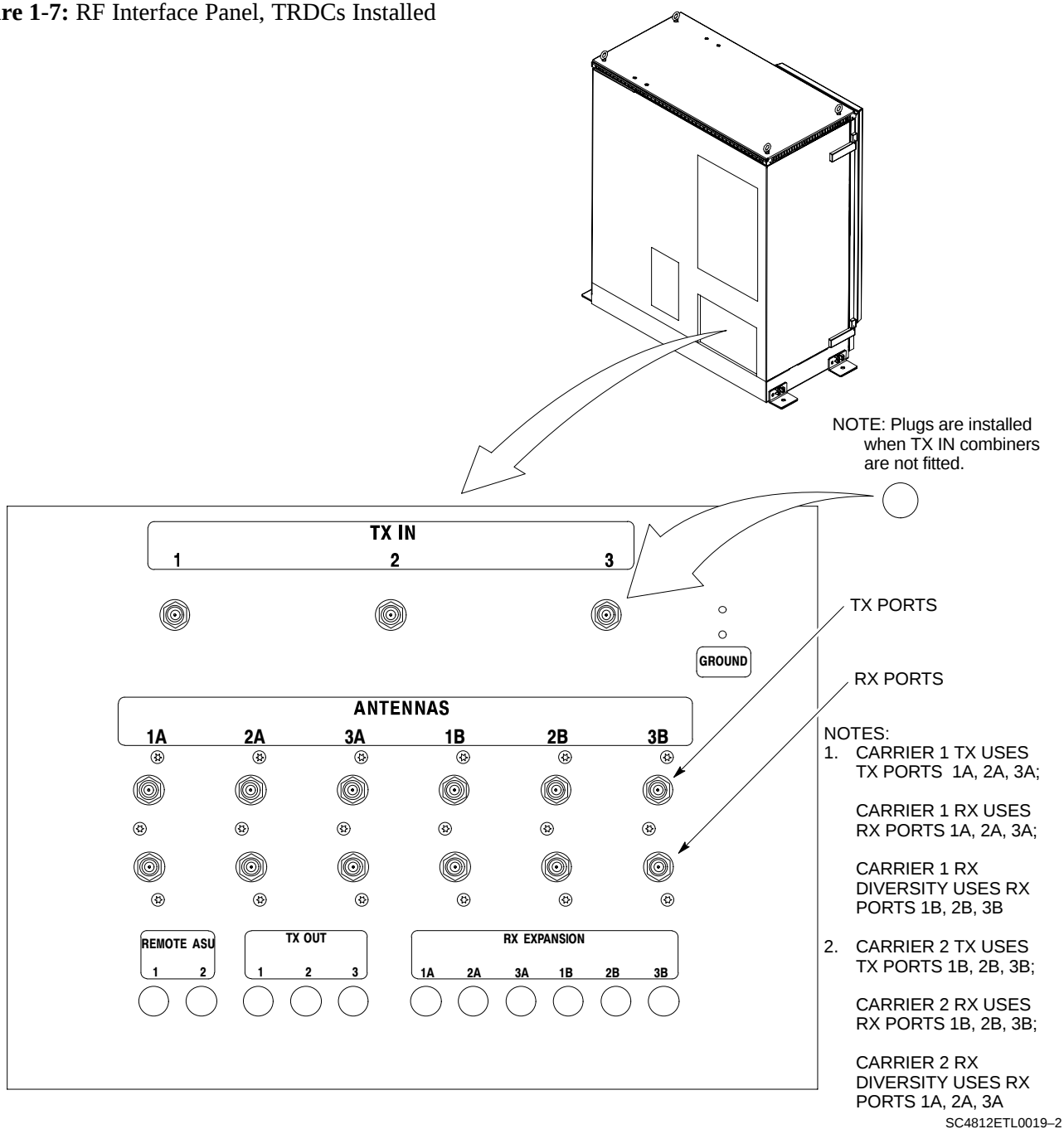
Figure 1-7: RF Interface Panel, TRDCs Installed
