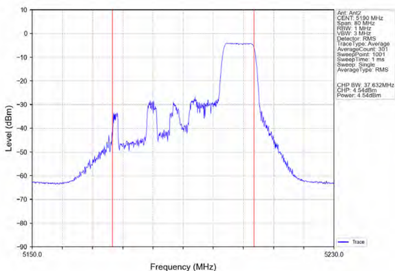
802.11ax(HE40) LCH 5190MHz RU106 Right Ant2 NTVN
