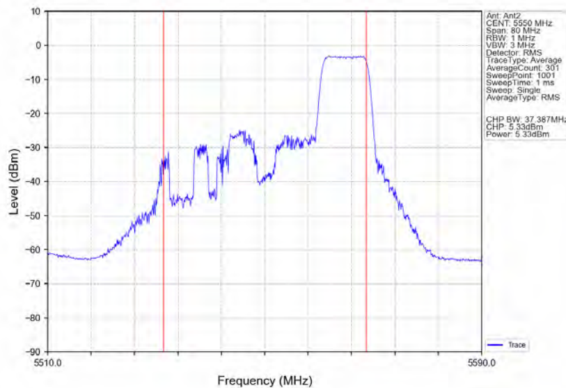
802.11ax(HE40) MCH_5550MHz RU106 Right Ant2 NTVN
