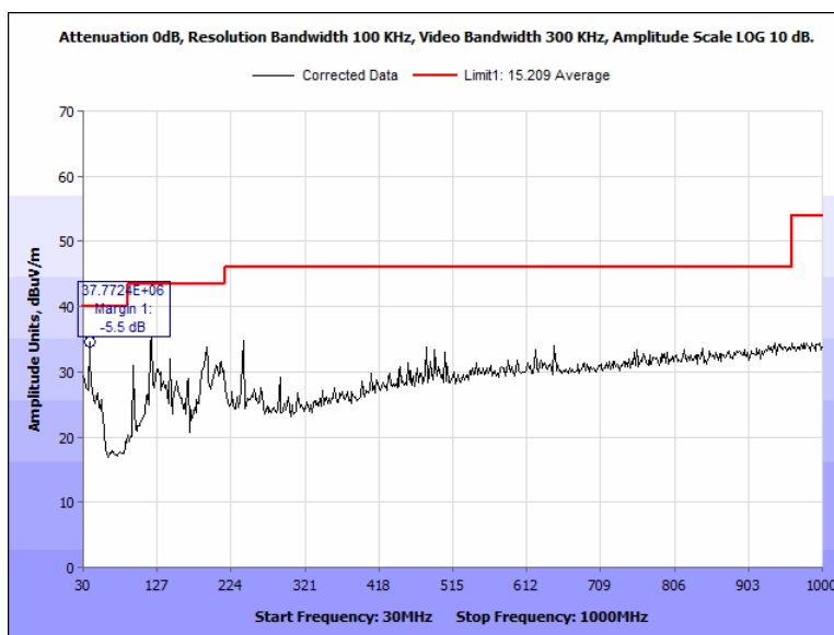
Figure 95: Radiated Spurious Emissions, Terminal, 2442 MHz, 30 MHz - 1000 MHz, Horizontal
