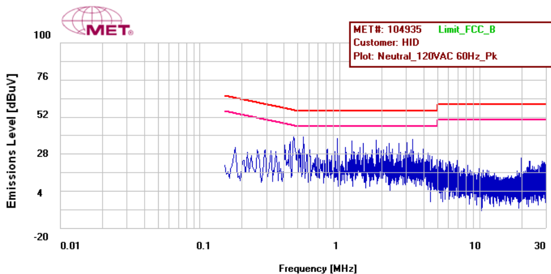
Figure 16: Conducted Emissions Limits, Terminal, Neutral Line, Prescan
