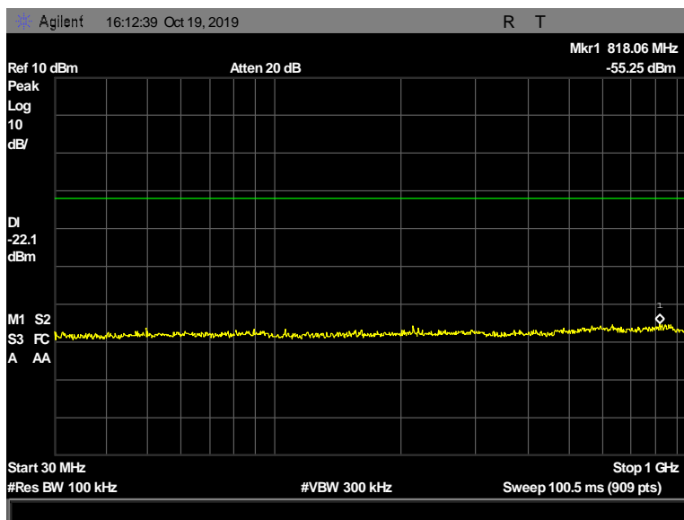
Figure 124: Conducted Spurious Emissions, Pigtail, 2402 MHz, 1 Mbps, 30 MHz - 1000 MHz
