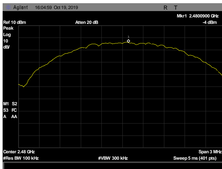
Figure 163: Peak Power Spectral Density, Pigtail, 2480 MHz, 2 Mbps, -4.000 dBm
