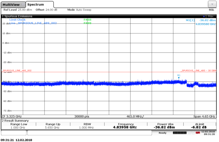
Figure 343 Spurious Emissions (1 GHz – 5.65 GHz) – 256QAM (5765.0/ 5785.0 MHz) (2 X 20MHz Channel BW)
