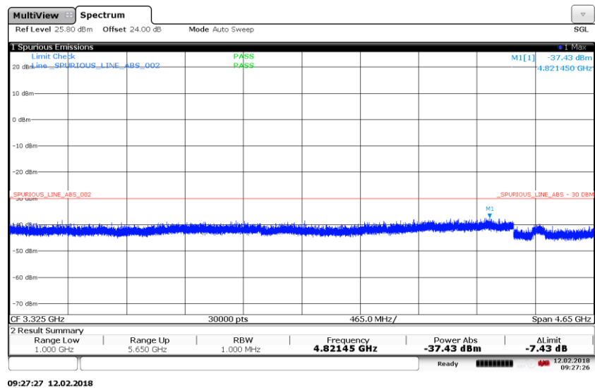
Figure 340 Spurious Emissions (1 GHz – 5.65 GHz) – QPSK (5765.0/ 5785.0 MHz) (2 X 20MHz Channel BW)
