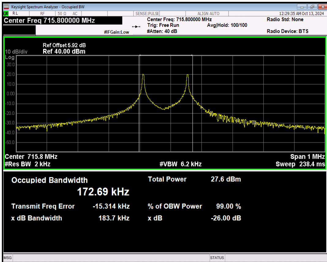
Band12 QPSK Channel=23178 nTones=1@0 Spacing=3.75kHz
