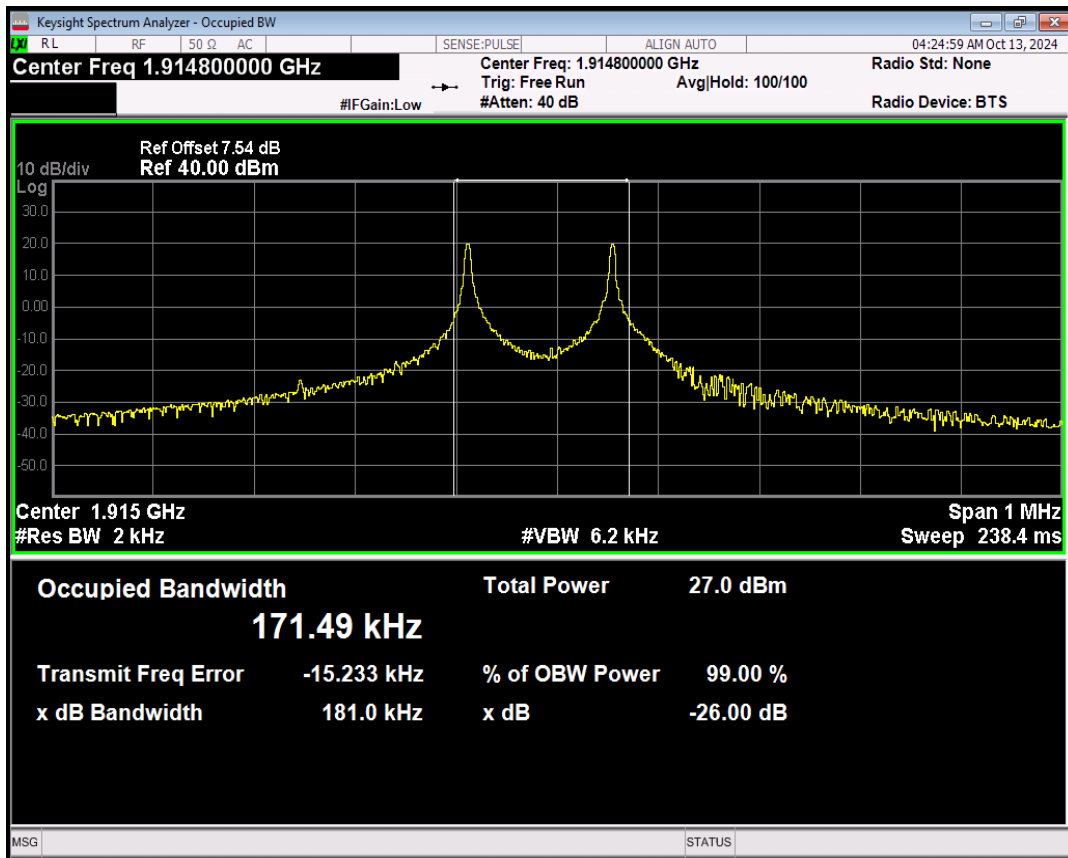
Band25 BPSK Channel=26688 nTones=1@0 Spacing=15kHz
