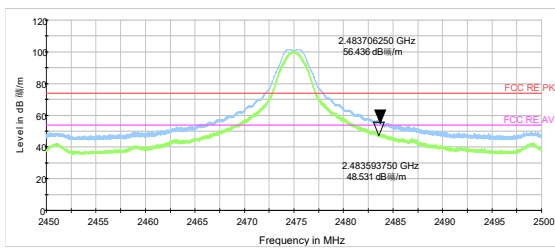
Zigbee-Channel 25: Peak & Average
