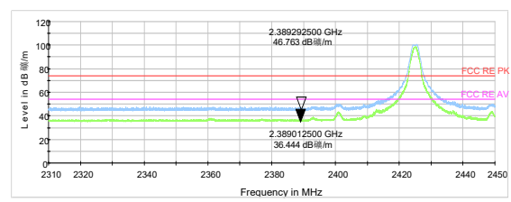
Zigbee-Channel 15: Peak & Average
