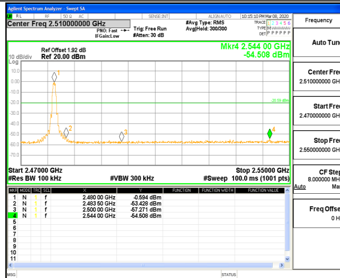
BLE_Ant1_High_2480
