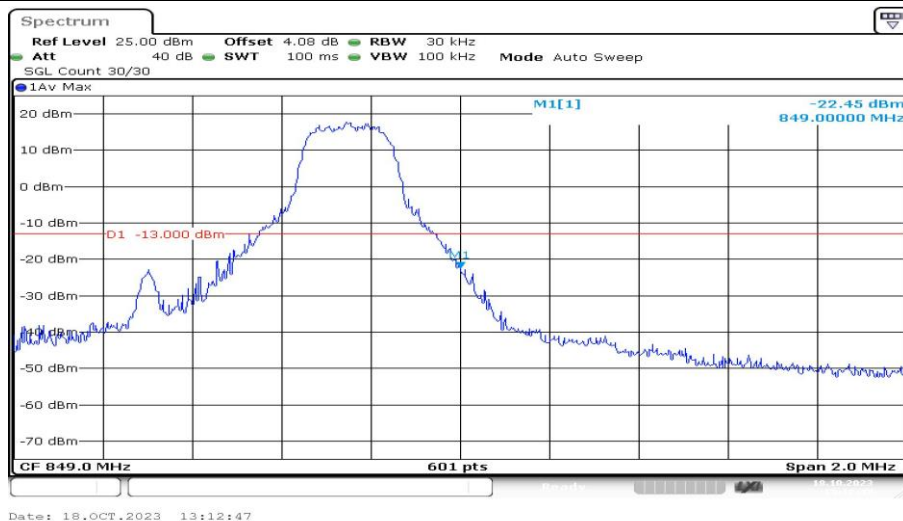
Band5-1.4MHz-QPSK-20643-1RB#5-PASS
