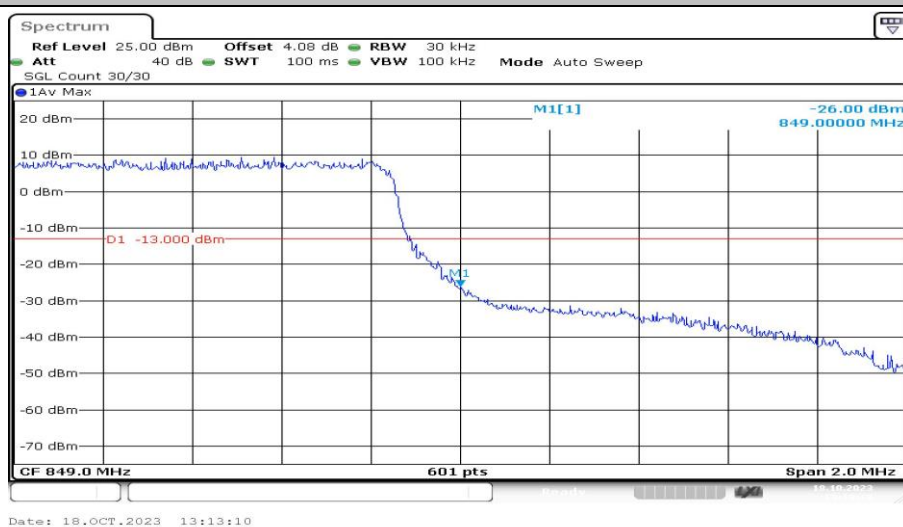
Band5-1.4MHz-QPSK-20643-6RB#0-PASS
