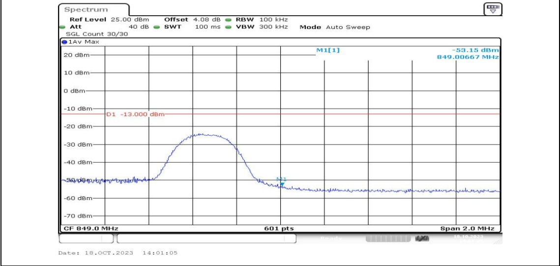
Band5-5MHz-16QAM-20625-1RB#0-PASS
