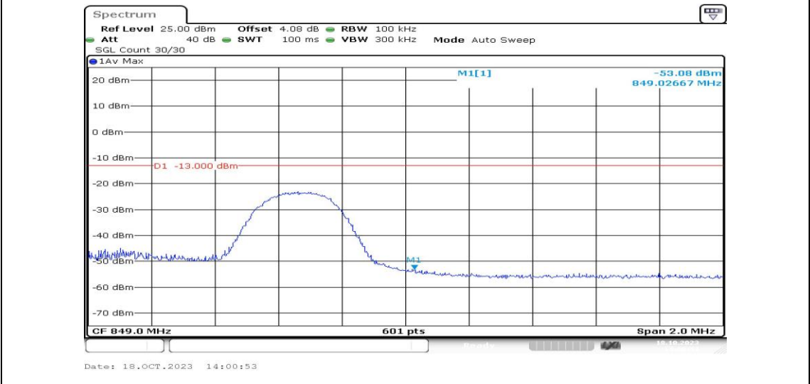
Band5-5MHz-QPSK-20625-1RB#0-PASS
