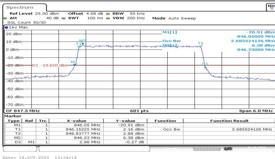
Band5-3MHz-16QAM-20635-15RB#0-PASS
