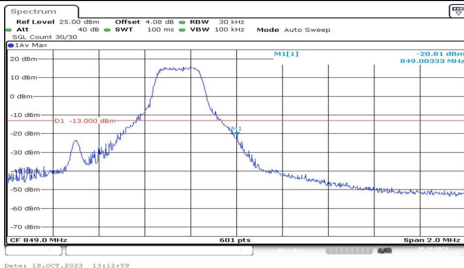
Band5-1.4MHz-16QAM-20643-1RB#5-PASS
