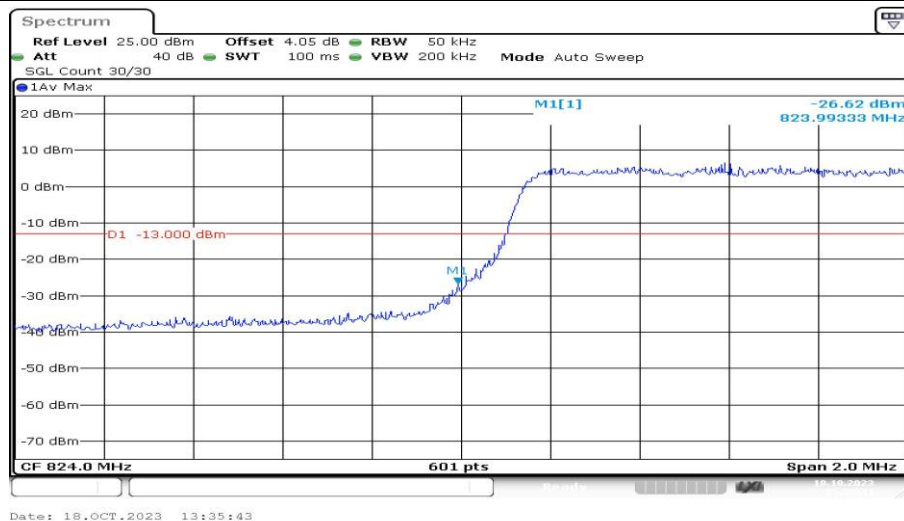
Band5-3MHz-16QAM-20415-15RB#0-PASS
