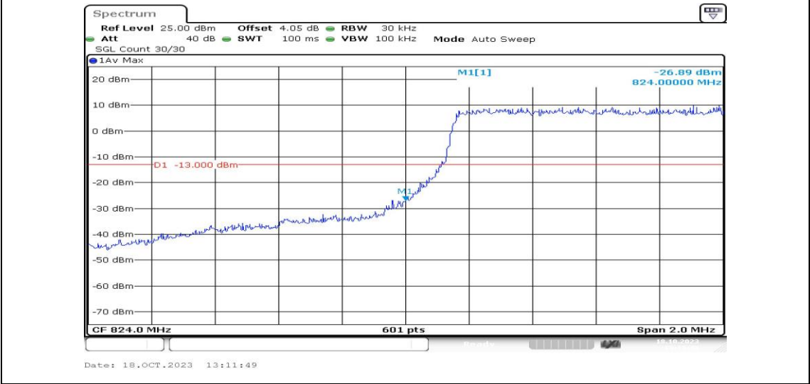
Band5-1.4MHz-QPSK-20407-6RB#0-PASS
