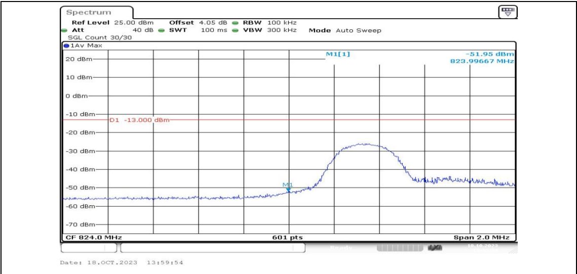
Band5-5MHz-QPSK-20425-1RB#24-PASS
