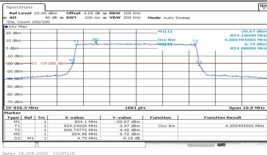
Band5-5MHz-16QAM-20425-25RB#0-PASS
