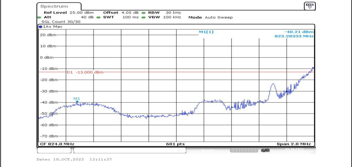
Band5-1.4MHz-16QAM-20407-1RB#5-PASS
