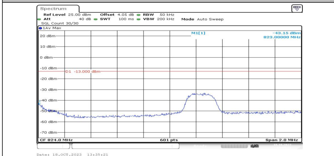
Band5-3MHz-16QAM-20415-1RB#14-PASS
