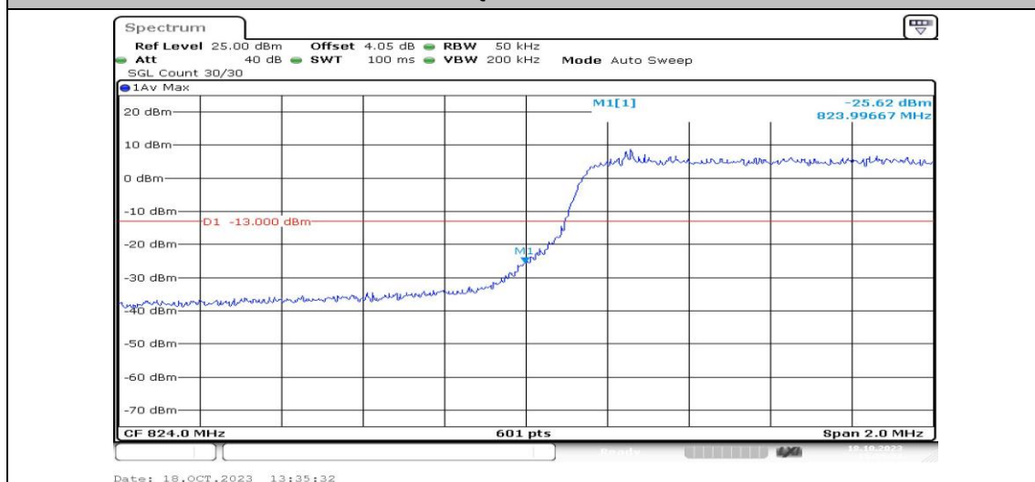
Band5-3MHz-QPSK-20415-15RB#0-PASS
