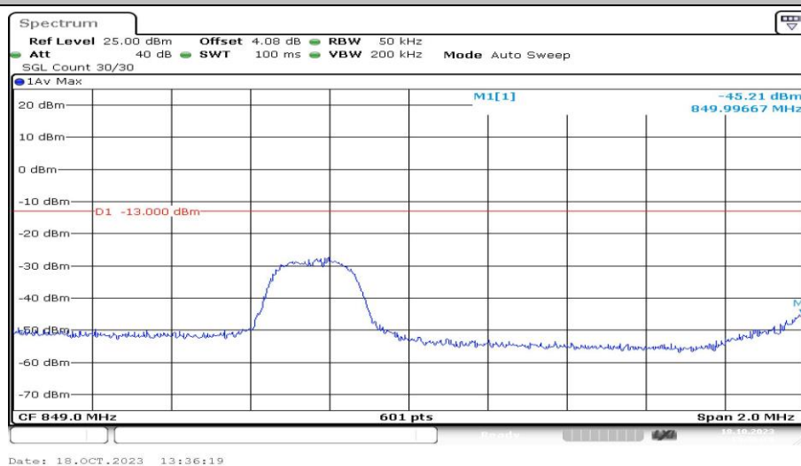
Band5-3MHz-16QAM-20635-1RB#0-PASS
