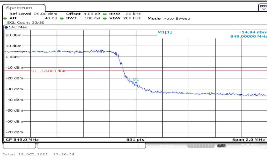
Band5-3MHz-QPSK-20635-15RB#0-PASS
