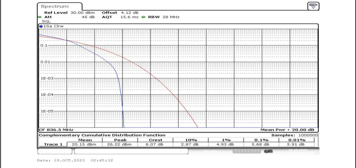
Band5-10MHz-16QAM-20525-25RB#0-PASS
