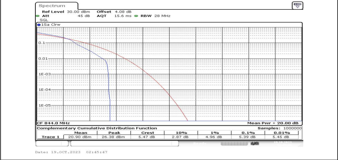
Band5-10MHz-16QAM-20600-1RB#0-PASS
