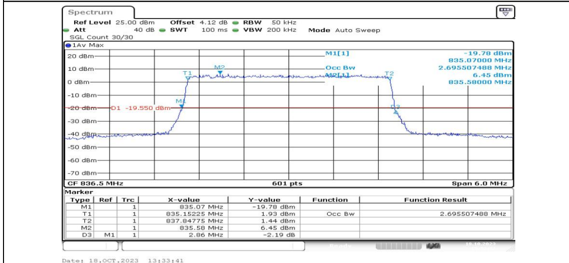
Band5-3MHz-16QAM-20525-15RB#0-PASS
