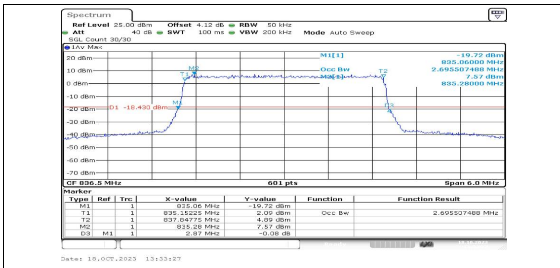
Band5-3MHz-QPSK-20525-15RB#0-PASS
