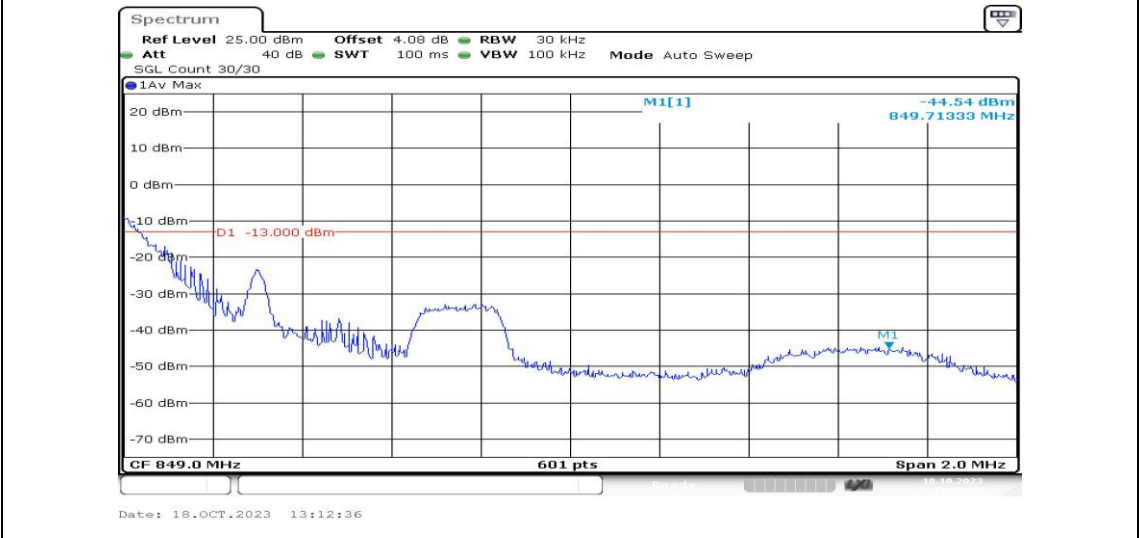
Band5-1.4MHz-16QAM-20643-1RB#0-PASS
