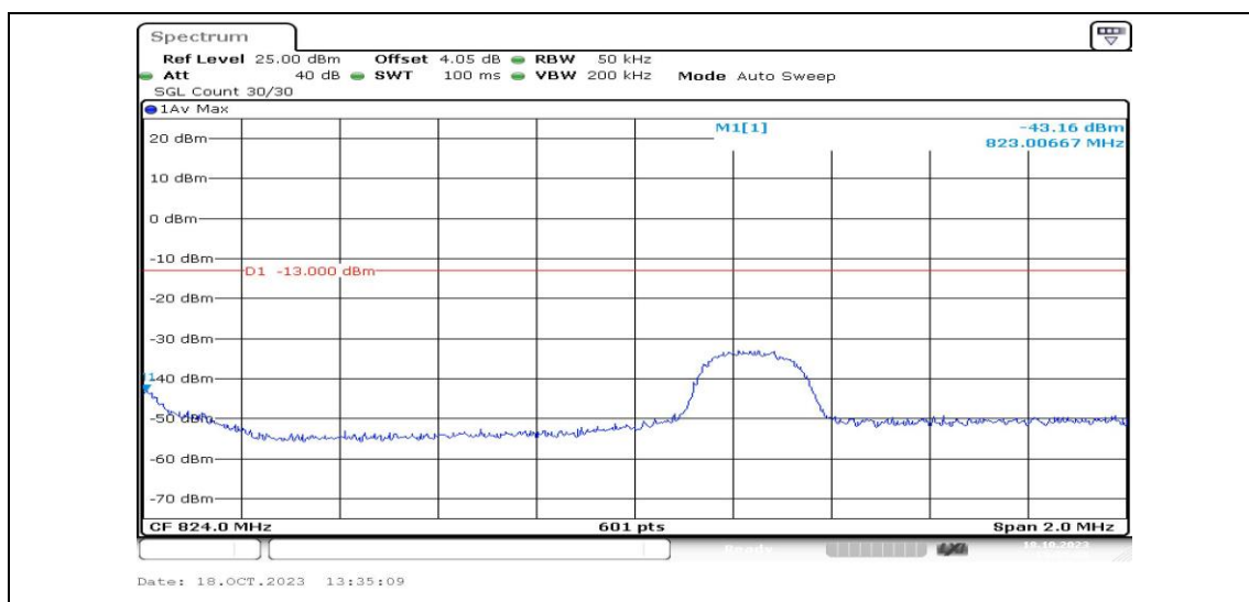
Band5-3MHz-QPSK-20415-1RB#14-PASS
