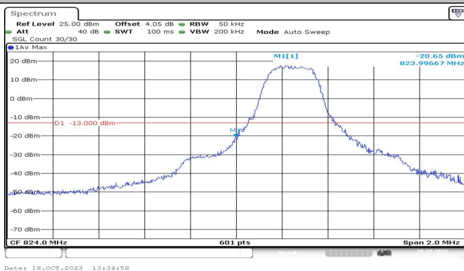
Band5-3MHz-16QAM-20415-1RB#0-PASS
