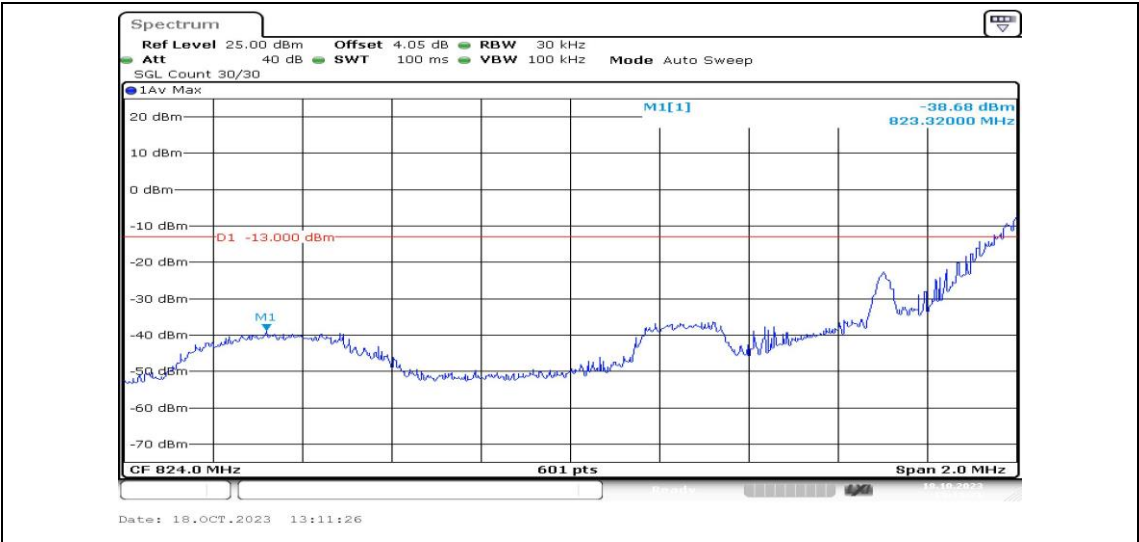
Band5-1.4MHz-QPSK-20407-1RB#5-PASS
