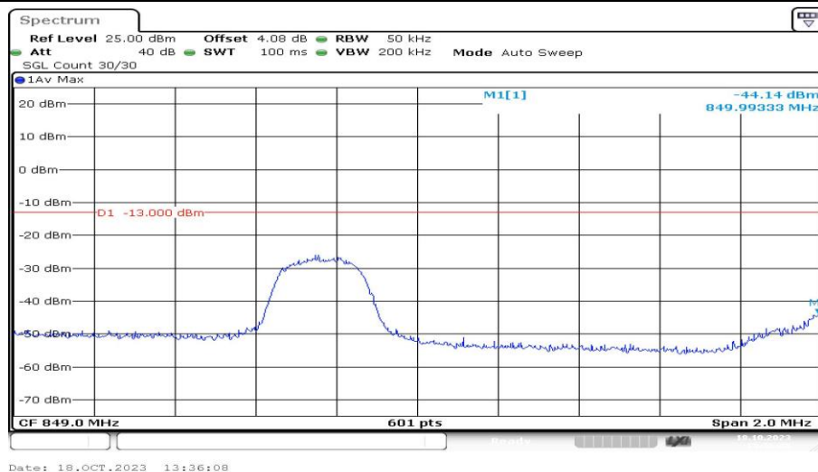
Band5-3MHz-QPSK-20635-1RB#0-PASS
