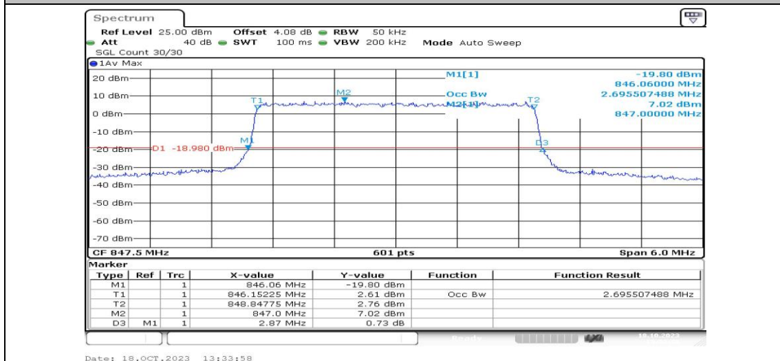
Band5-3MHz-QPSK-20635-15RB#0-PASS
