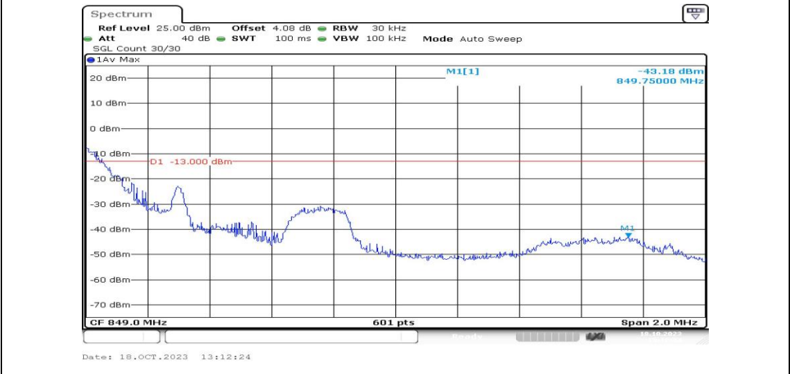
Band5-1.4MHz-QPSK-20643-1RB#0-PASS
