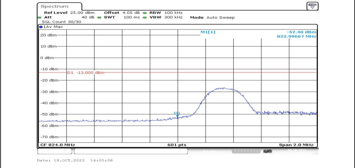
Band5-5MHz-16QAM-20425-1RB#24-PASS
