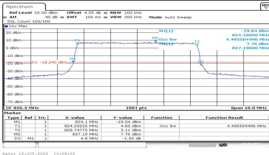
Band5-5MHz-QPSK-20425-25RB#0-PASS
