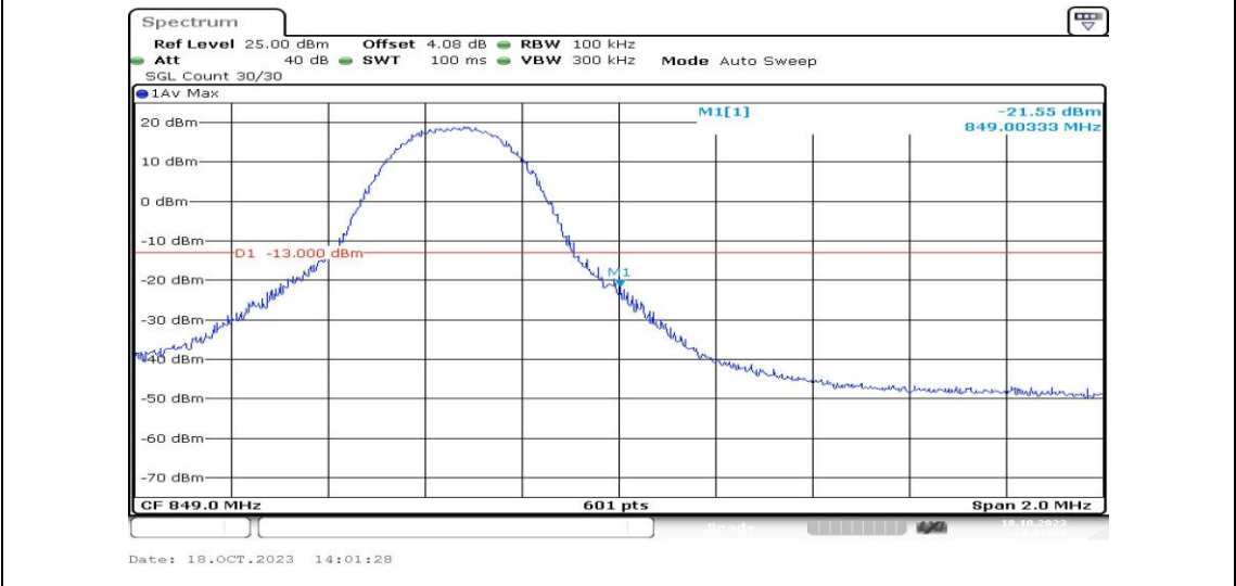
Band5-5MHz-16QAM-20625-1RB#24-PASS
