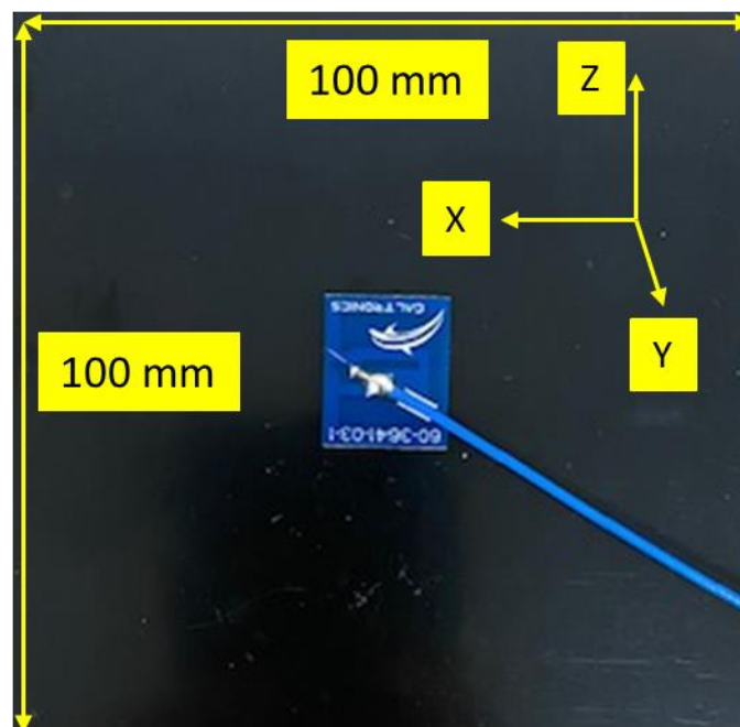
Figure 3 Measurement Orientation
