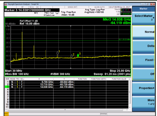
Channel 39 (2480MHz)
