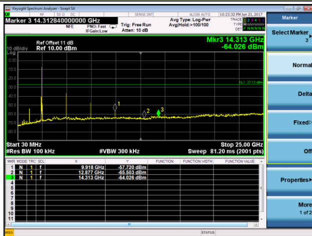
Spurious Emission 30MHz ~ 25GHz
