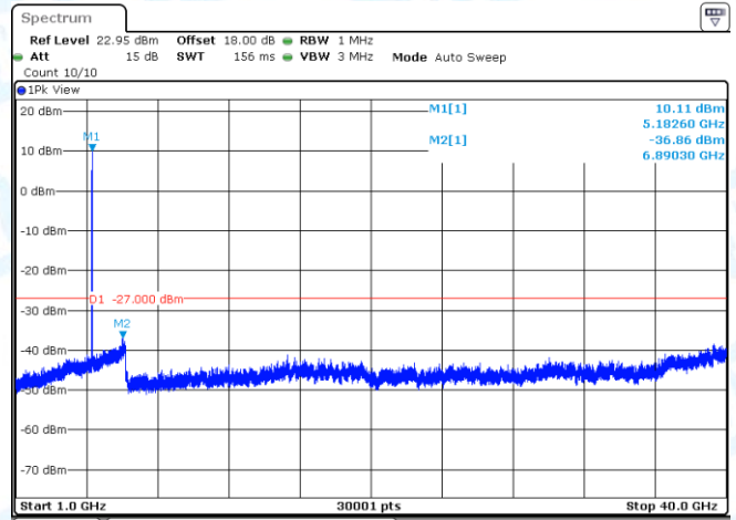
11AC20MIMO-Ant2-5180-1000~40000-PASS
