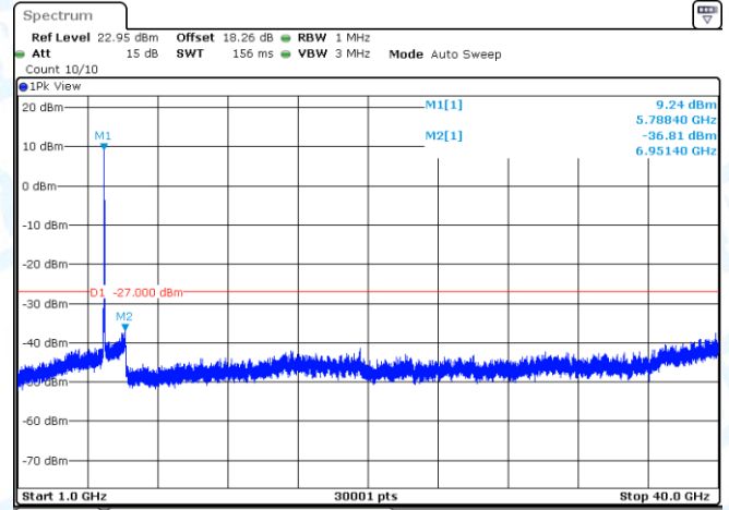
11AC40MIMO-Ant2-5795-1000~40000-PASS
