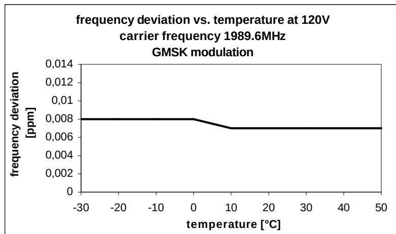
Fig. 74 – Frequency deviation vs. temperature (120V, 1989.6 MHz, GMSK modulation)
