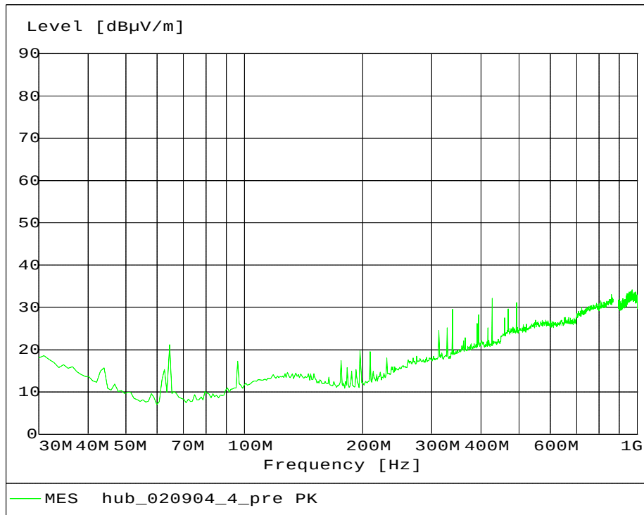
Fig. 64 – Radiated Emission 30 MHz – 1 GHz, 8PSK modulation.
