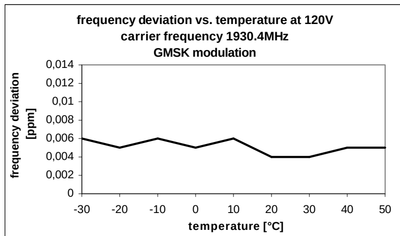
Fig. 68 – Frequency deviation vs. temperature (120V, 1930.4 MHz, GMSK modulation)
