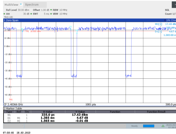
11ax20SISO_Ant1_2412_52Tone_RU37
