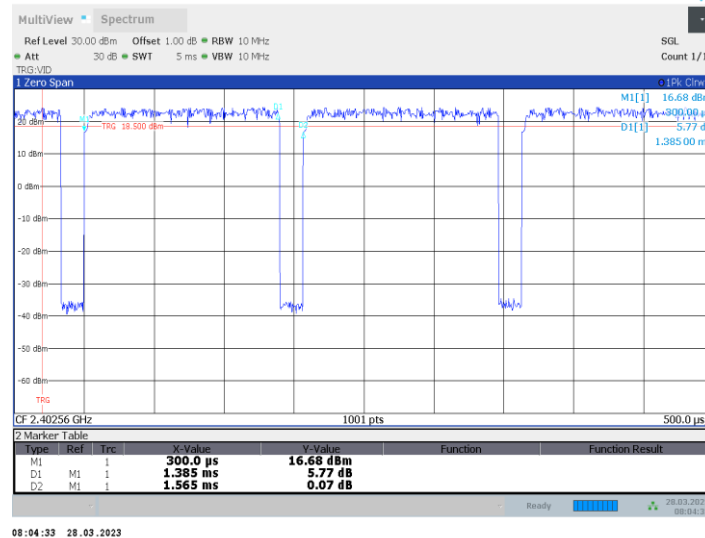
11ax20SISO_Ant1_2412_52Tone_RU37
