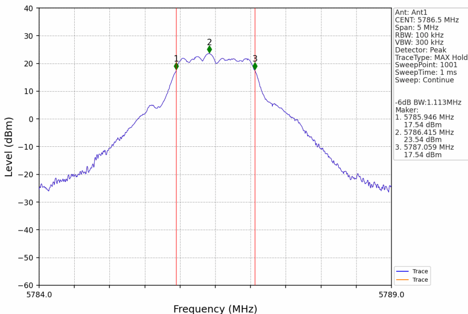
1.4M_MCH_5786.5MHz_Ant1_NTNV
