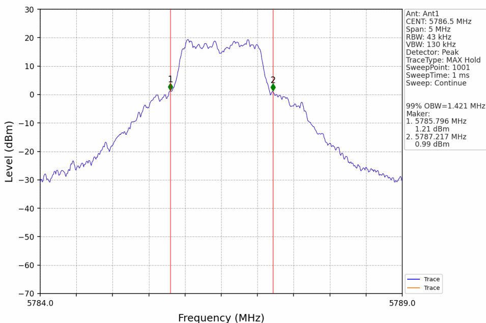
1.4M_MCH_5786.5MHz_Ant1_NTNV
