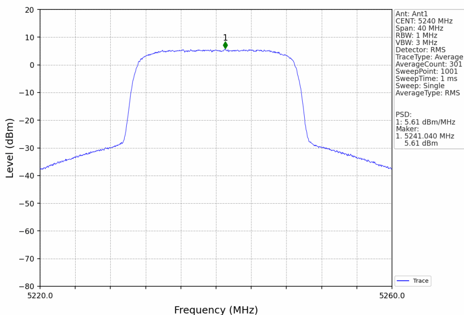
20M_HCH_5240MHz_Ant1_NTNV
