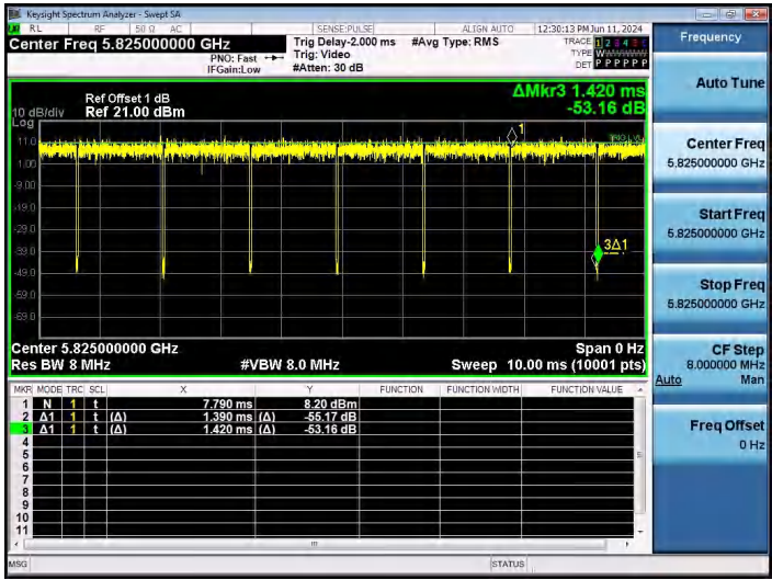
NTNV-11A-Ant1-5825
