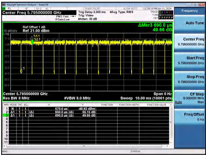
NTVN-11N40SISO-Ant1-5795
