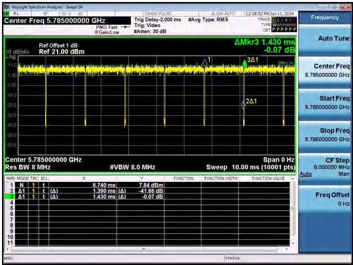
NTNV-11A-Ant1-5785
