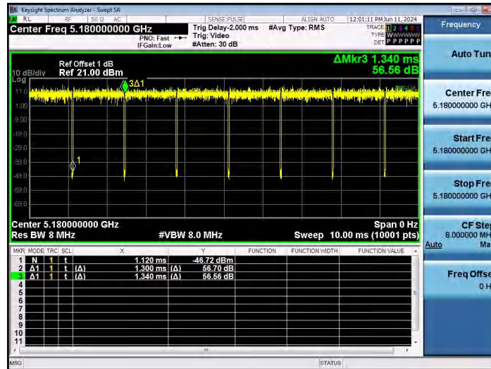
NTVN-11N20SISO-Ant1-5180
