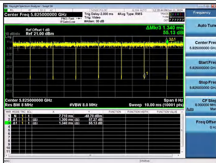
NTVN-11N20SISO-Ant1-5825
