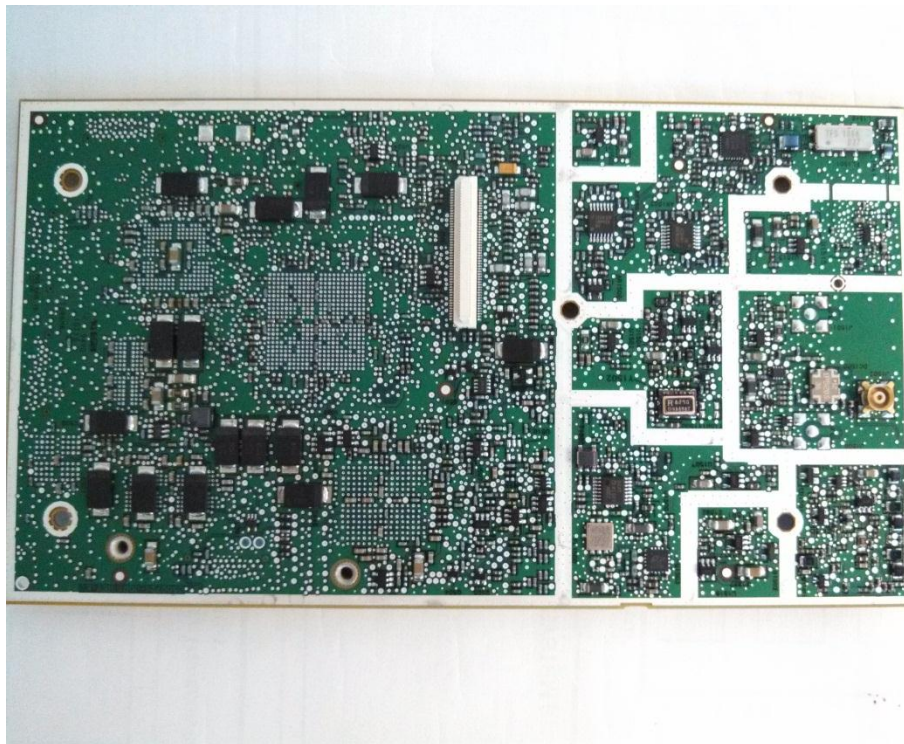
Core Module – Under side
