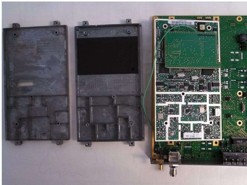
Both Shields Removed From Core Module. WLAN card shown attached.
