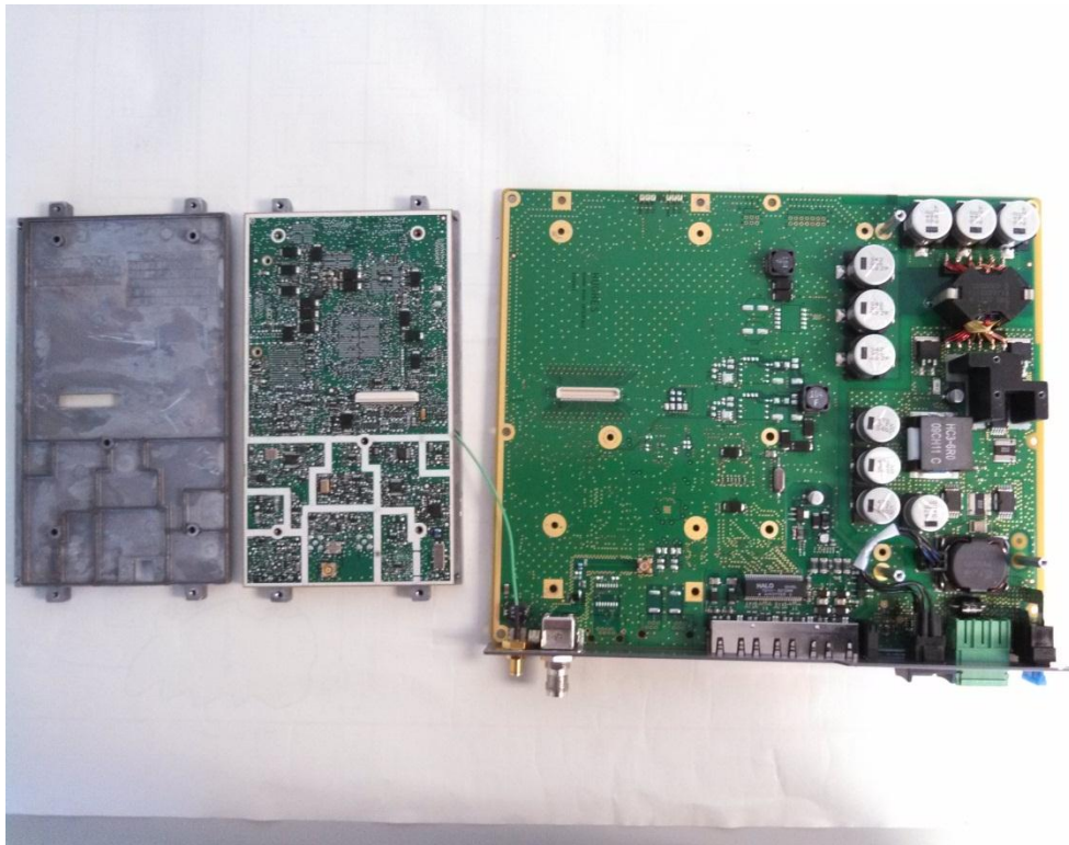
Bottom Shield Removed From Core Module
