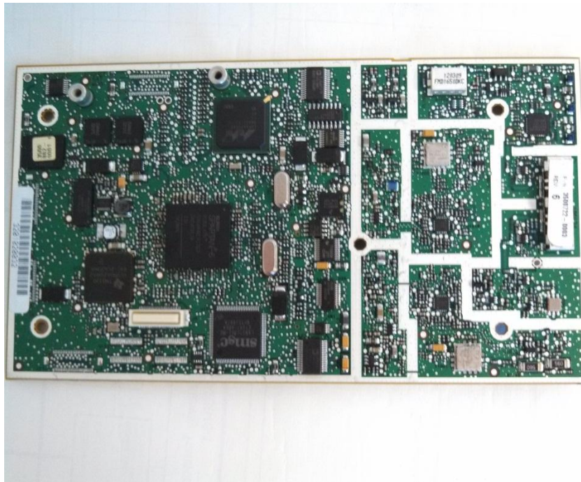
Core Module – Top side without WLAN card
