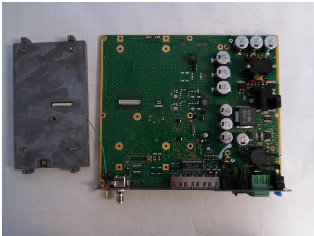
9105 Interface board with Core Module separated– Top side
