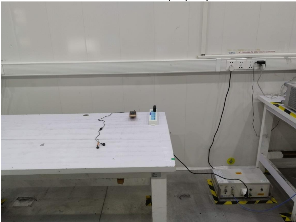
Conducted Emission(Adapter 2)
