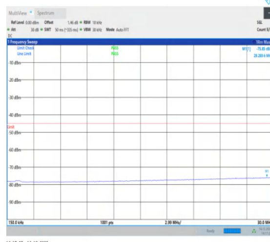
1-N41-30-100-M-1-DFT-PI2BPSK-Inner_1RB_Left-1 @ 1-0.15-30-Ant1-29.28--75.85--45-PASS
