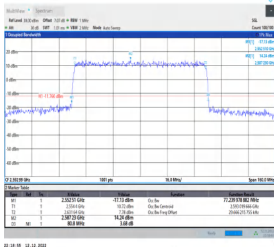
1-N41-30-80-M-6-CP-QPSK-Outer_Full-217@0-Ant 1-77.24-80.800-≤80-PASS
