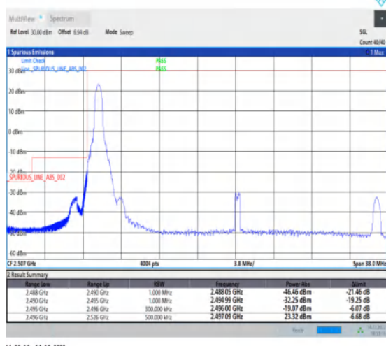
1-N41-30-30-L-4-CP-QPSK-Edge_1RB_Left-1@0-Ant1-1--PASS-see graph
