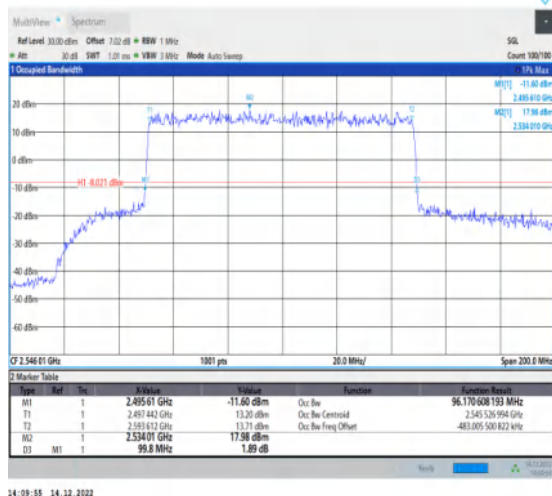
1-N41-30-100-L-1-DFT-QPSK-Outer_Full-270@0-An t1-96.171-99.800-≤100-PASS
