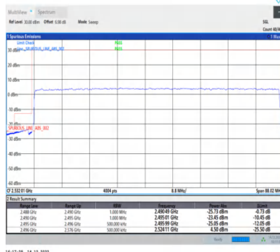
1-N41-30-80-L-3-DFT-PI2BPSK-Outer_Full-216@0-Ant1-1--PASS-see graph
