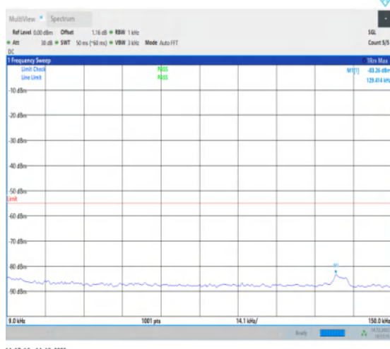
1-N41-30-100-M-1-DFT-PI2BPSK-Inner_1RB_Left-1 @ 1-0.009-0.15-Ant1-0.13--83.26--55-PASS
