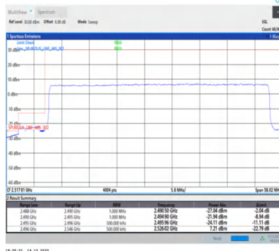
1-N41-30-50-L-3-DFT-PI2BPSK-Outer_Full-128@0-Ant1-1--PASS-see graph
