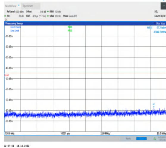
1-N41-30-100-H-1-DFT-QPSK-Edge_1RB_Left-1@0- 0.15-30-Ant1-27.67--77.78--45-PASS
