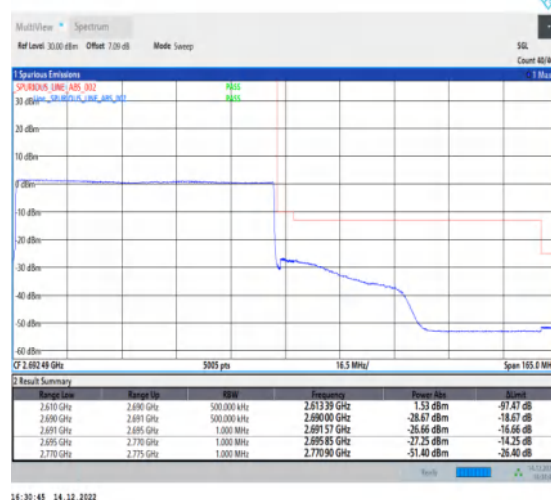
1-N41-30-80-H-6-CP-QPSK-Outer_Full-217@0-Ant1-1--PASS-see graph
