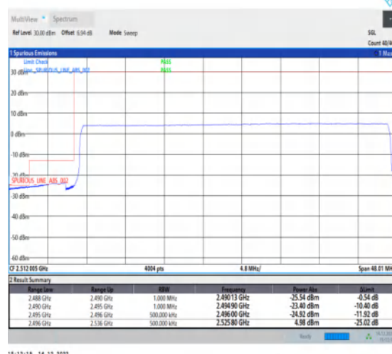
1-N41-30-40-L-6-CP-QPSK-Outer_Full-106@0-Ant1-1--PASS-see graph
