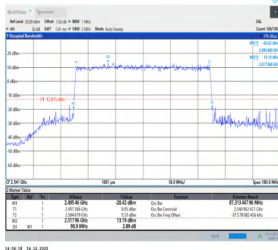
1-N41-30-90-L-9-CP-256QAM-Outer_Full-245@0-Ant t1-87.313-90.900≤90-PASS
