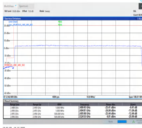
1-N41-30-100-L-3-DFT-PI2BPSK-Outer_Full-270@0-Ant1-1--PASS-see graph
