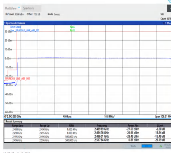
1-N41-30-100-L-6-CP-QPSK-Outer_Full-273@0-Ant1-1--PASS-see graph
