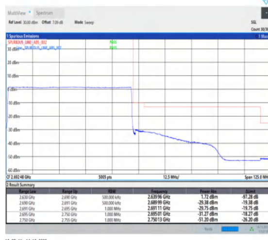
1-N41-30-60-H-6-CP-QPSK-Outer_Full-162@0-Ant1-1--PASS-see graph
