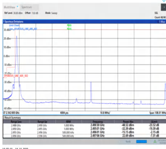
1-N41-30-100-L-1-DFT-PI2BPSK-Edge_1RB_Left-1@0-Ant1-1--PASS-see graph
