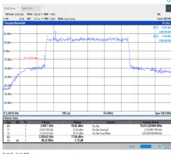
1-N41-30-80-L-1-DFT-QPSK-Outer_Full-216@0-Ant 1-76.913-80.320-≤80-PASS
