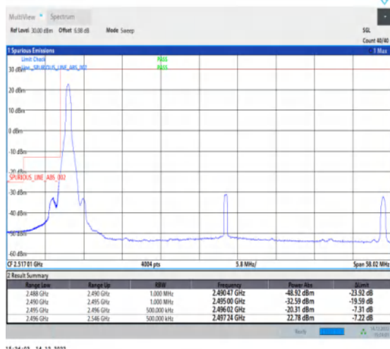
1-N41-30-50-L-1-DFT-PI2BPSK-Edge_1RB_Left-1@0-Ant1-1--PASS-see graph
