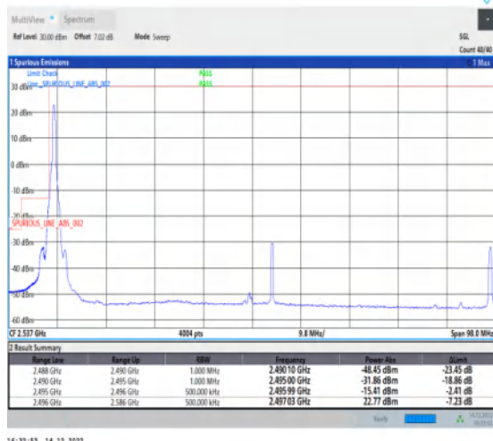
1-N41-30-90-L-1-DFT-PI2BPSK-Edge_1RB_Left-1@0-Ant1-1--PASS-see graph
