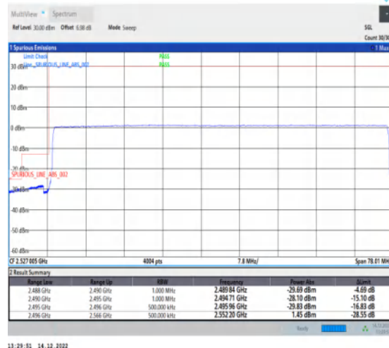
1-N41-30-70-L-6-CP-QPSK-Outer_Full-189@0-Ant1 -1--PASS-see graph
