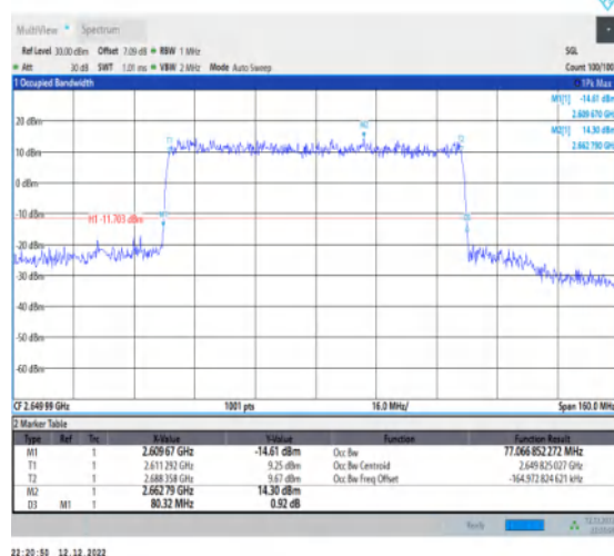
1-N41-30-80-H-4-DFT-64QAM-Outer_Full-216@0-Ant 1-77.067-80.320-≤80-PASS
