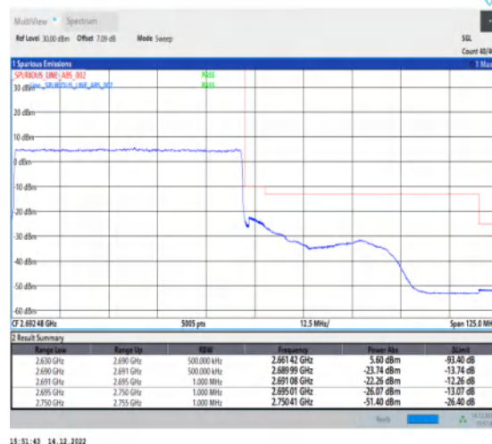
1-N41-30-60-H-3-DFT-PI2BPSK-Outer_Full-162@0-Ant1-1--PASS-see graph
