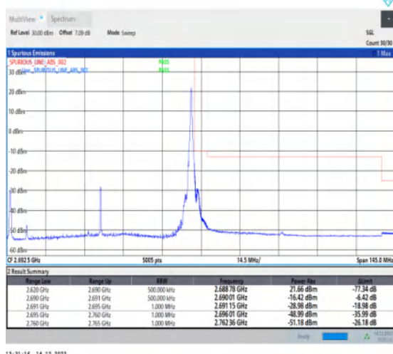
1-N41-30-70-H-5-CP-QPSK-Edge_1RB_Right-1@188-Ant1 -1--PASS-see graph
