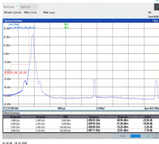
1-N41-30-40-L-1-DFT-PI2BPSK-Edge_1RB_Left-1@0-Ant1-1--PASS-see graph
