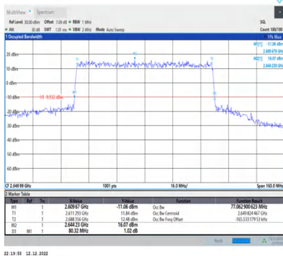
1-N41-30-80-H-1-DFT-QPSK-Outer_Full-216@0-Ant 1-77.063-80.320-≤80-PASS
