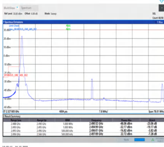
1-N41-30-70-L-4-CP-QPSK-Edge_1RB_Left-1@0-Ant1-1--PASS-see graph
