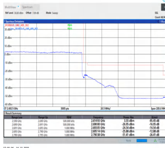
1-N41-30-100-H-3-DFT-PI2BPSK-Outer_Full-270 @0-Ant1-1--PASS-see graph
