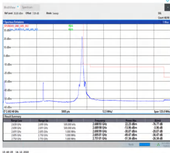
1-N41-30-60-H-2-DFT-PI2BPSK-Edge_1RB_Right-1@161-Ant1-1--PASS-see graph
