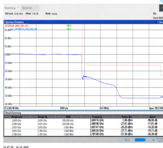
1-N41-30-90-H-6-CP-QPSK-Outer_Full-245@0-Ant1-1--PASS-see graph
