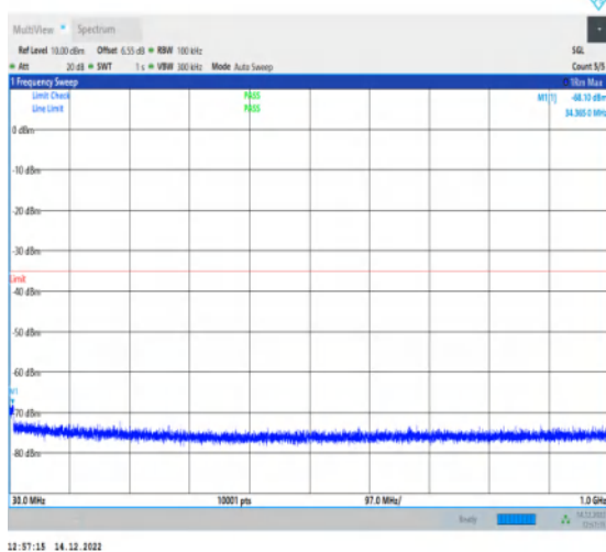
1-N41-30-100-H-1-DFT-QPSK-Edge_1RB_Left-1@ 0-30-1000-Ant1-34.37--68.10--35-PASS
