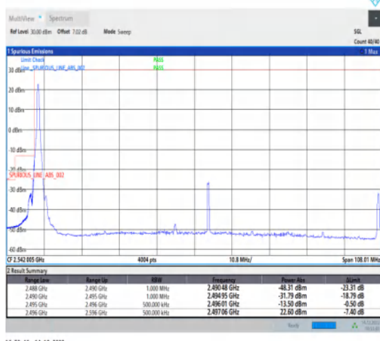
1-N41-30-100-L-4-CP-QPSK-Edge_1RB_Left-1@0-Ant1-1--PASS-see graph
