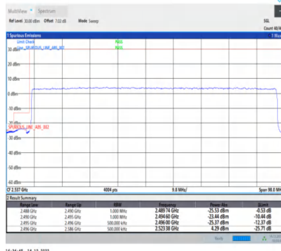
1-N41-30-90-L-3-DFT-PI2BPSK-Outer_Full-240@0-Ant1-1--PASS-see graph
