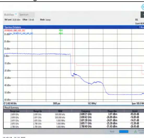
1-N41-30-90-H-3-DFT-PI2BPSK-Outer_Full-240@0-Ant1-1--PASS-see graph
