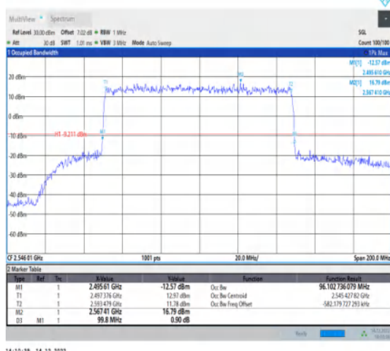
1-N41-30-100-L-3-DFT-16QAM-Outer_Full-270@0-A Ant1-96.103-99.800-≤100-PASS
