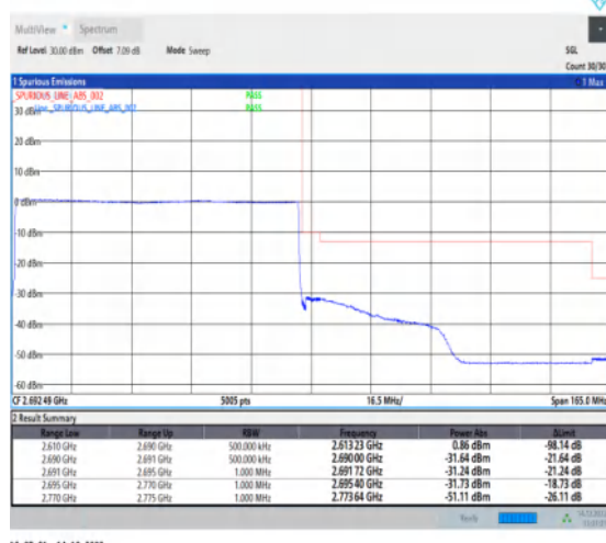
1-N41-30-80-H-6-CP-QPSK-Outer_Full-217@0-Ant1-1--PASS-see graph
