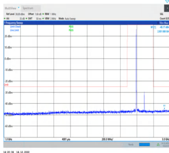
1-N41-30-100-H-1-DFT-PI2BPSK-Inner_1RB_Left-1 @1-1000-3000-Ant1-2931.00--45.17--25-PASS
