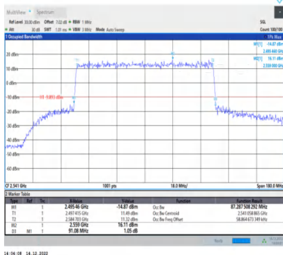
1-N41-30-90-L-8-CP-64QAM-Outer_Full-245@0-Ant 1-87.288-91.080≤90-PASS
