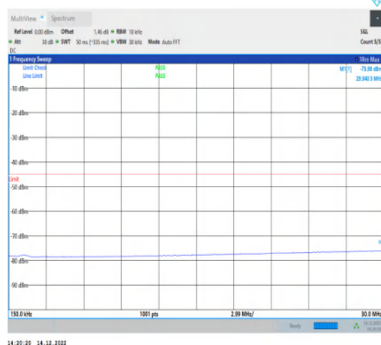
1-N41-30-100-H-1-DFT-PI2BPSK-Inner_1RB_Left-1 @1-0.15-30-Ant1-29.94--75.98--45-PASS
