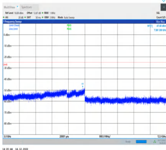
1-N41-30-100-H-1-DFT-PI2BPSK-Inner_1RB_Left-1 @ 1-3000-12000-Ant1-7381.20--47.60--25-PASS
