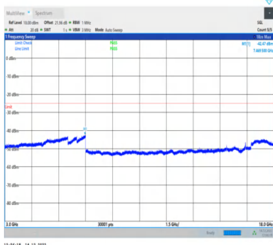
1-N41-30-100-M-1-DFT-QPSK-Edge_1RB_Left-1@ 0-3000-18000-Ant1-7469.50--42.47--25-PASS
