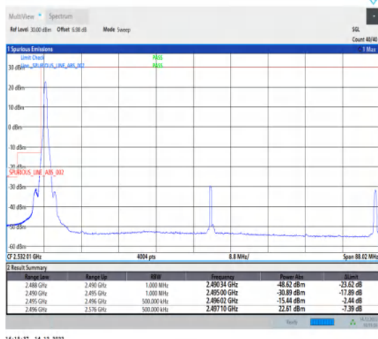
1-N41-30-80-L-1-DFT-PI2BPSK-Edge_1RB_Left-1@0-Ant1-1--PASS-see graph
