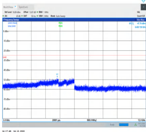
1-N41-30-100-M-1-DFT-PI2BPSK-Inner_1RB_Left-1 @1-3000-12000-Ant1-6432.15--47.76--25-PASS
