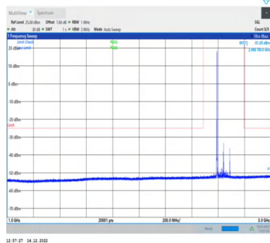
1-N41-30-100-H-1-DFT-QPSK-Edge_1RB_Left-1@0- 1000-3000-Ant1-2998.70--51.03--25-PASS
