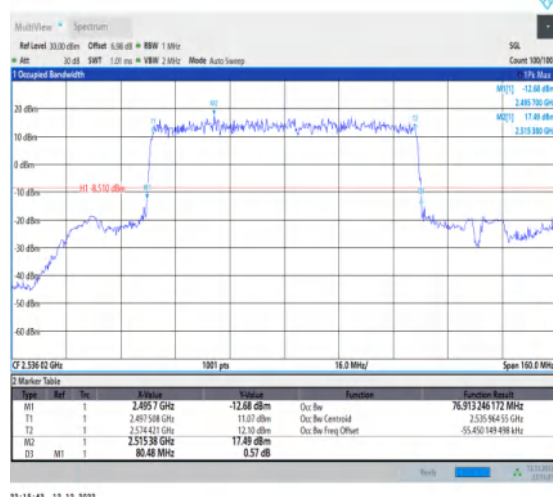
1-N41-30-80-L-2-DFT-PI2BPSK-Outer_Full-216@0-Ant 1-76.913-80.480-≤80-PASS
