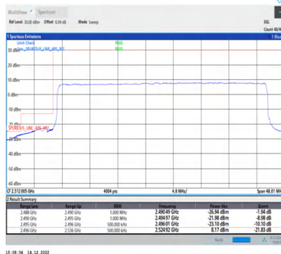
1-N41-30-40-L-3-DFT-PI2BPSK-Outer_Full-100@0-Ant1-1--PASS-see graph
