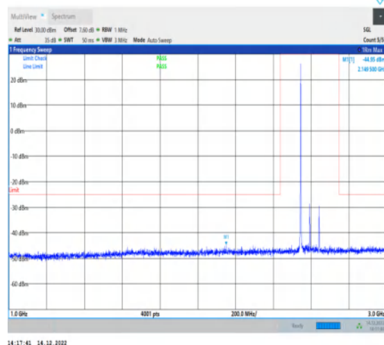
1-N41-30-100-M-1-DFT-PI2BPSK-Inner_1RB_Left-1 @1-1000-3000-Ant1-2149.50--44.95--25-PASS
