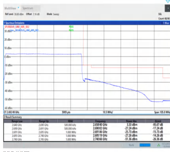
1-N41-30-50-H-6-CP-QPSK-Outer_Full-133@0-Ant1-1--PASS-see graph
