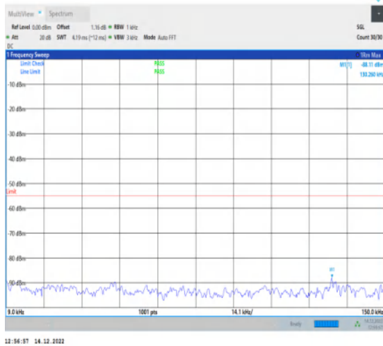
1-N41-30-100-H-1-DFT-QPSK-Edge_1RB_Left-1@ 0-0.009-0.15-Ant1-0.13--88.11--55-PASS
