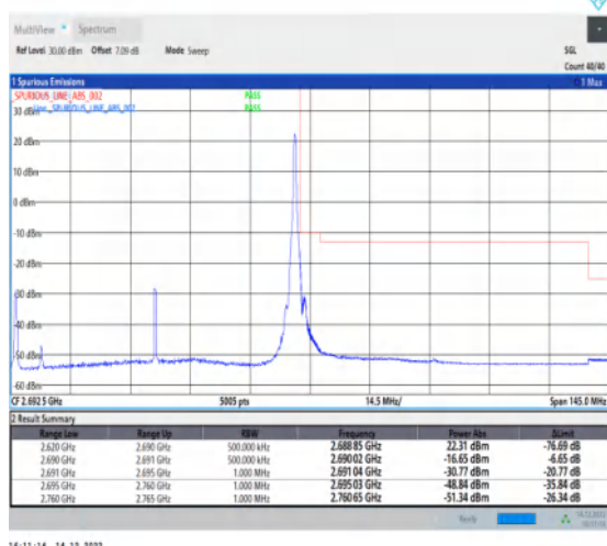
1-N41-30-70-H-5-CP-QPSK-Edge_1RB_Right-1@188-Ant1-1--PASS-see graph
