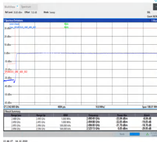
1-N41-30-100-L-6-CP-QPSK-Outer_Full-273@0-A nt1-1--PASS-see graph
