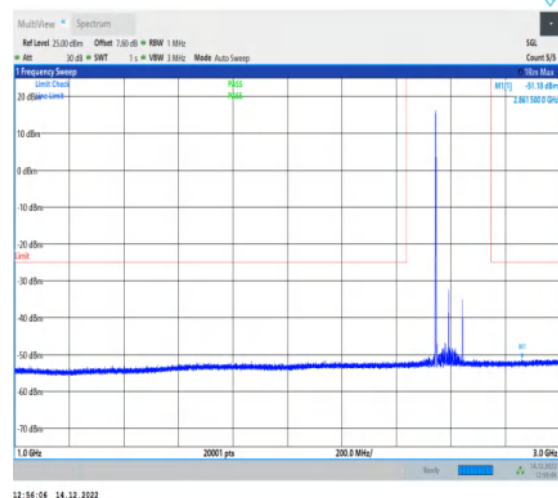
1-N41-30-100-M-1-DFT-QPSK-Edge_1RB_Left-1@0- 1000-3000-Ant1-2861.50--51.18--25-PASS
