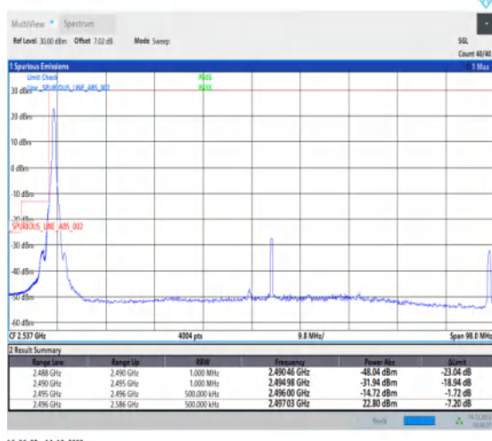
1-N41-30-90-L-4-CP-QPSK-Edge_1RB_Left-1@0-Ant1-1--PASS-see graph
