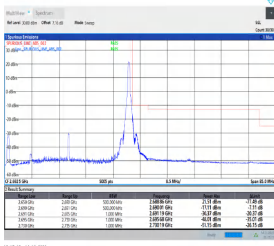
1-N41-30-40-H-5-CP-QPSK-Edge_1RB_Right-1@105-Ant1-1--PASS-see graph
