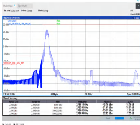
1-N41-30-20-L-4-CP-QPSK-Edge_1RB_Left-1@0-Ant1-1--PASS-see graph
