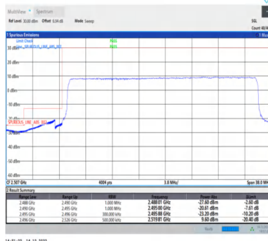
1-N41-30-30-L-3-DFT-PI2BPSK-Outer_Full-75@0-Ant1-1--PASS-see graph
