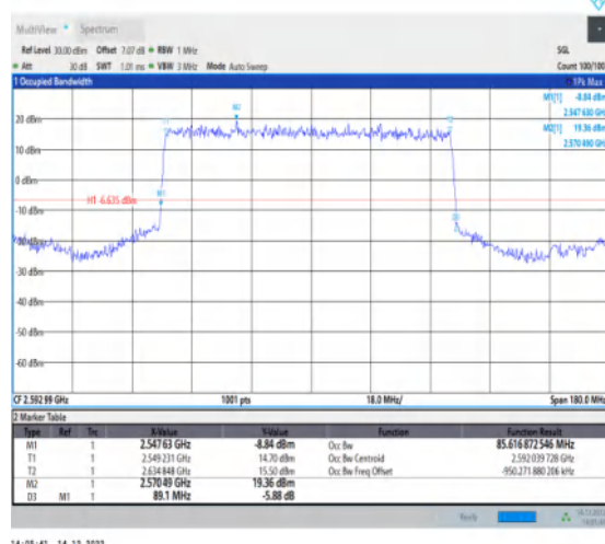
1-N41-30-90-M-2-DFT-PI2BPSK-Outer_Full-240@0-Ant Ant1-85.617-89.100≤90-PASS
