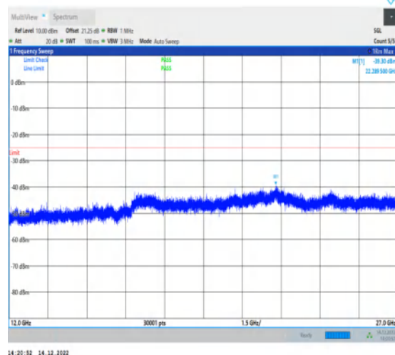
1-N41-30-100-H-1-DFT-PI2BPSK-Inner_1RB_Left-1 @ 1-12000-27000-Ant1-22289.50--39.30--25-PASS
