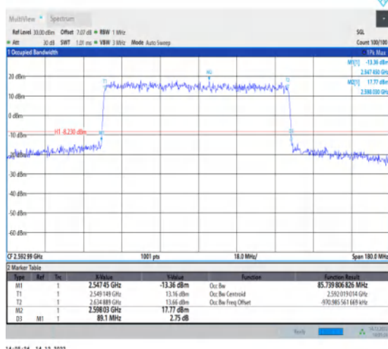
1-N41-30-90-M-1-DFT-QPSK-Outer_Full-240@0-Ant 1-85.74-89.100≤90-PASS
