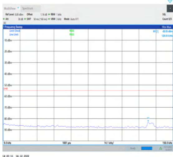
1-N41-30-100-H-1-DFT-PI2BPSK-Inner_1RB_Left-1 @1-0.009-0.15-Ant1-0.13--83.05--55-PASS
