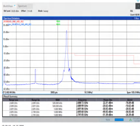
1-N41-30-50-H-2-DFT-PI2BPSK-Edge_1RB_Right-1@132-Ant1-1--PASS-see graph
