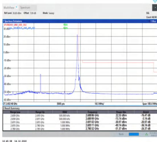
1-N41-30-90-H-5-CP-QPSK-Edge_1RB_Right-1@244-Ant1-1--PASS-see graph
