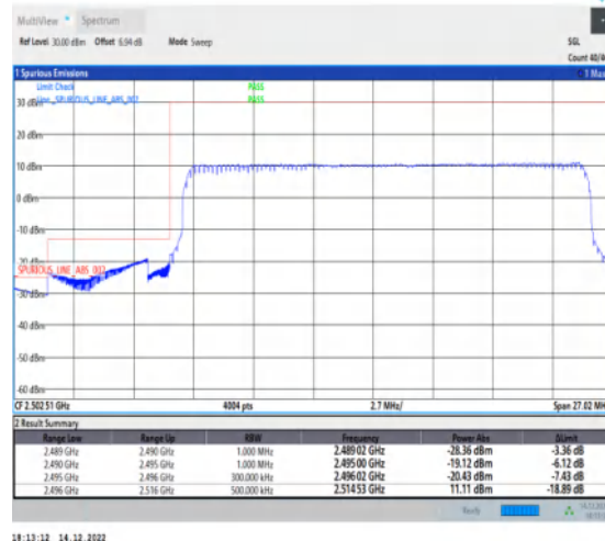
1-N41-30-20-L-3-DFT-PI2BPSK-Outer_Full-50@0-Ant1-1--PASS-see graph
