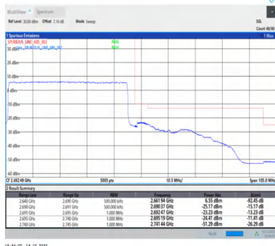
1-N41-30-50-H-3-DFT-PI2BPSK-Outer_Full-128@0-Ant1-1--PASS-see graph
