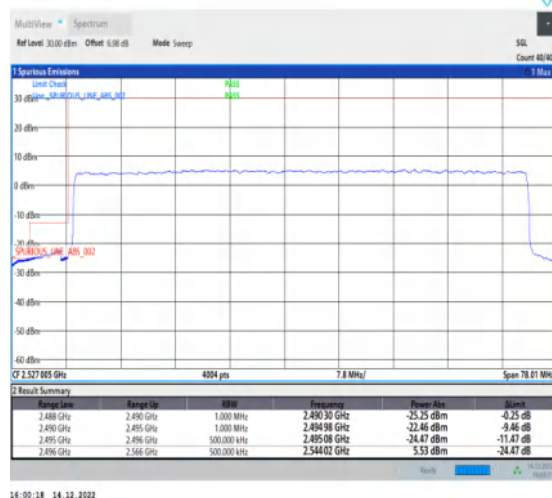
1-N41-30-70-L-3-DFT-PI2BPSK-Outer_Full-180@0-Ant1-1--PASS-see graph
