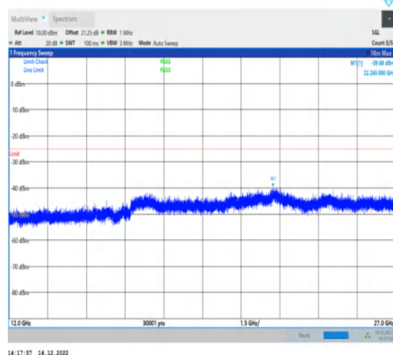
1-N41-30-100-M-1-DFT-PI2BPSK-Inner_1RB_Left-1 @1-12000-27000-Ant1-22245.00--39.68--25-PASS
