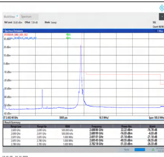
1-N41-30-90-H-2-DFT-PI2BPSK-Edge_1RB_Right-1@244-Ant1-1--PASS-see graph
