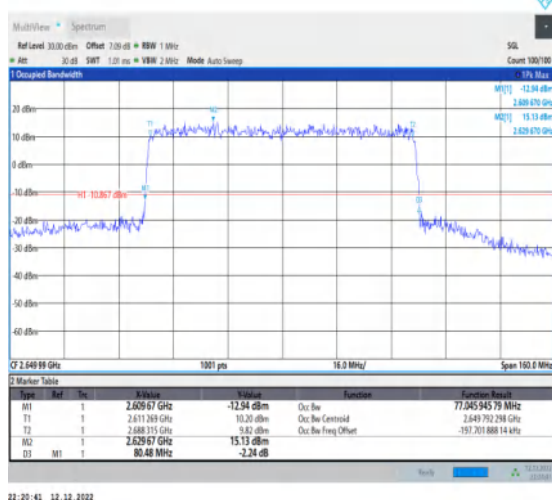
1-N41-30-80-H-3-DFT-16QAM-Outer_Full-216@0-Ant 1-77.046-80.480-≤80-PASS
