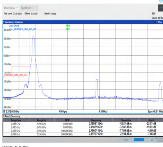
1-N41-30-40-L-4-CP-QPSK-Edge_1RB_Left-1@0-Ant1-1--PASS-see graph
