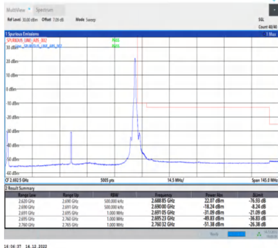
1-N41-30-70-H-2-DFT-PI2BPSK-Edge_1RB_Right-1@188-Ant1-1--PASS-see graph
