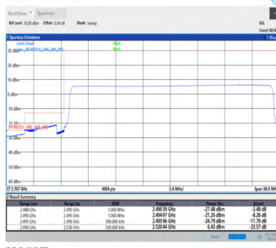
1-N41-30-30-L-6-CP-QPSK-Outer_Full-78@0-Ant1-1--PASS-see graph
