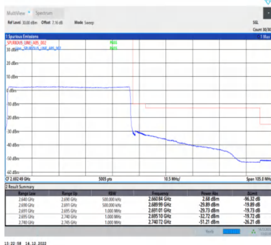
1-N41-30-50-H-6-CP-QPSK-Outer_Full-133@0-Ant1 -1--PASS-see graph
