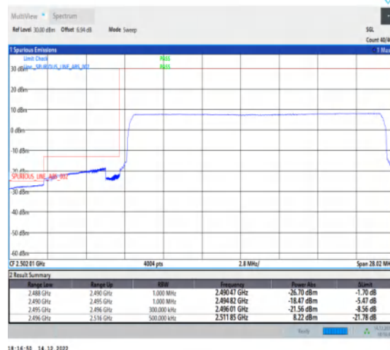
1-N41-30-20-L-6-CP-QPSK-Outer_Full-51@0-Ant1-1--PASS-see graph
