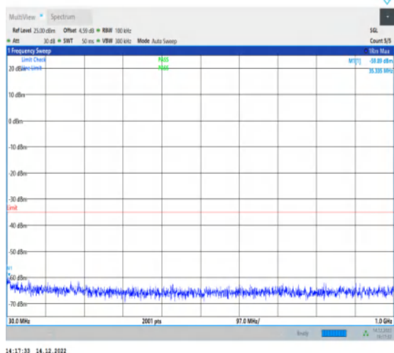
1-N41-30-100-M-1-DFT-PI2BPSK-Inner_1RB_Left-1 @1-30-1000-Ant1-35.34--59.89--35-PASS
