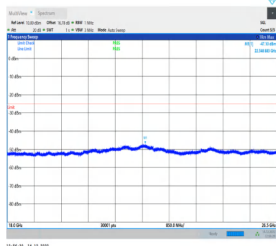
1-N41-30-100-M-1-DFT-QPSK-Edge_1RB_Left-1@0- 18000-26500-Ant1-22348.88--47.10--25-PASS
