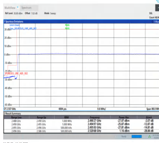
1-N41-30-90-L-6-CP-QPSK-Outer_Full-245@0-Ant1-1--PASS-see graph
