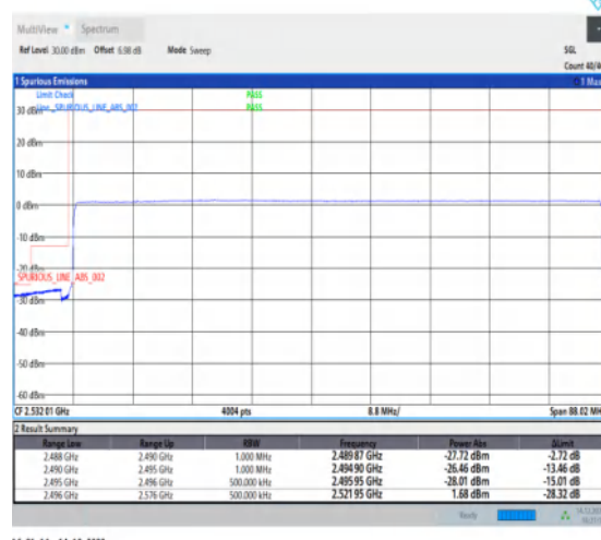
1-N41-30-80-L-6-CP-QPSK-Outer_Full-217@0-Ant1-1--PASS-see graph
