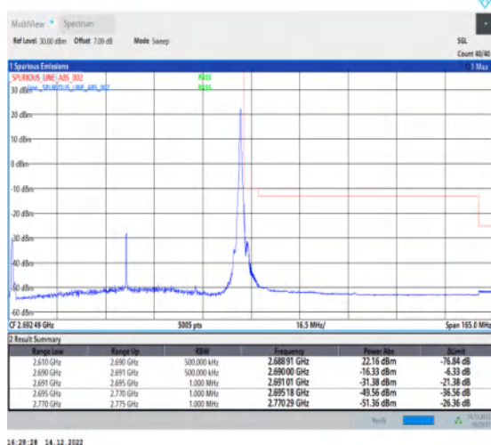
1-N41-30-80-H-5-CP-QPSK-Edge_1RB_Right-1@216-Ant1-1--PASS-see graph
