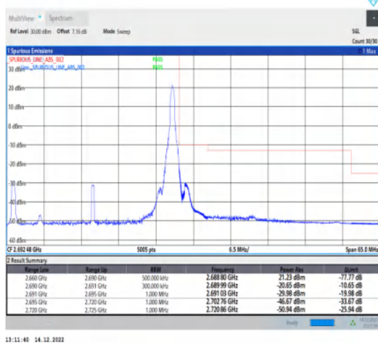
1-N41-30-30-H-5-CP-QPSK-Edge_1RB_Right-1@77-Ant1 1-1--PASS-see graph
