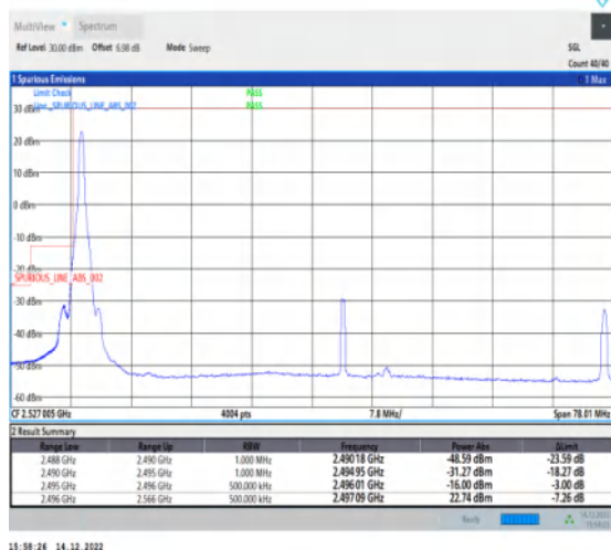
1-N41-30-70-L-1-DFT-PI2BPSK-Edge_1RB_Left-1@0-Ant1-1--PASS-see graph
