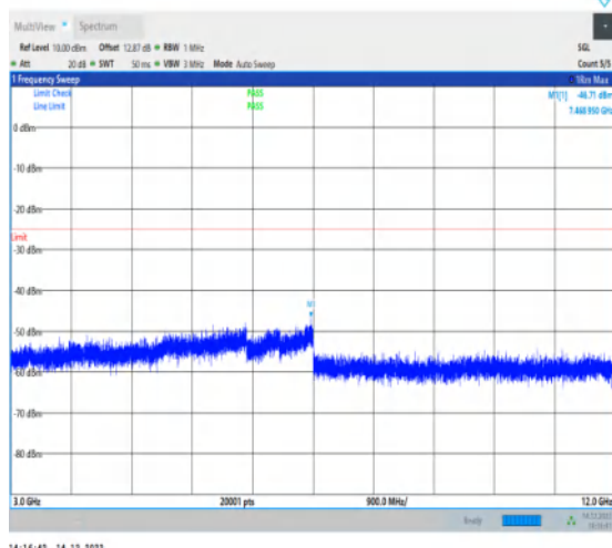
1-N41-30-100-L-1-DFT-PI2BPSK-Inner_1RB_Left-1 @ 1-3000-12000-Ant1-7468.95--46.71--25-PASS
