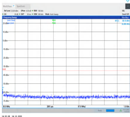
1-N41-30-100-H-1-DFT-PI2BPSK-Inner_1RB_Left-1 @1-30-1000-Ant1-33.40--58.10--35-PASS
