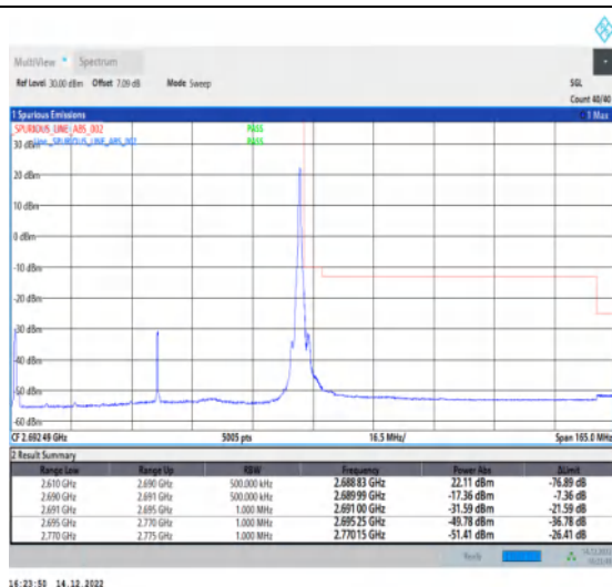
1-N41-30-80-H-2-DFT-PI2BPSK-Edge_1RB_Right-1@216-Ant1-1--PASS-see graph
