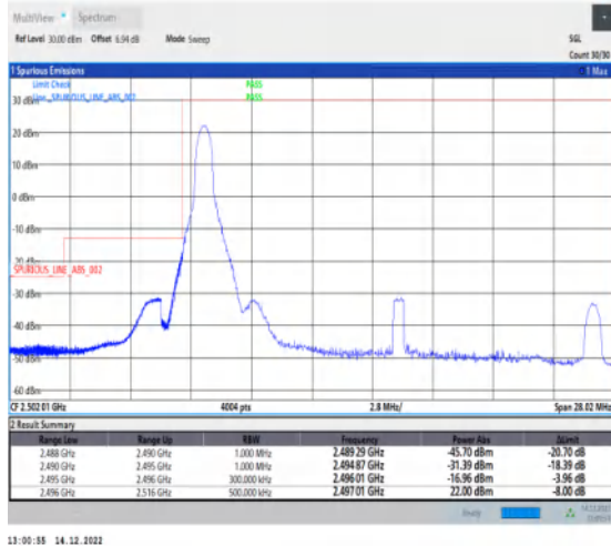
1-N41-30-20-L-4-CP-QPSK-Edge_1RB_Left-1@0-Ant1 1-1--PASS-see graph
