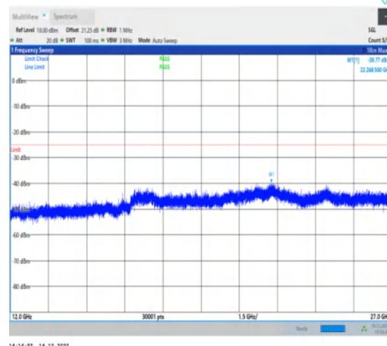
1-N41-30-100-L-1-DFT-PI2BPSK-Inner_1RB_Left-1 @ 1-12000-27000-Ant1-22268.50--39.77--25-PASS
