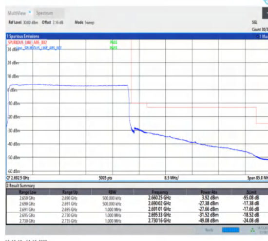
1-N41-30-40-H-6-CP-QPSK-Outer_Full-106@0-Ant1-1--PASS-see graph
