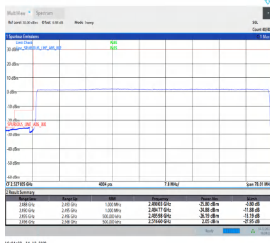
1-N41-30-70-L-6-CP-QPSK-Outer_Full-189@0-Ant1-1--PASS-see graph
