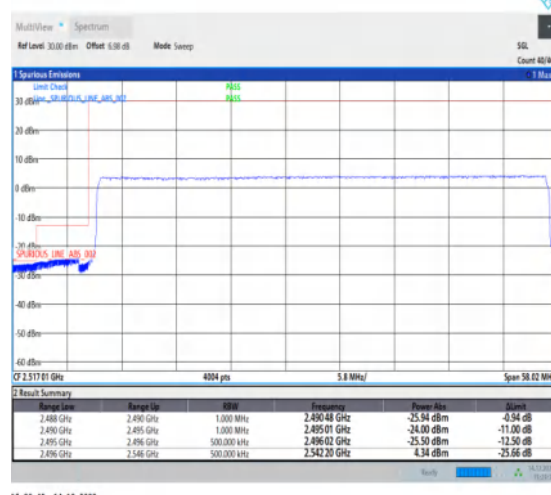
1-N41-30-50-L-6-CP-QPSK-Outer_Full-133@0-Ant1-1--PASS-see graph
