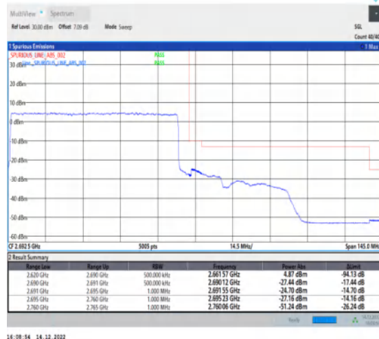
1-N41-30-70-H-3-DFT-PI2BPSK-Outer_Full-180@0-Ant1-1--PASS-see graph
