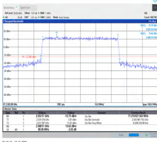
1-N41-30-80-M-8-CP-64QAM-Outer_Full-217@0-Ant t1-77.211-80.960-≤80-PASS
