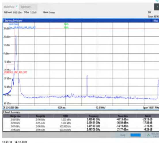
1-N41-30-100-L-4-CP-QPSK-Edge_1RB_Left-1@0-Ant 1-1--PASS-see graph
