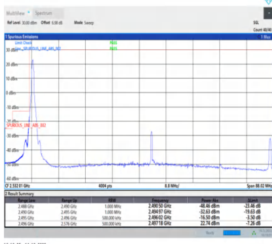
1-N41-30-80-L-4-CP-QPSK-Edge_1RB_Left-1@0-Ant1-1--PASS-see graph
