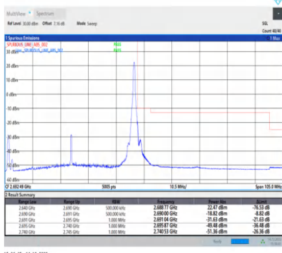
1-N41-30-50-H-5-CP-QPSK-Edge_1RB_Right-1@132-Ant1-1--PASS-see graph
