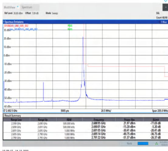
1-N41-30-100-H-2-DFT-PI2BPSK-Edge_1RB_Right-1 @272-Ant1-1--PASS-see graph
