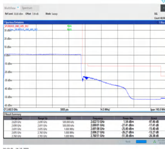
1-N41-30-70-H-6-CP-QPSK-Outer_Full-189@0-Ant1-1--PASS-see graph
