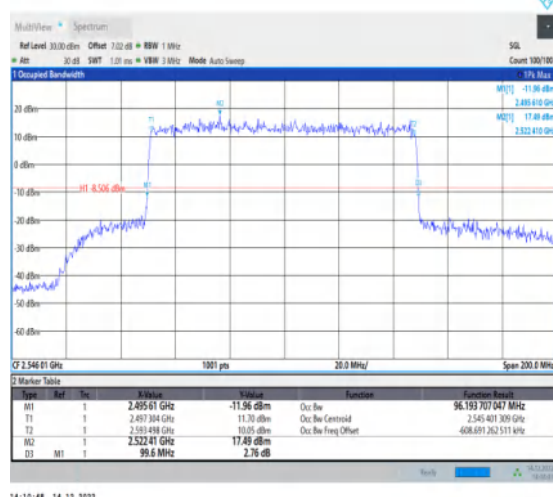
1-N41-30-100-L-4-DFT-64QAM-Outer_Full-270@0-A Ant1-96.194-99.600-≤100-PASS
