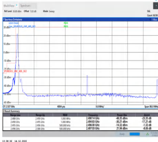
1-N41-30-90-L-4-CP-QPSK-Edge_1RB_Left-1@0-Ant1 -1--PASS-see graph
