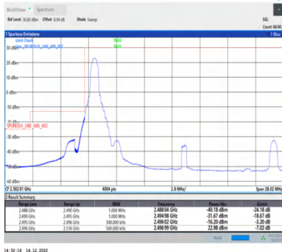
1-N41-30-20-L-1-DFT-PI2BPSK-Edge_1RB_Left-1@0-Ant1-1--PASS-see graph
