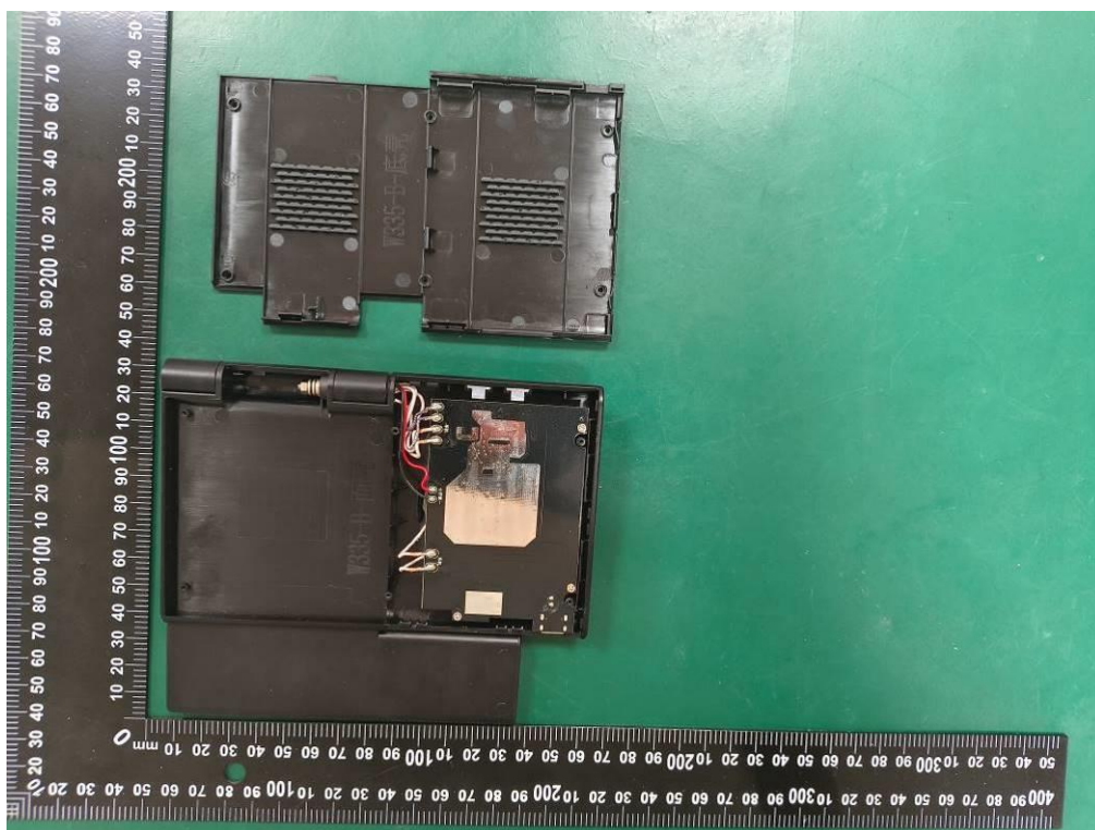
Internal Photo FCC ID: 2BBEH-W335B
