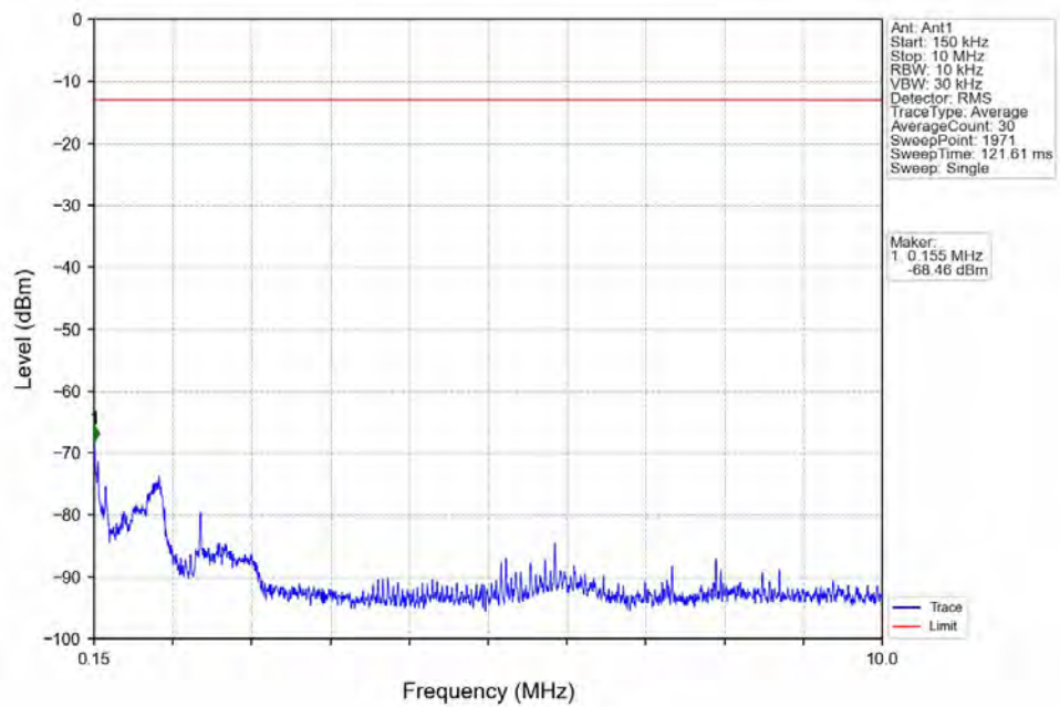
Band4_5MHz_16QAM_LCH_1712.5MHz_RB_1_0_NTNV
