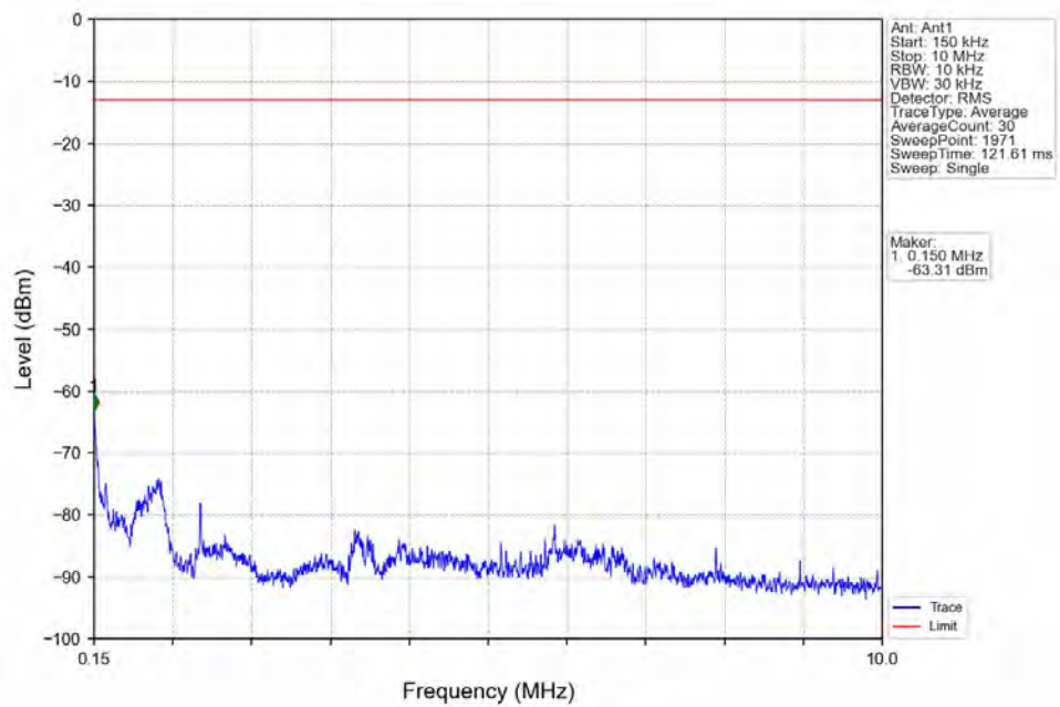
Band4_3MHz_16QAM_MCH_1732.5MHz_RB_1_0_NTNV
