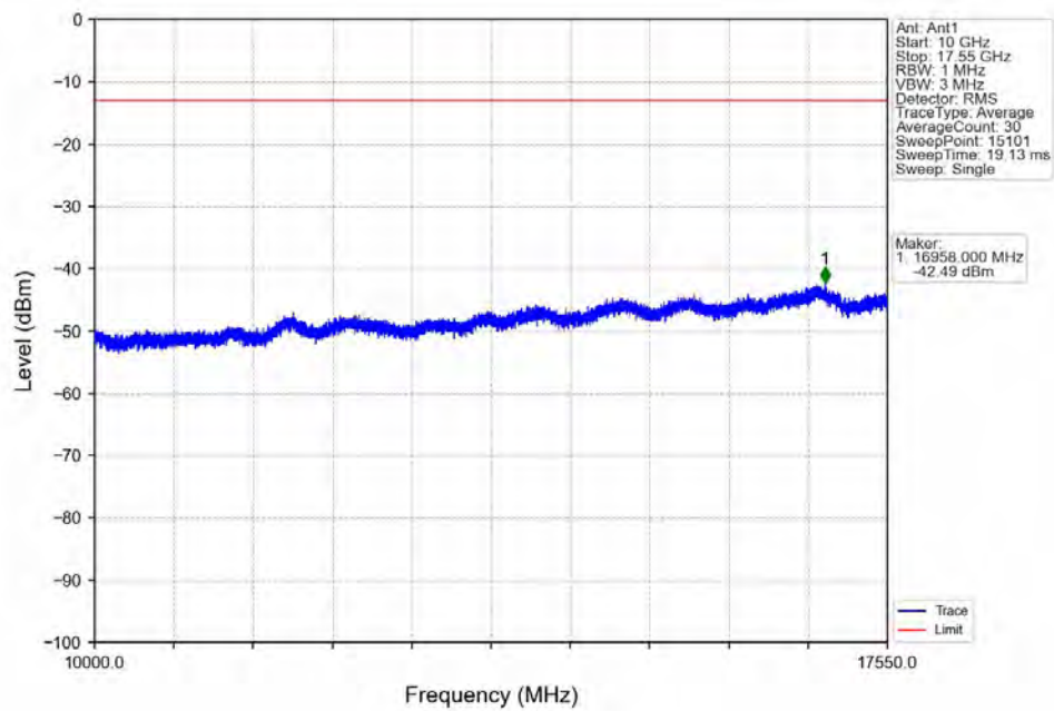
Band4_1.4MHz_QPSK_LCH_1710.7MHz_RB_1_0_NTNV
