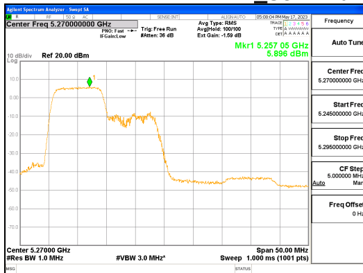
ANT R_802.11ax_HE40_106T_Low_UNII 2A
