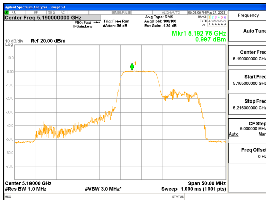
ANT L_802.11ax_HE40_106T_Mid_UNII 1
