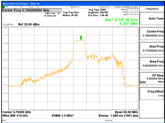
ANT R_802.11ax_HE40_52T_Mid_UNII 3
