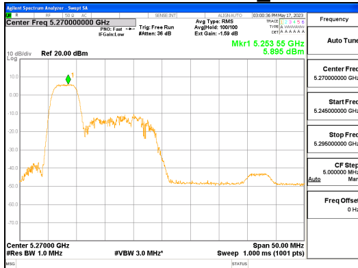
ANT R_802.11ax_HE40_52T_Low_UNII 2A
