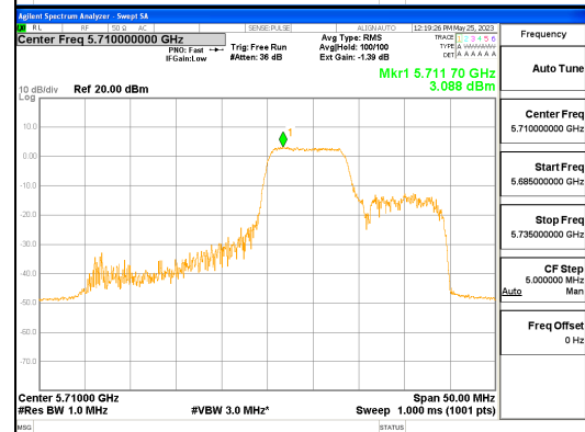
ANT L_802.11ax_HE40_106T_Mid_UNII 2C
