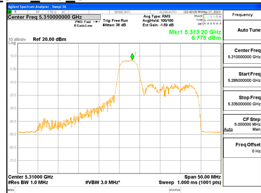
ANT R_802.11ax_HE40_52T_Mid_UNII 2A
