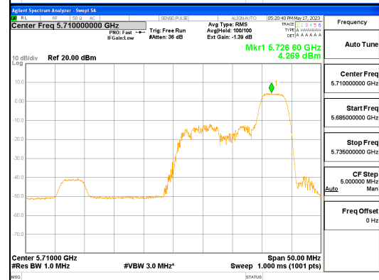
ANT L_802.11ax_HE40_52T_High_UNII 2C
