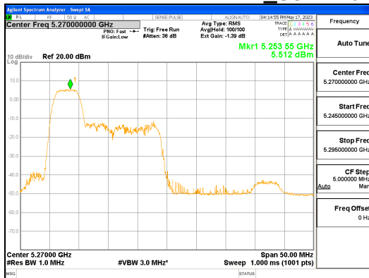
ANT L_802.11ax_HE40_52T_Low_UNII 2A
