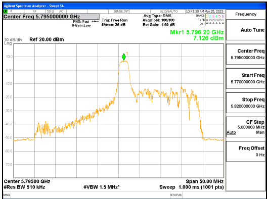
ANT R_802.11ax_HE40_26T_Mid_UNII 3
