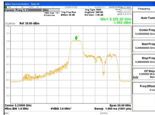
ANT L_802.11ax_HE40_52T_Mid_UNII 1
