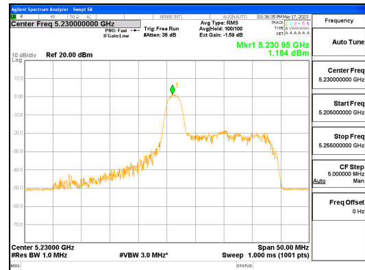
ANT R_802.11ax_HE40_26T_Mid_UNII 1
