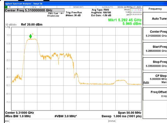
ANT R_802.11ax_HE40_52T_Low_UNII 2A
