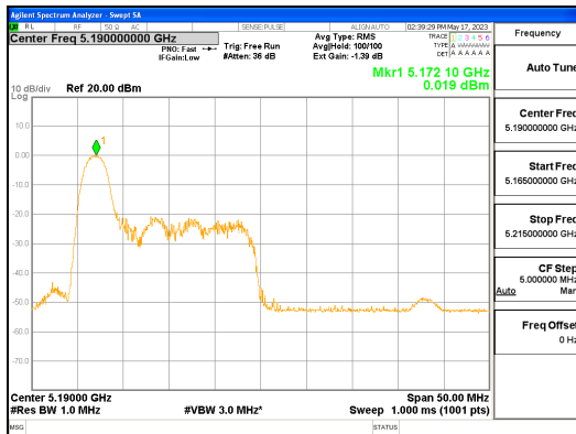
ANT L_802.11ax_HE40_26T_Low_UNII 1
