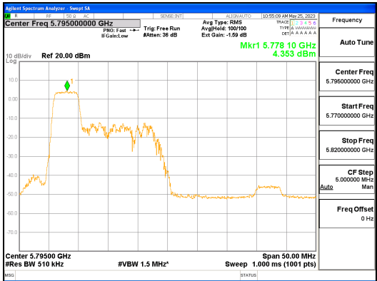
ANT R_802.11ax_HE40_52T_Low_UNII 3
