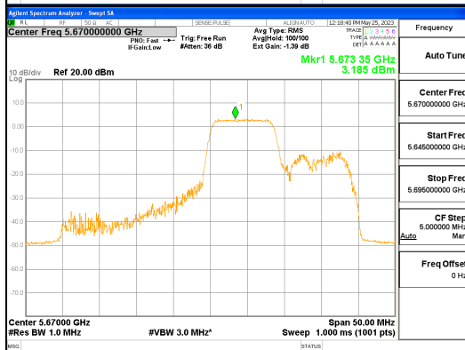
ANT L_802.11ax_HE40_106T_Mid_UNII 2C
