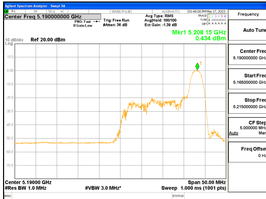
ANT L_802.11ax_HE40_26T_High_UNII 1
