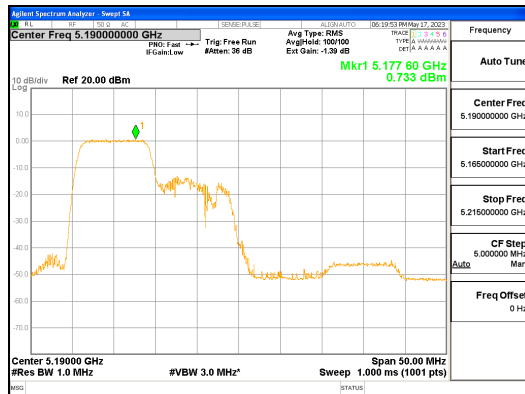
ANT L_802.11ax_HE40_106T_Low_UNII 1
