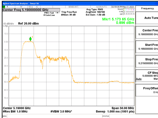
ANT R_802.11ax_HE40_52T_Low_UNII 1
