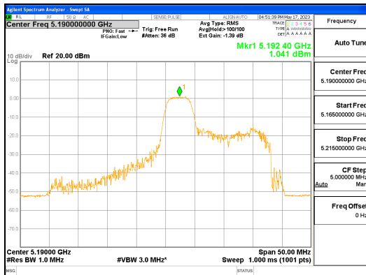
ANT L_802.11ax_HE40_52T_Mid_UNII 1
