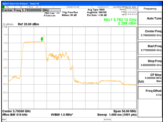
ANT L_802.11ax_HE40_106T_Low_UNII 3
