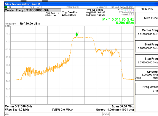
ANT L_802.11ax_HE40_106T_Mid_UNII 2A
