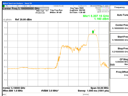
ANT L_802.11ax_HE40_52T_High_UNII 1
