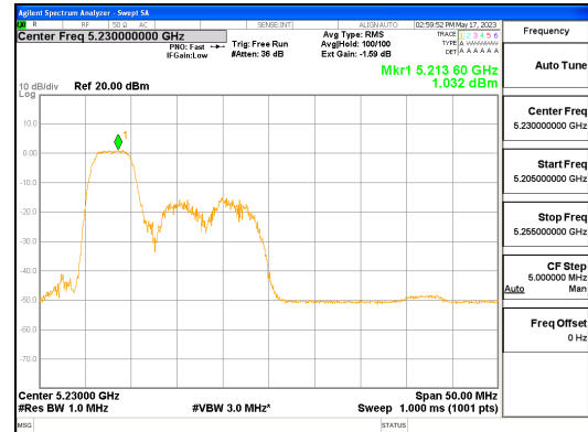
ANT R_802.11ax_HE40_52T_Low_UNII 1
