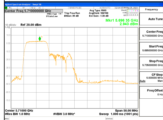
ANT L_802.11ax_HE40_106T_Low_UNII 2C
