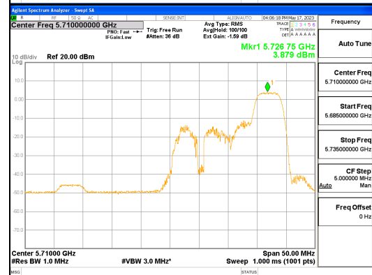
ANT R_802.11ax_HE40_52T_High_UNII 2C
