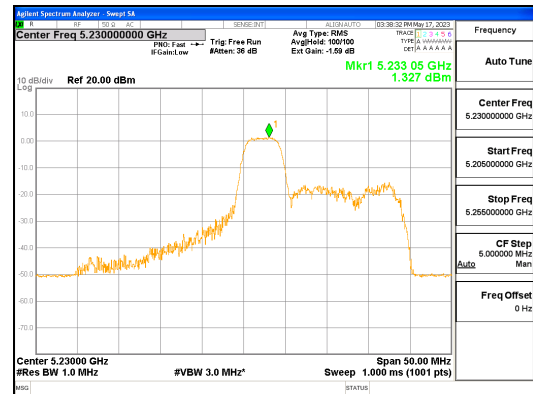
ANT R_802.11ax_HE40_52T_Mid_UNII 1
