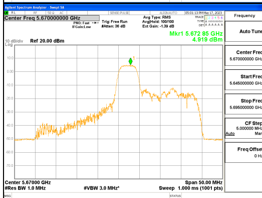
ANT L_802.11ax_HE40_52T_Mid_UNII 2C
