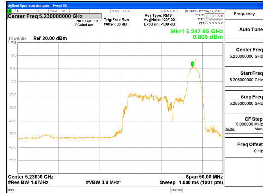
ANT L_802.11ax_HE40_26T_High_UNII 1
