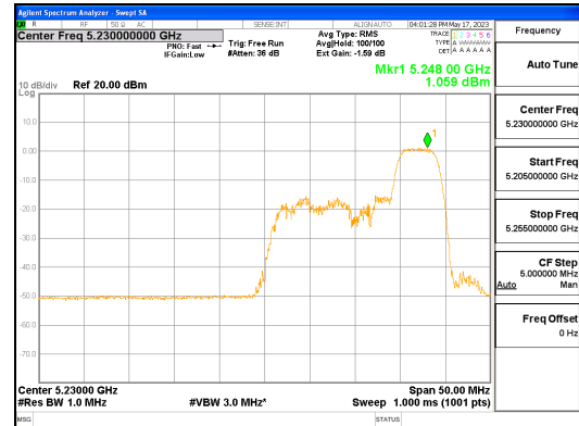
ANT R_802.11ax_HE40_52T_High_UNII 1
