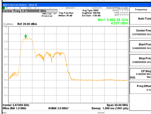
ANT R_802.11ax_HE40_52T_Low_UNII 2C
