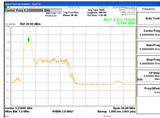
ANT L_802.11ax_HE40_26T_Low_UNII 1
