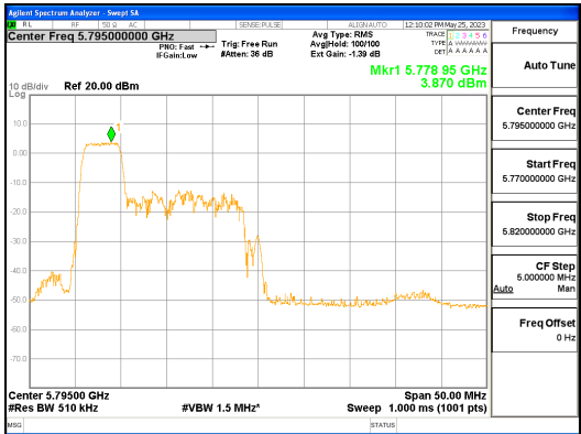
ANT L_802.11ax_HE40_52T_Low_UNII 3
