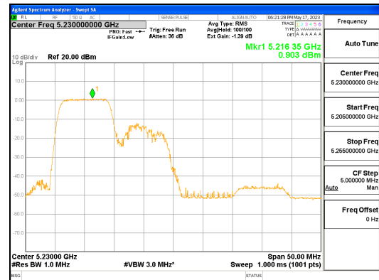
ANT L_802.11ax_HE40_106T_Low_UNII 1
