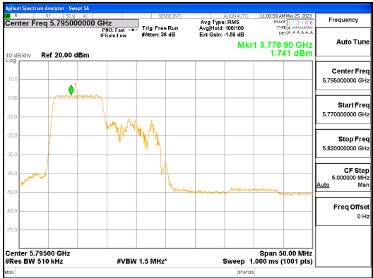
ANT R_802.11ax_HE40_106T_Low_UNII 3
