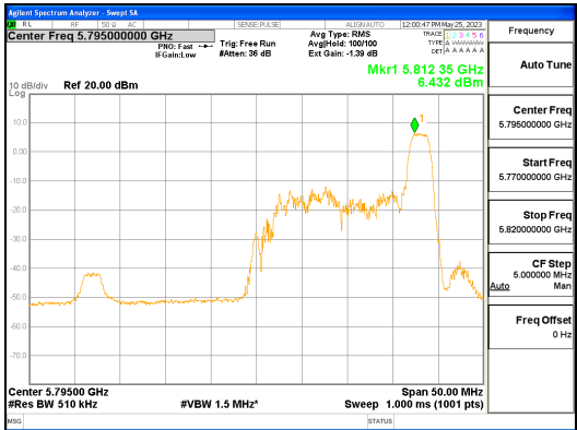
ANT L_802.11ax_HE40_26T_High_UNII 3
