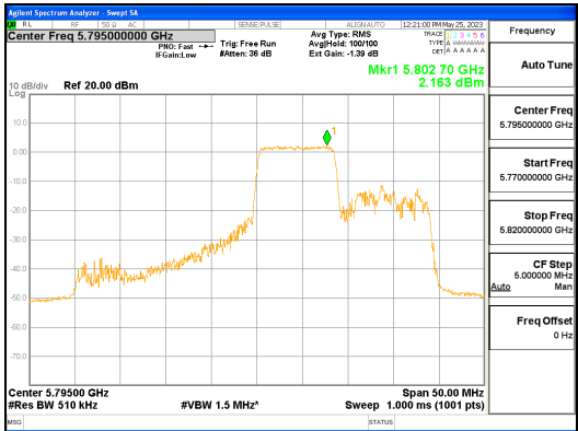
ANT L_802.11ax_HE40_106T_Mid_UNII 3
