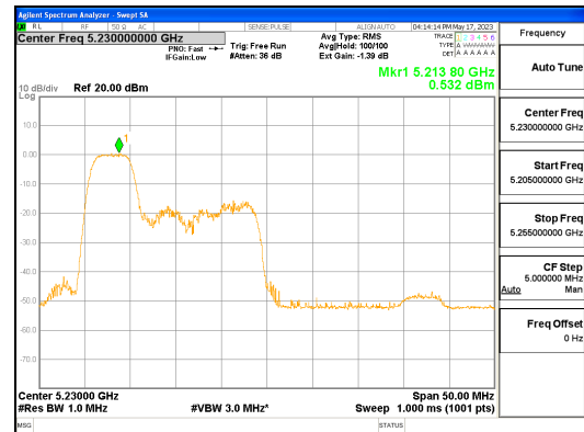
ANT L_802.11ax_HE40_52T_Low_UNII 1
