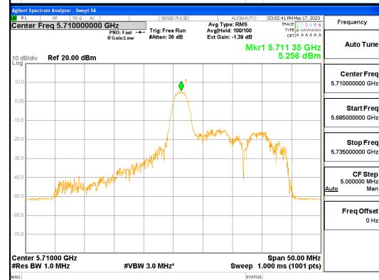
ANT L_802.11ax_HE40_26T_Mid_UNII 2C
