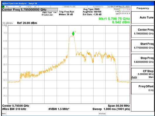
ANT L_802.11ax_HE40_26T_Mid_UNII 3
