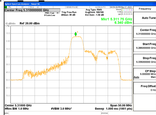
ANT L_802.11ax_HE40_52T_Mid_UNII 2A
