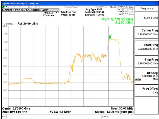
ANT L_802.11ax_HE40_52T_High_UNII 3
