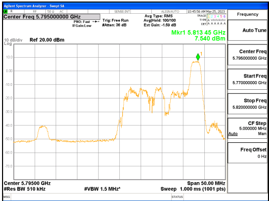
ANT R_802.11ax_HE40_26T_High_UNII 3
