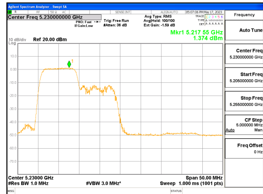
ANT R_802.11ax_HE40_106T_Low_UNII 1
