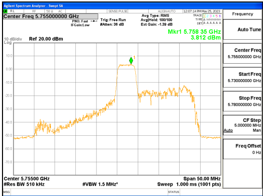
ANT L_802.11ax_HE40_52T_Mid_UNII 3
