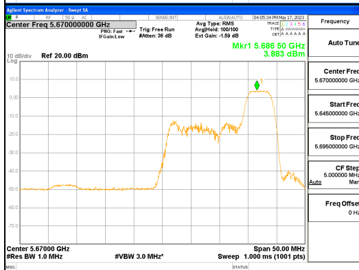
ANT R_802.11ax_HE40_52T_High_UNII 2C
