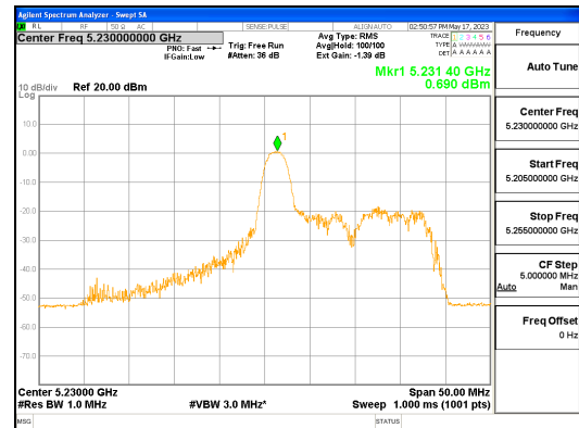
ANT L_802.11ax_HE40_26T_Mid_UNII 1
