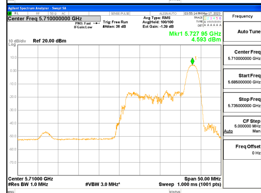
ANT L_802.11ax_HE40_26T_High_UNII 2C
