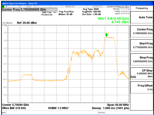
ANT R_802.11ax_HE40_52T_High_UNII 3
