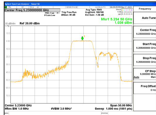
ANT L_802.11ax_HE40_106T_Mid_UNII 1
