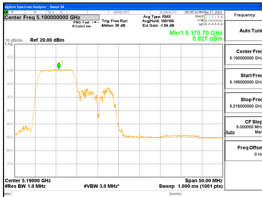
ANT R_802.11ax_HE40_106T_Low_UNII 1
