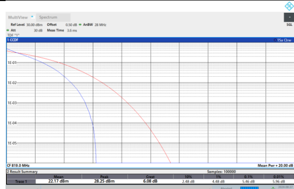
Band26-10MHz-16QAM-26740-50RB#0
