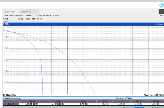
Band26-3MHz-16QAM-26705-1RB#0
