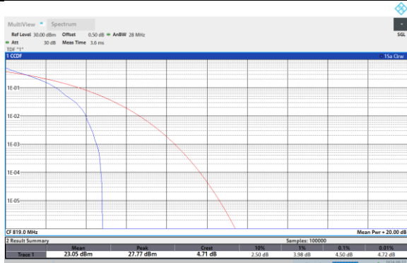
Band26-10MHz-16QAM-26740-1RB#0
